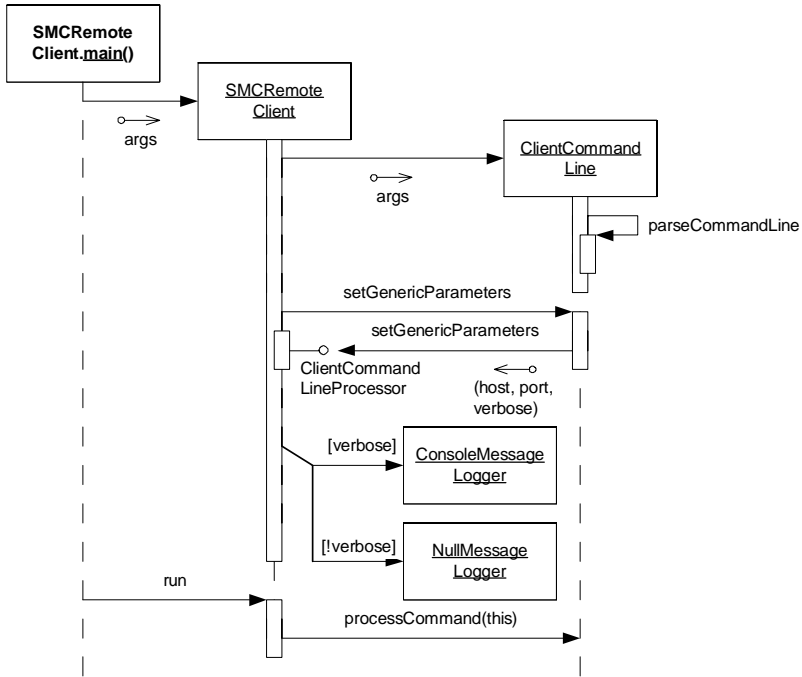
Figure 12-5 SMCRemoteClient.main()
