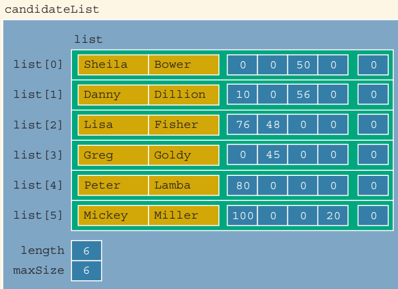
FIGURE 18-47 candidateList after copying temp
