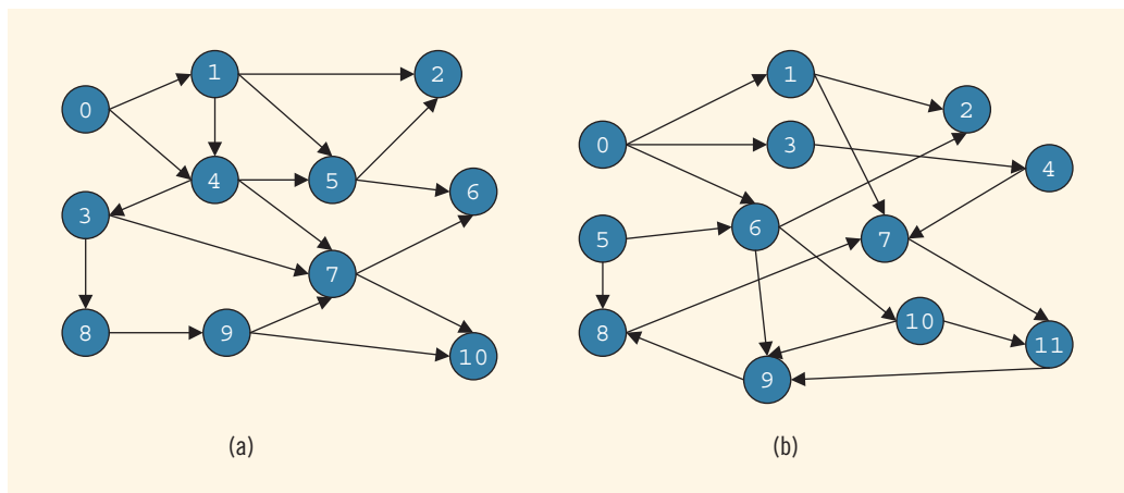
FIGURE 20-17 Graphs for Exercises 2 to 10
