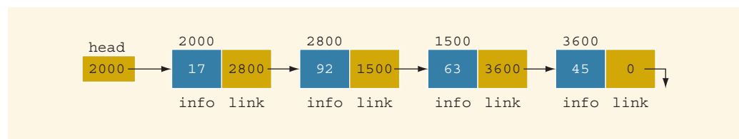
FIGURE 16-4 Linked list with four nodes
