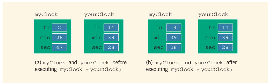
FIGURE 10-3 myClock and yourClock before and after executing the statement myClock = yourClock;
