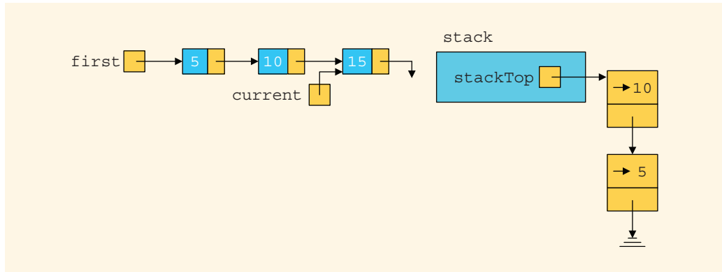
FIGURE 17-21 List and stack after the statements stack.push(current); and current = current->link; execute
