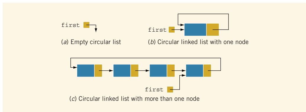
FIGURE 16-45 Circular linked lists
