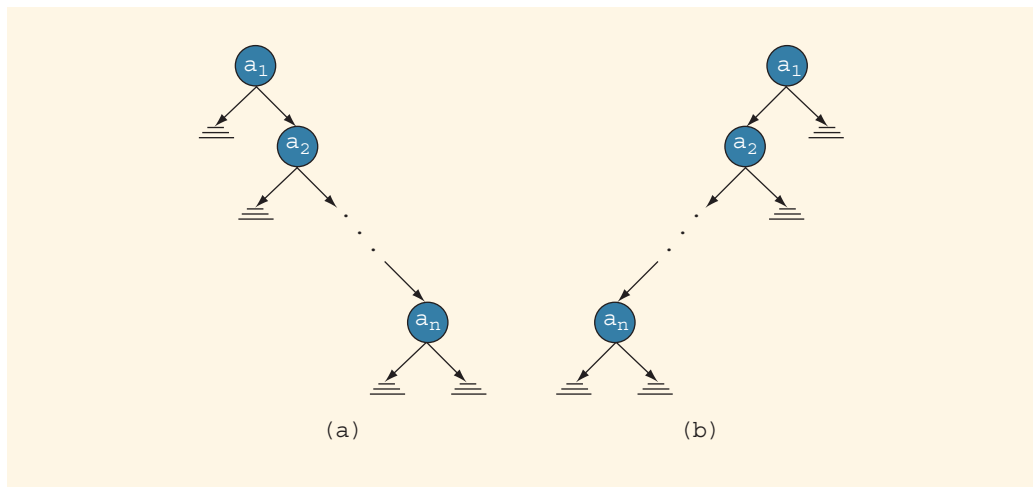
FIGURE 19-11 Linear binary search trees
