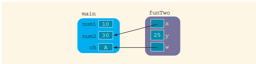
FIGURE 6-12 Values of the variables before the statement in Line 14 executes
