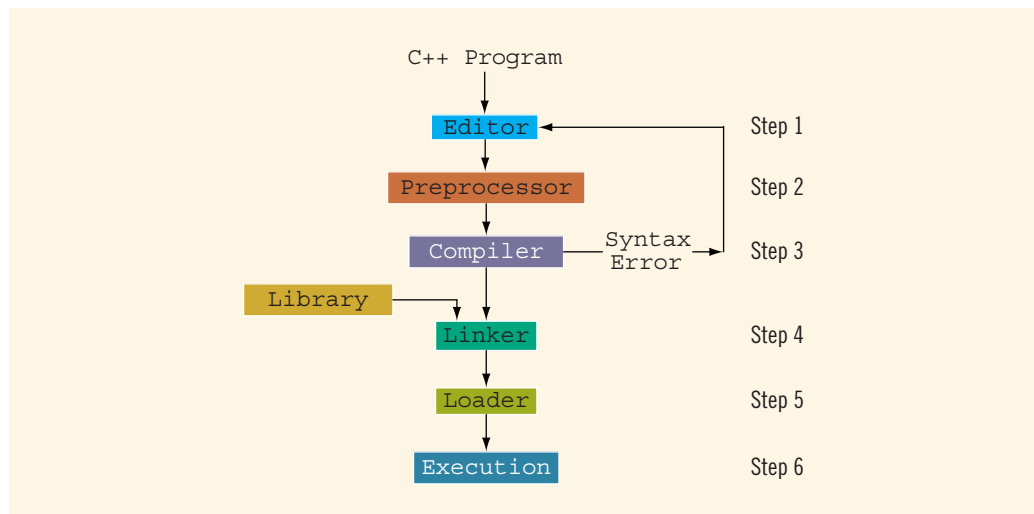
FIGURE 1-2 Processing a C++ program
