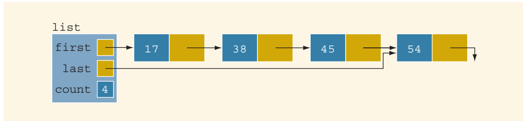
FIGURE 16-35 list before inserting 27
