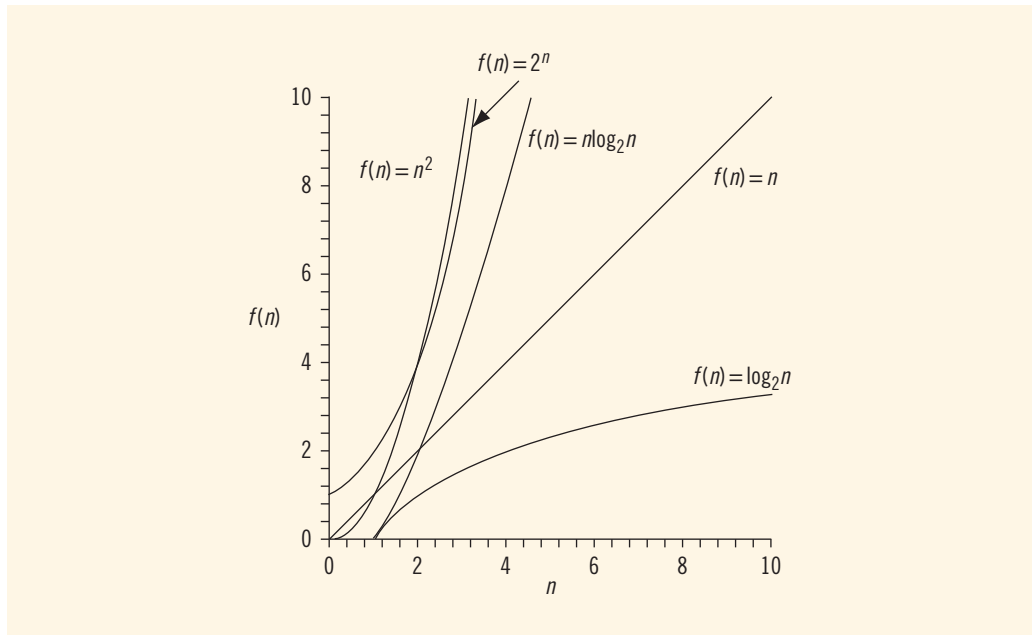
FIGURE 18-5 Growth rate of various functions
