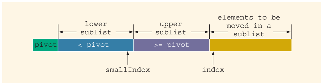
FIGURE 18-21 List during the execution of Step 2
