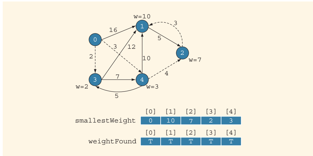
FIGURE 20-12 Graph after the fourth iteration of Steps 3, 4, and 5
