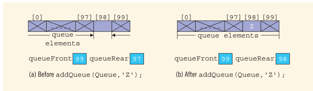
FIGURE 17-33 Queue before and after the add operation
