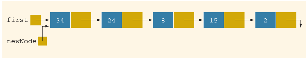
FIGURE 16-18 List after building it backward
