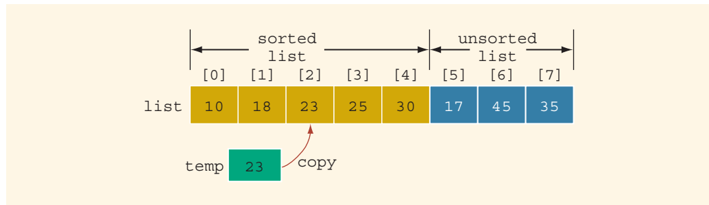
FIGURE 18-17 List after copying temp into list[2]
