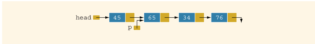
FIGURE 16-10 Node to be deleted is with info 34
