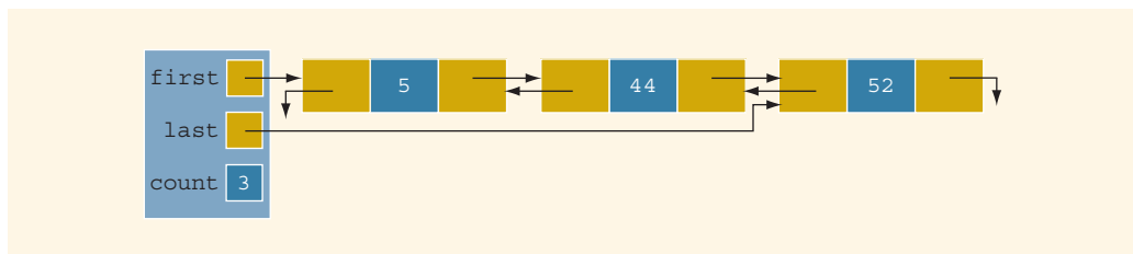
FIGURE 16-44 List after deleting the node with info 17
