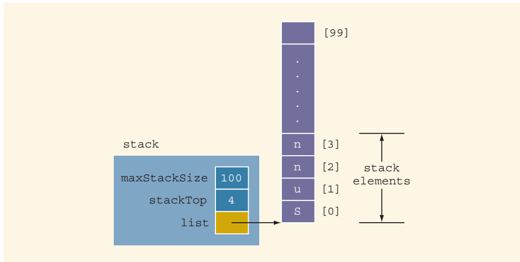
FIGURE 17-8 Stack before pushing y
