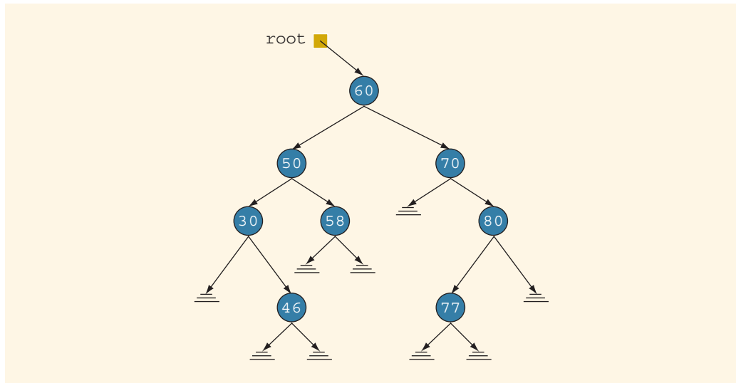
FIGURE 19-8 Binary search tree
