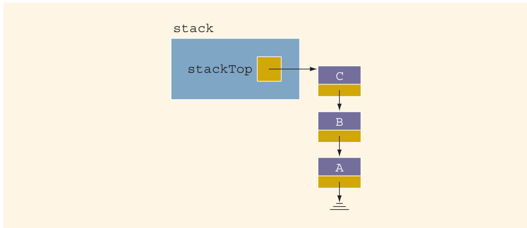
FIGURE 17-13 Stack before the push operation
