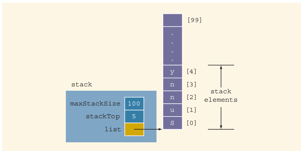
FIGURE 17-9 Stack after pushing y
