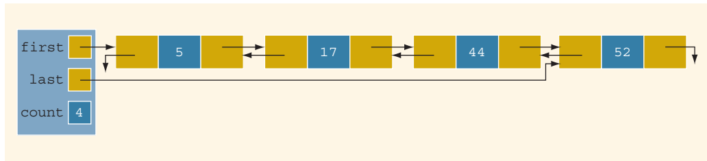
FIGURE 16-42 Doubly linked list before deleting 17
