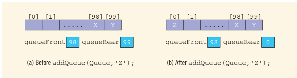
FIGURE 17-31 Queue before and after the add operation
