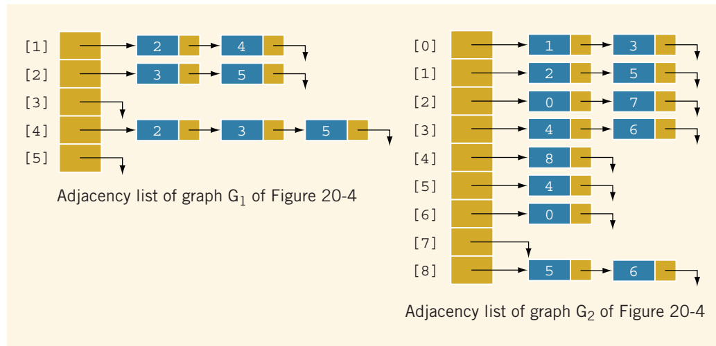
FIGURE 20-5 Adjacency list of graphs of Figure 20-4
