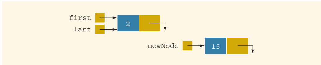
FIGURE 16-15 List and newNode with info 15
