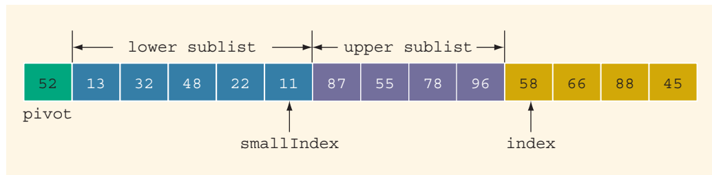
FIGURE 18-26 List before moving 58 into a sublist
