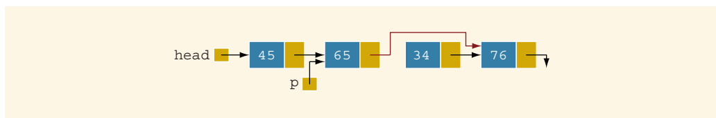
FIGURE 16-11 List after the statement newNode->link = q; executes
