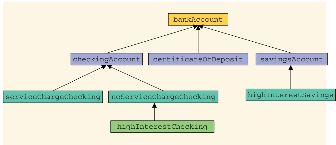
FIGURE 12-25 Inheritance hierarchy of banking accounts
