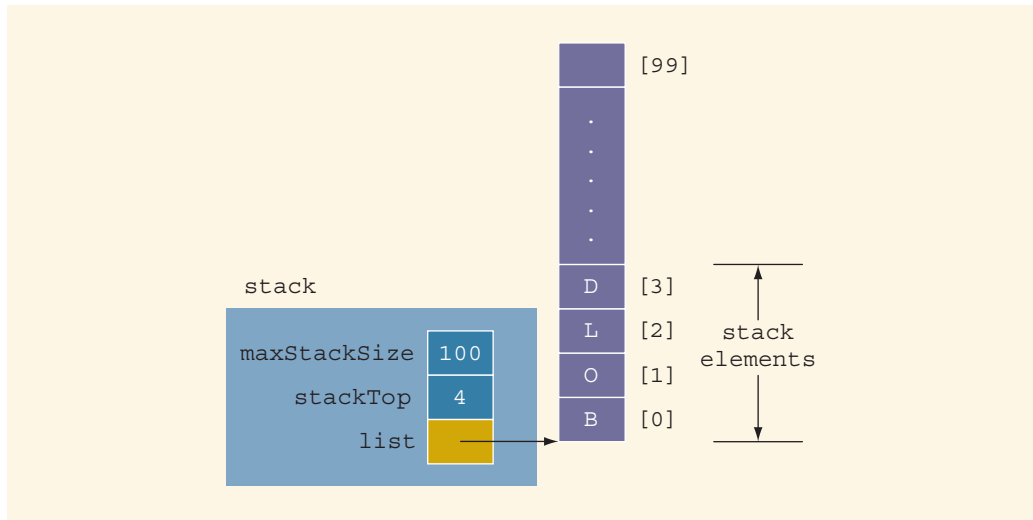
FIGURE 17-10 Stack before popping D
