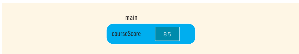
FIGURE 6-7 Variable courseScore after the statement in Line 6 is executed and control goes back to main
