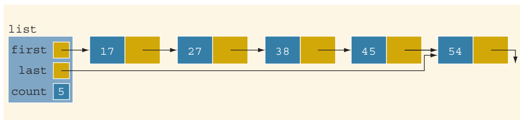
FIGURE 16-36 list after inserting 27
