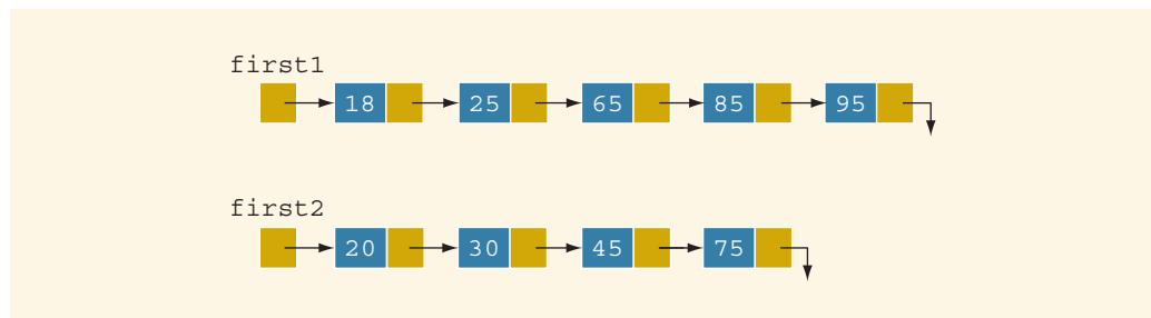
FIGURE 18-35 Sublists before merging
