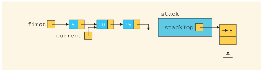
FIGURE 17-24 List and stack after the statements current = stack.top(); and stack.pop(); execute
