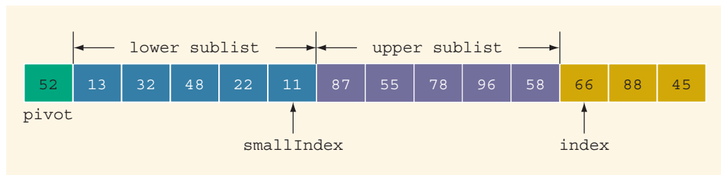
FIGURE 18-27 List after moving 58 into the upper sublist
