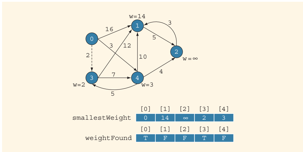
FIGURE 20-9 Graph after the first iteration of Steps 3, 4, and 5
