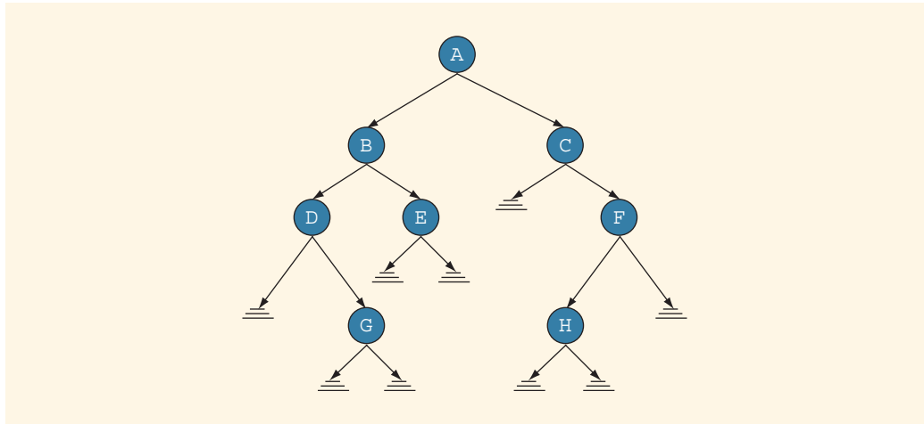
FIGURE 19-1 Binary tree
