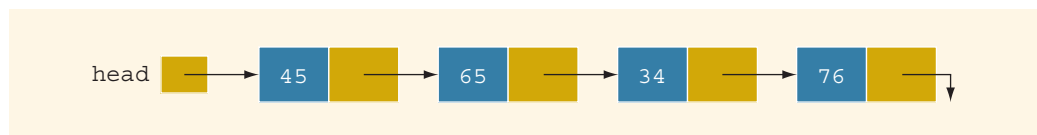
FIGURE 16-2 Linked list
