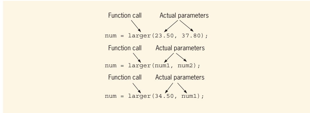
FIGURE 6-3 Function calls
