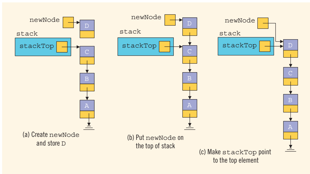
FIGURE 17-14 Push operation
