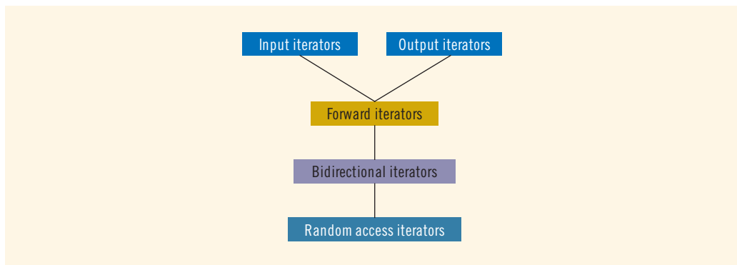
FIGURE 21-1 Iterator hierarchy
