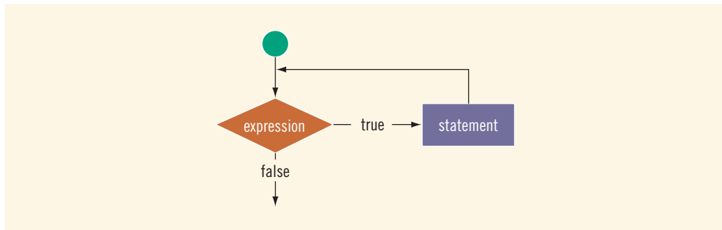
FIGURE 5-1 while loop
