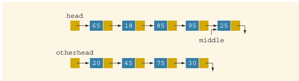
FIGURE 18-34 List after dividing it into two lists
