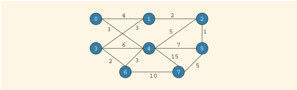
FIGURE 20-23 Graph for Exercise 21
