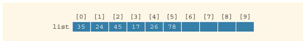
FIGURE 12-23 Array list
