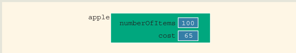
FIGURE 10-17 Object apple
