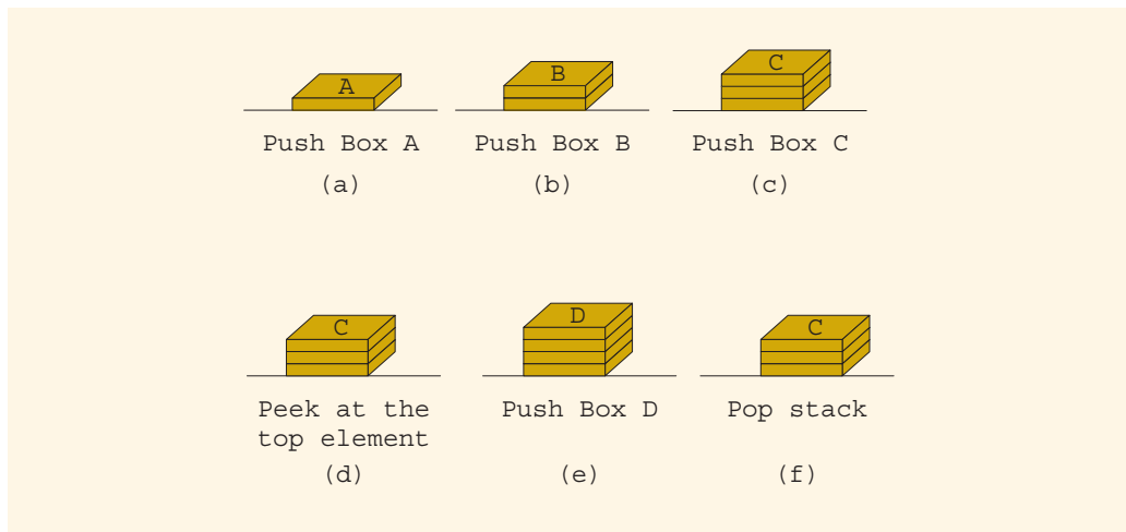
FIGURE 17-3 Stack operations
