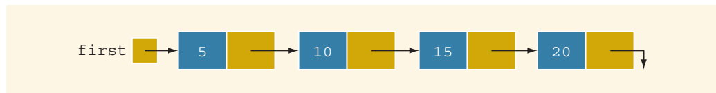
FIGURE 16-37 Linked list
