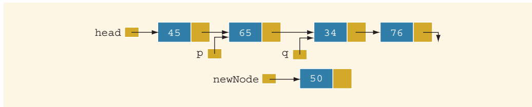
FIGURE 16-9 List with pointers p and q
