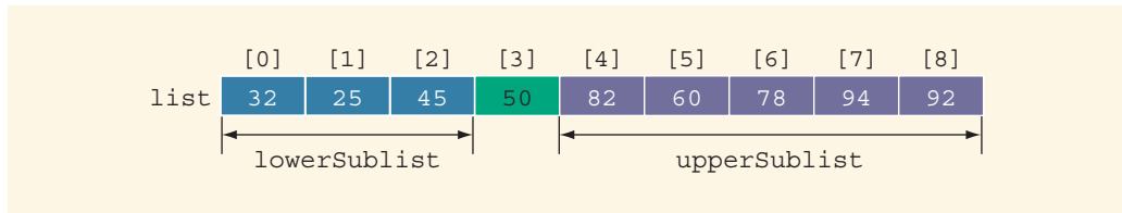
FIGURE 18-20 list after the partition
