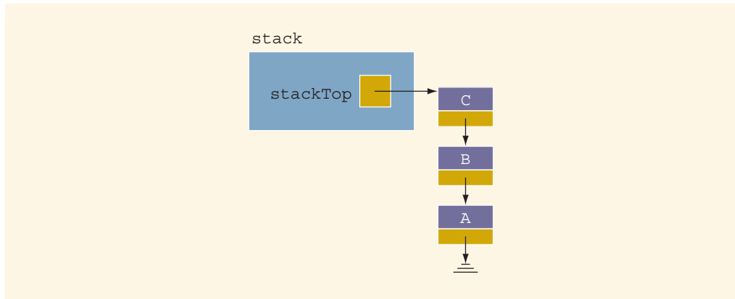
FIGURE 17-15 Stack before the pop operation
