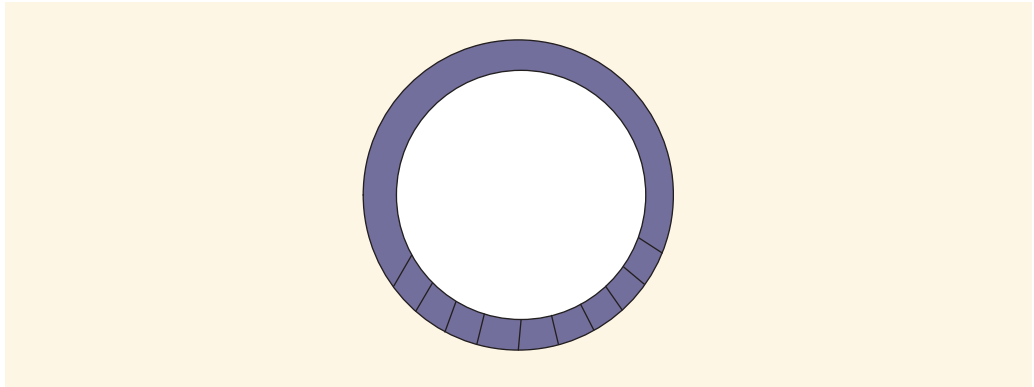
FIGURE 17-30 Circular queue
