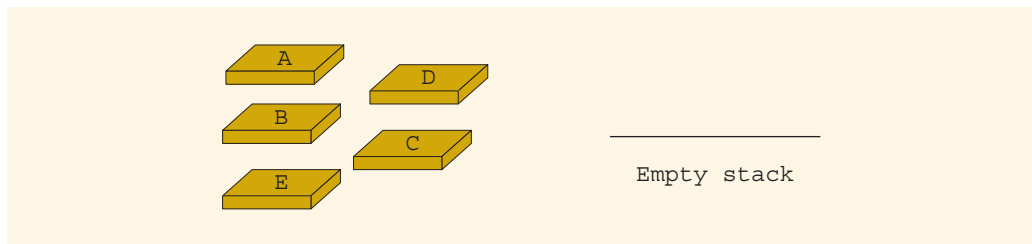
FIGURE 17-2 Empty stack
