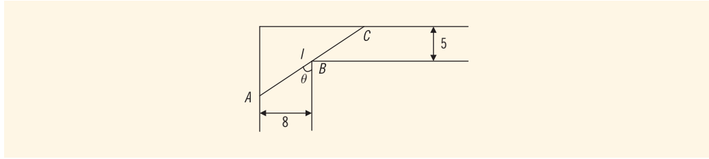
FIGURE 6-19 Pipe problem
