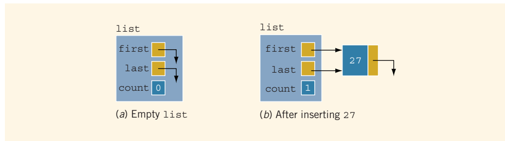
FIGURE 16-30 list
