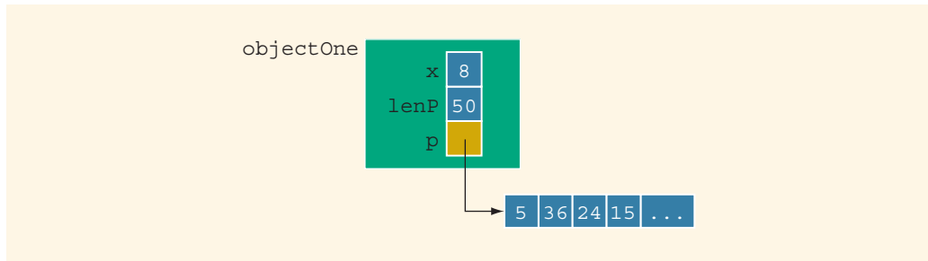
FIGURE 12-19 Object objectOne
