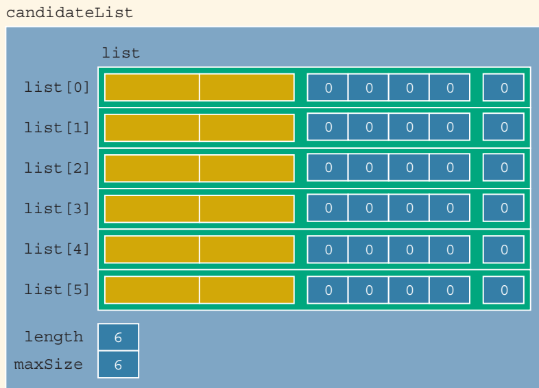
FIGURE 18-41 candidateList
