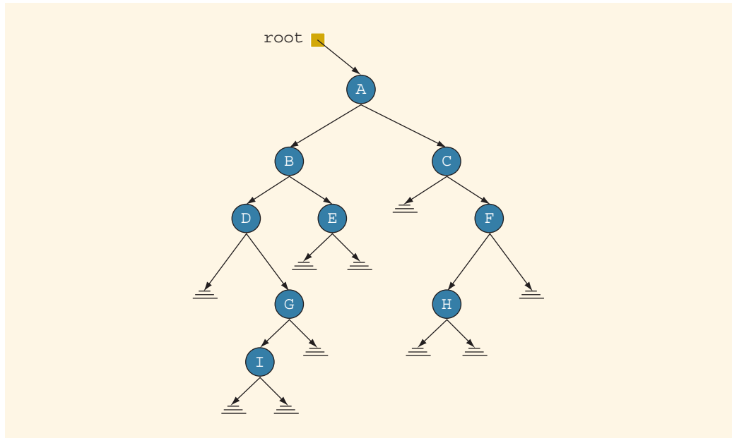
FIGURE 19-5 Binary tree
