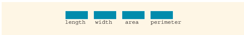
FIGURE 2-2 Memory allocation
