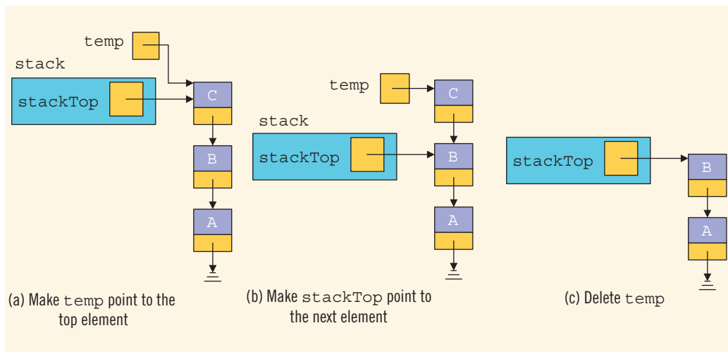
FIGURE 17-16 Pop operation
