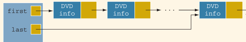
FIGURE 16-46 dvdList
