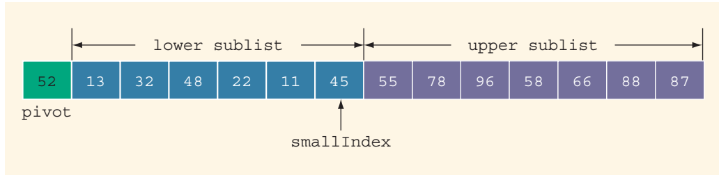
FIGURE 18-28 List elements after arranging into the lower sublist and upper sublist
