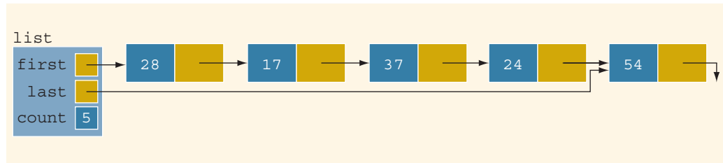
FIGURE 16-23 list with more than one node
