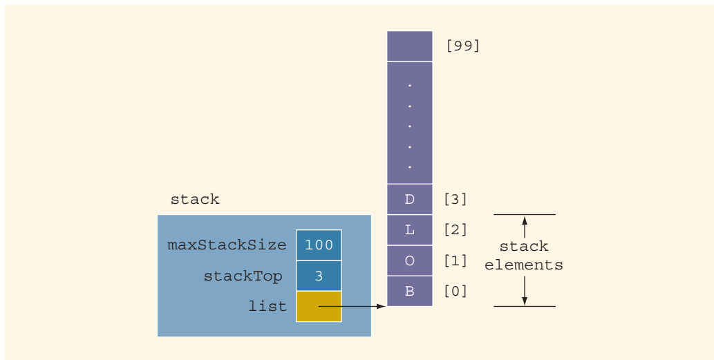
FIGURE 17-11 Stack after popping D
