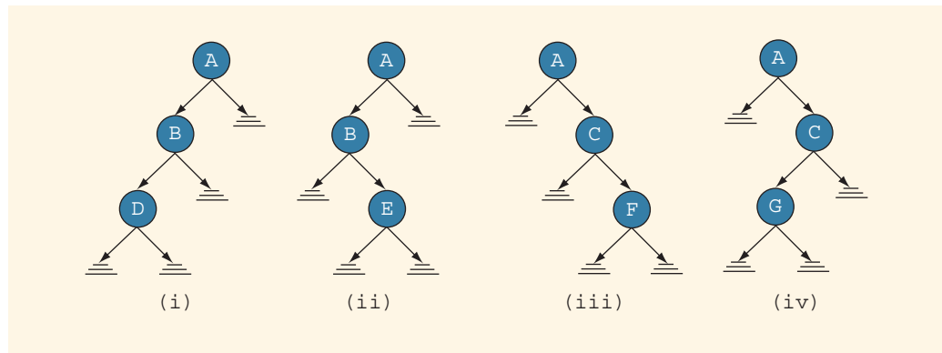
FIGURE 19-3 Various binary trees with three nodes
