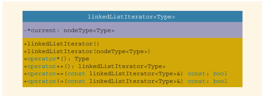
FIGURE 16-19 UML class diagram of the class linkedListIterator
