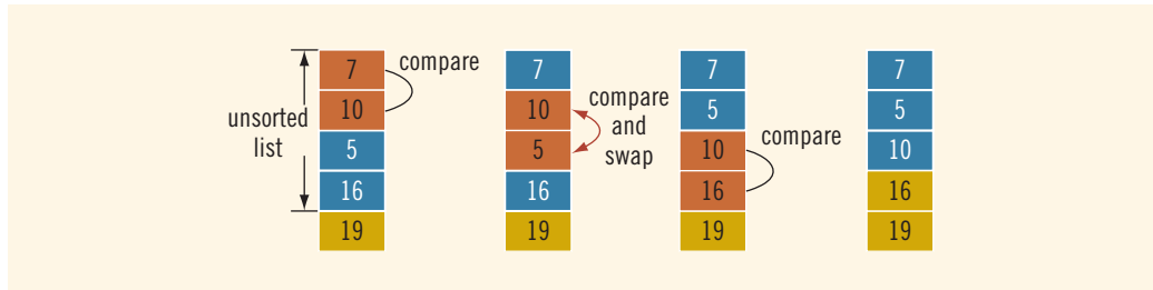
FIGURE 18-8 Elements of list during the second iteration
