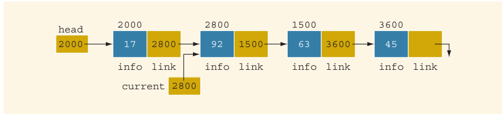
FIGURE 16-6 List after the statement current = current->link; executes
