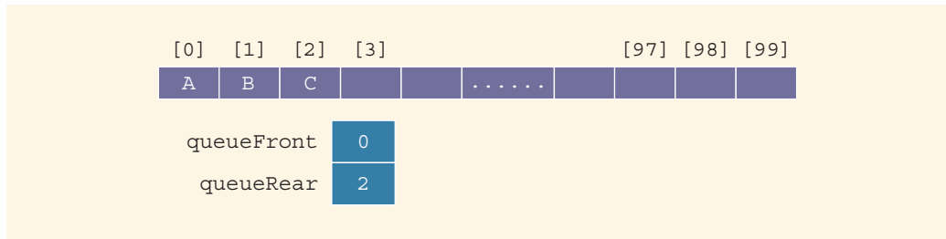
FIGURE 17-27 Queue after two more addQueue operations
