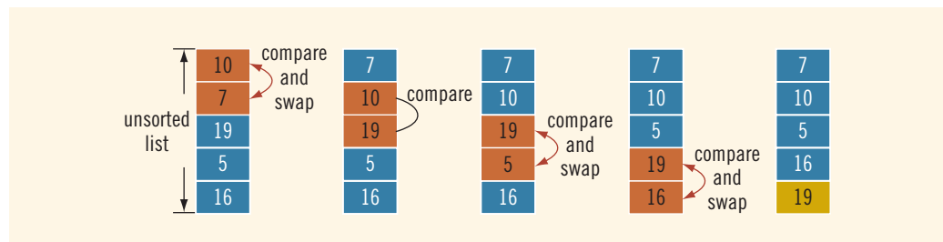
FIGURE 18-7 Elements of list during the first iteration
