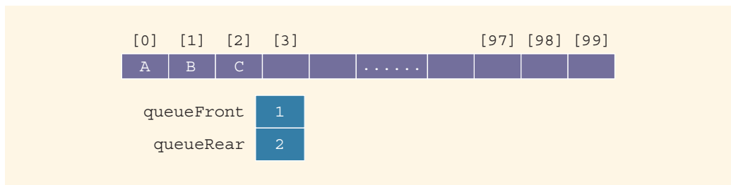
FIGURE 17-28 Queue after the deleteQueue operation
