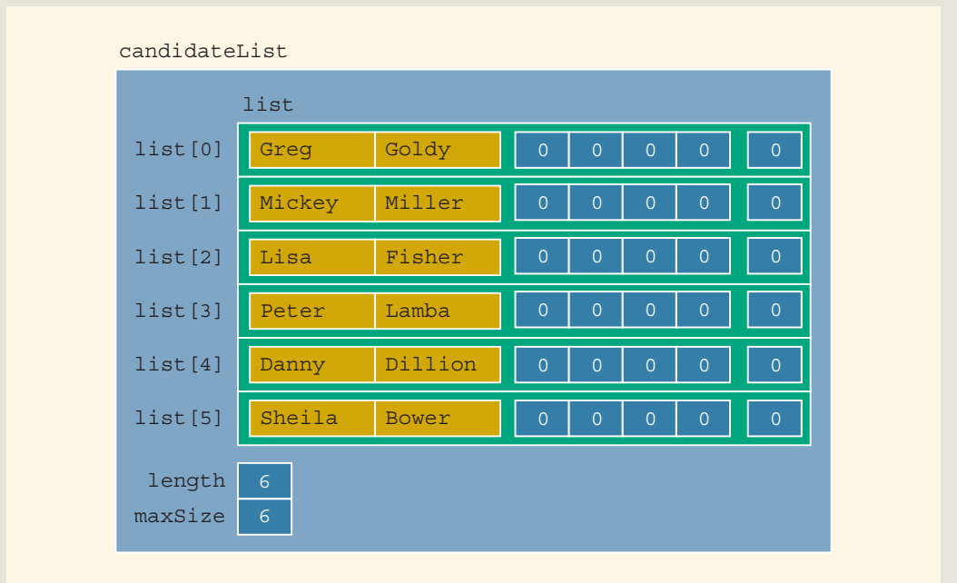
FIGURE 18-42 Object candidateList after a call to the function fillNames
