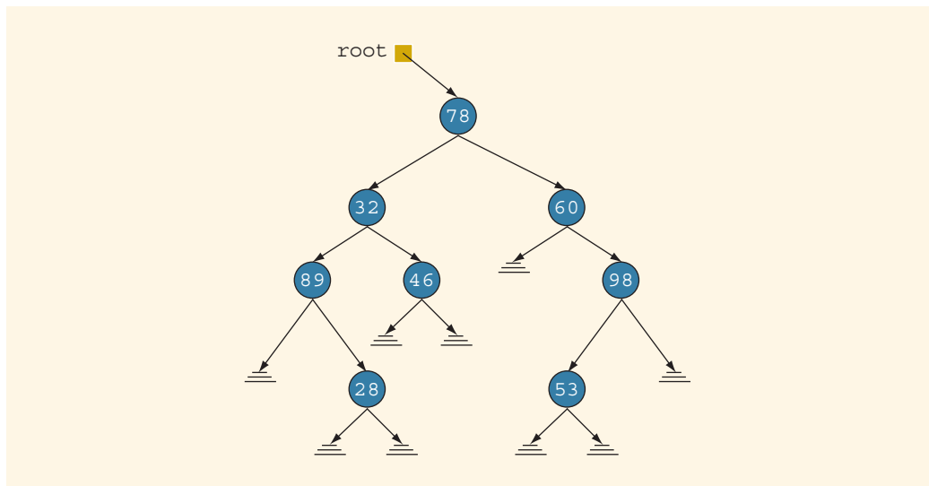
FIGURE 19-7 Arbitrary binary tree
