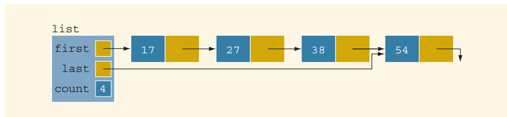
FIGURE 16-31 Nonempty list before inserting 10
