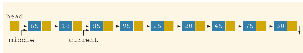
FIGURE 18-32 middle and current before traversing the list
