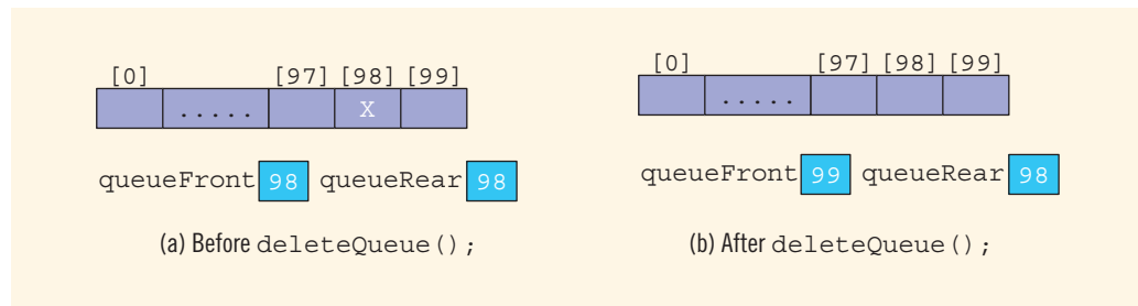
FIGURE 17-32 Queue before and after the delete operation
