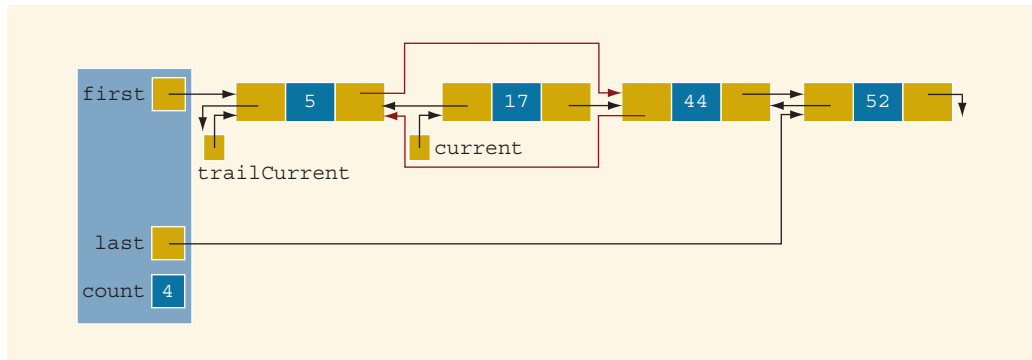
FIGURE 16-43 List after adjusting the links of the nodes before and after the node with info 17
