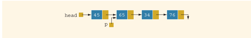
FIGURE 16-7 Linked list before item insertion
