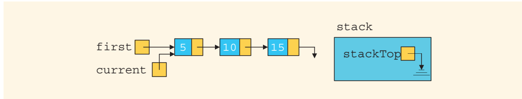
FIGURE 17-25 List and stack after the statements current = stack.top() ; and stack.pop() ; execute
