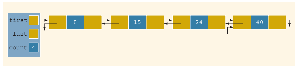
FIGURE 16-40 Doubly linked list before inserting 20
