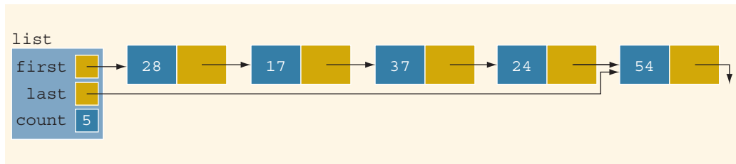
FIGURE 16-27 list before deleting 54
