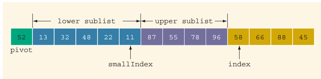
FIGURE 18-25 List after moving 11 into the lower sublist
