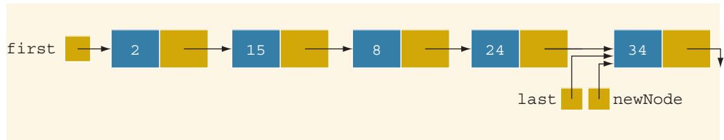
FIGURE 16-17 List after inserting 8, 24, and 34
