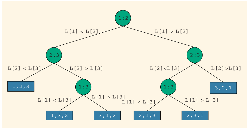
FIGURE 18-18 Comparison tree for sorting three items
