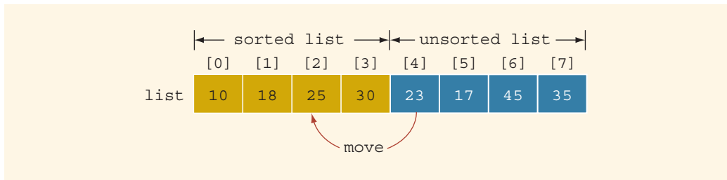
FIGURE 18-13 Move list[4] into list[2]
