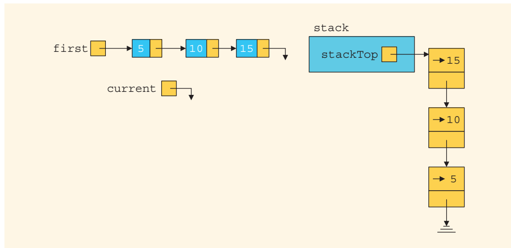
FIGURE 17-22 List and stack after the statements stack.push(current); and current = current->link; execute
