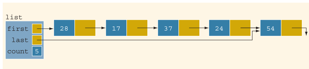
FIGURE 16-25 list before deleting 37
