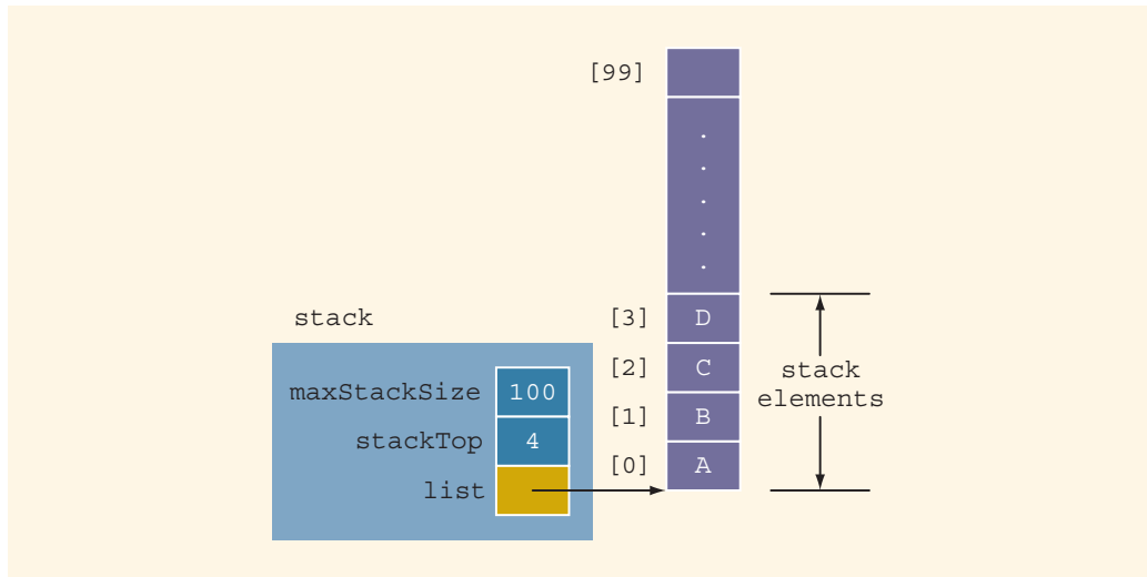
FIGURE 17-6 Example of a stack
