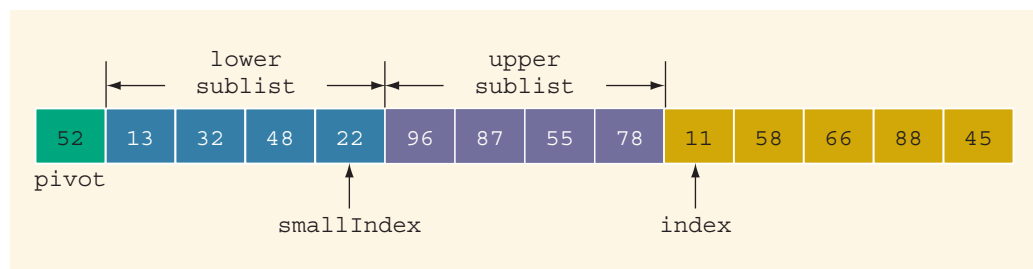
FIGURE 18-24 List after a few iterations of Step 2
