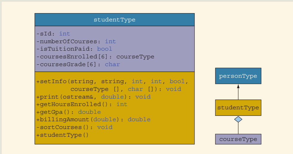
FIGURE 11-10 UML class diagram of the class studentType together with inheritance and composition (aggregation) relation
