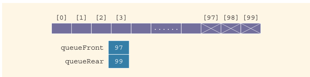
FIGURE 17-29 Queue after the sequence of operations AAADADADADADA...
