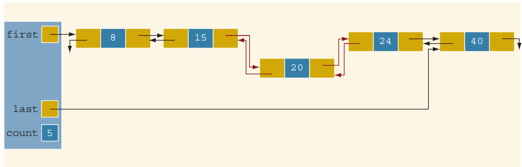
FIGURE 16-41 Doubly linked list after inserting 20
