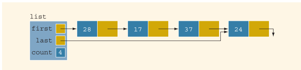
FIGURE 16-28 list after deleting 54
