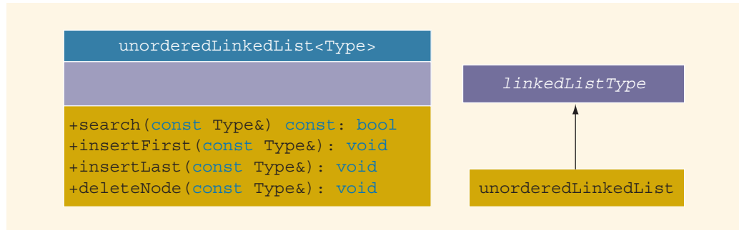
FIGURE 16-21 UML class diagram of the class unorderedLinkedList and inheritance hierarchy
