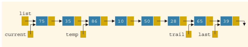
FIGURE 16-50 Linked list for Exercises 6 through 14
