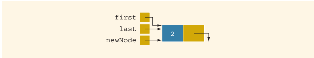
FIGURE 16-14 List after inserting newNode in it
