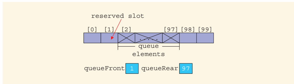
FIGURE 17-34 Array to store the queue elements with a reserved slot
