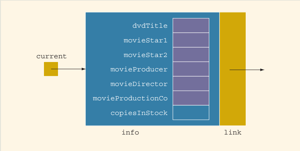
FIGURE 16-49 Pointer current and DVD list node
