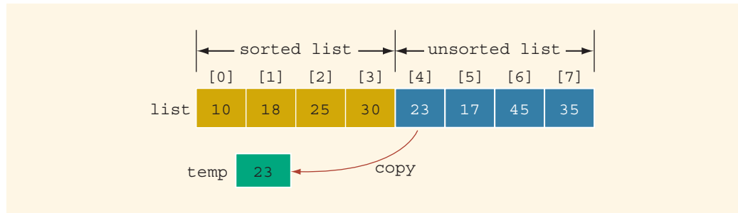
FIGURE 18-14 Copy list[4] into temp
