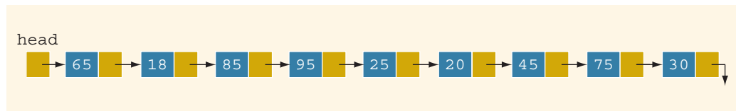
FIGURE 18-31 Unsorted linked list
