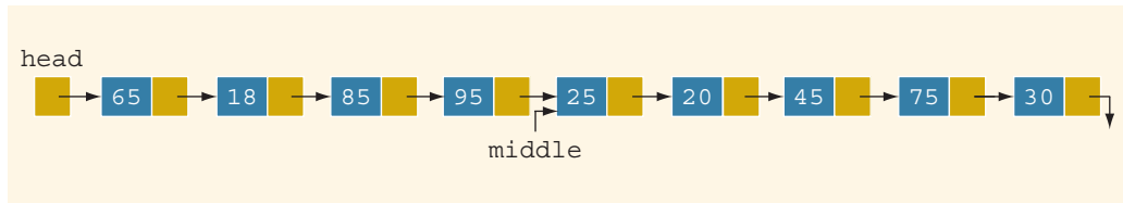
FIGURE 18-33 middle after traversing the list
