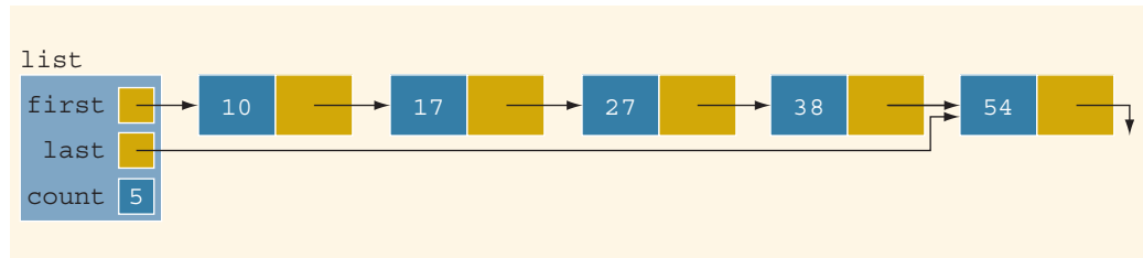
FIGURE 16-32 list after inserting 10
