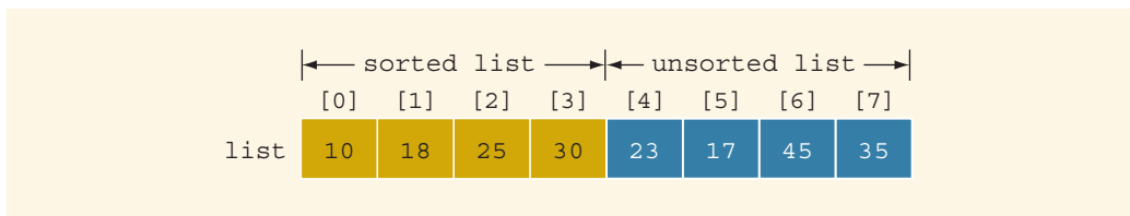
FIGURE 18-12 Sorted and unsorted portion of list
