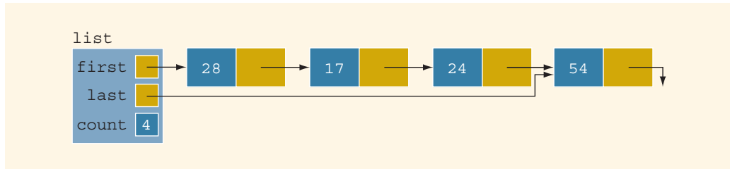
FIGURE 16-26 list after deleting 37
