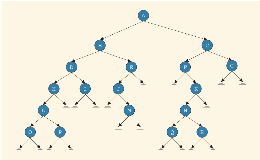
FIGURE 19-13 Figure for Exercises 3 to 20
