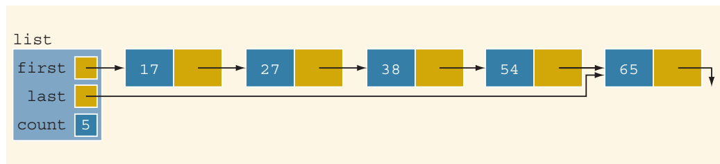
FIGURE 16-34 list after inserting 65
