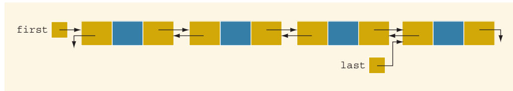
FIGURE 16-39 Doubly linked list
