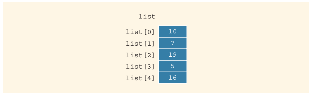
FIGURE 18-6 List of five elements
