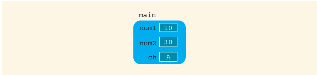
FIGURE 6-11 Values of the variables after the statement in Line 6
