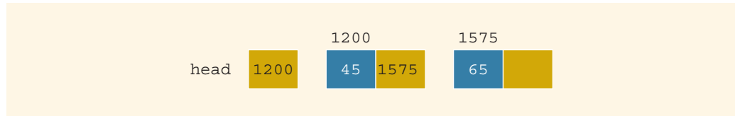
FIGURE 16-3 Linked list and values of the links
