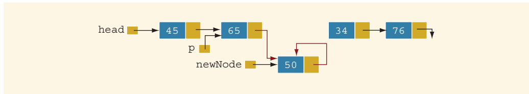
FIGURE 16-8 List after the execution of the statement p->link = newNode; followed by the execution of the statement newNode->link = p->link;
