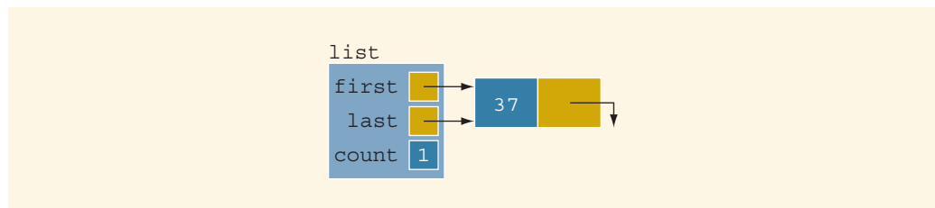
FIGURE 16-22 list with one node
