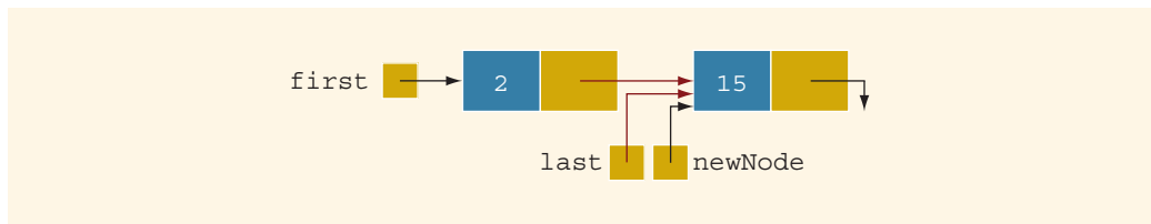
FIGURE 16-16 List after inserting newNode at the end
