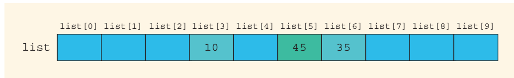
FIGURE 8-5 Array list after execution of the statements list[3]= 10; , list[6]= 35; , and list[5] = list[3] + list[6];
