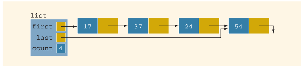
FIGURE 16-24 list after deleting node with info 28
