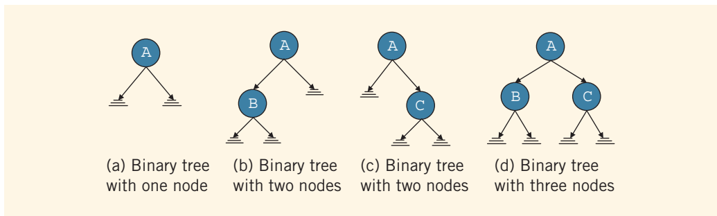
FIGURE 19-2 Binary tree with one, two, or three nodes
