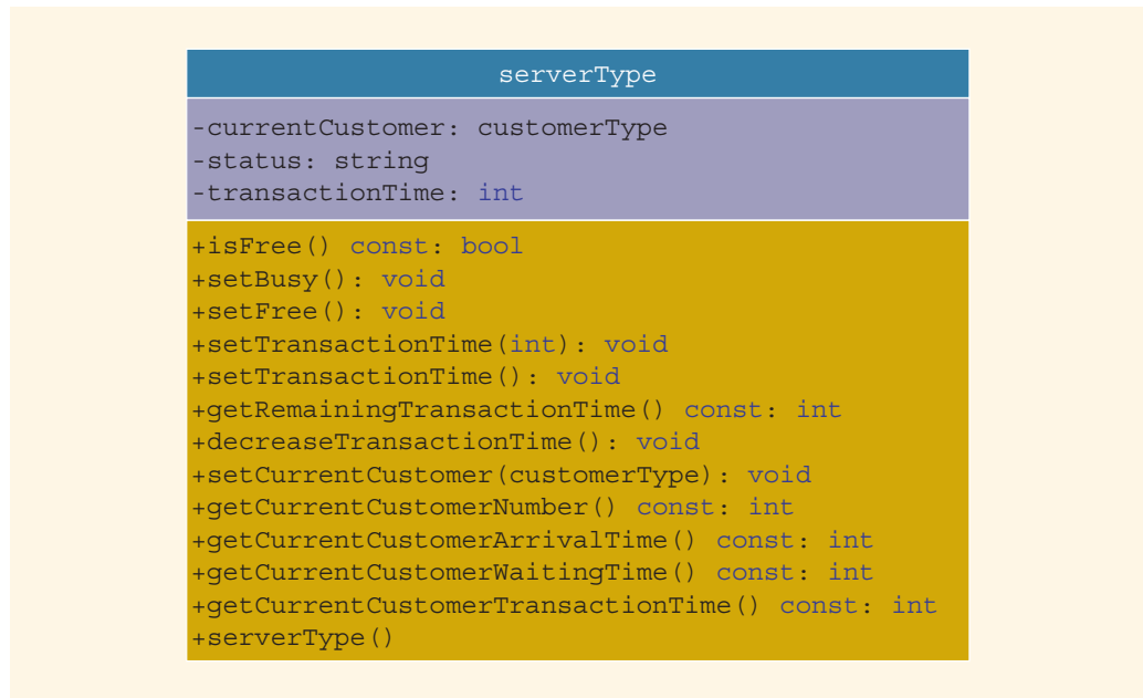
FIGURE 17-37 UML class diagram of the class serverType
