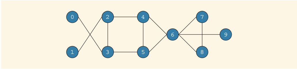
FIGURE 20-22 Graph for Exercise 20
