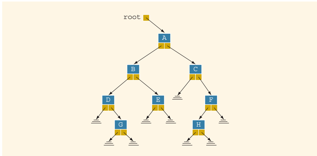
FIGURE 19-4 Binary tree
