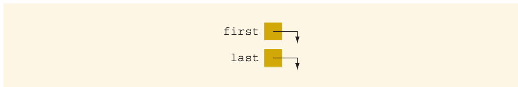
FIGURE 16-12 Empty list
