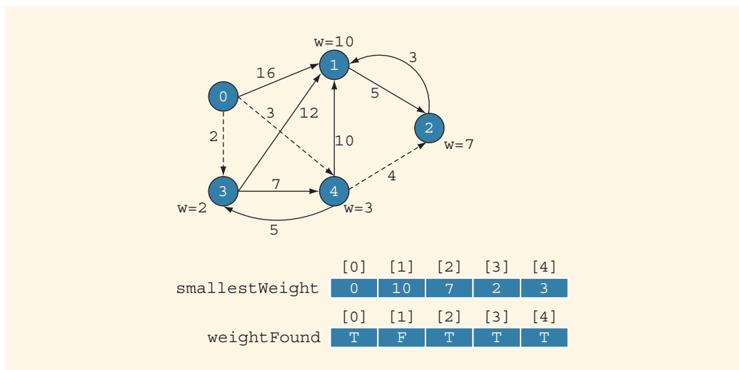
FIGURE 20-11 Graph after the third iteration of Steps 3, 4, and 5
