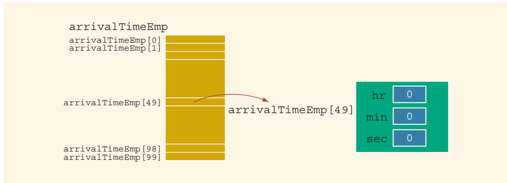
FIGURE 10-8 Array arrivalTimeEmp
