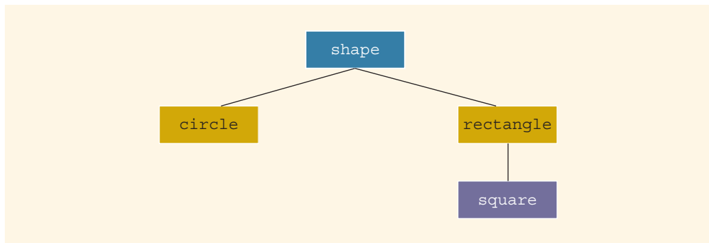
FIGURE 11-1 Inheritance hierarchy
