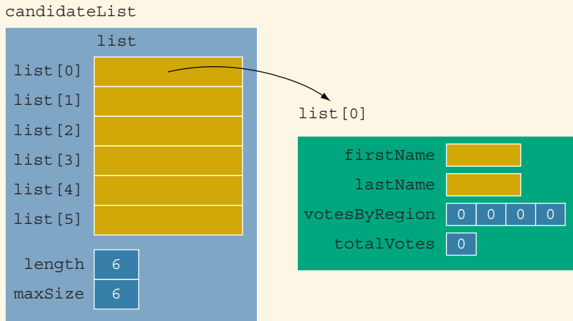
FIGURE 18-40 candidateList
