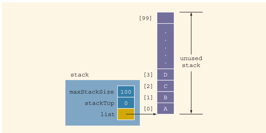
FIGURE 17-7 Empty stack
