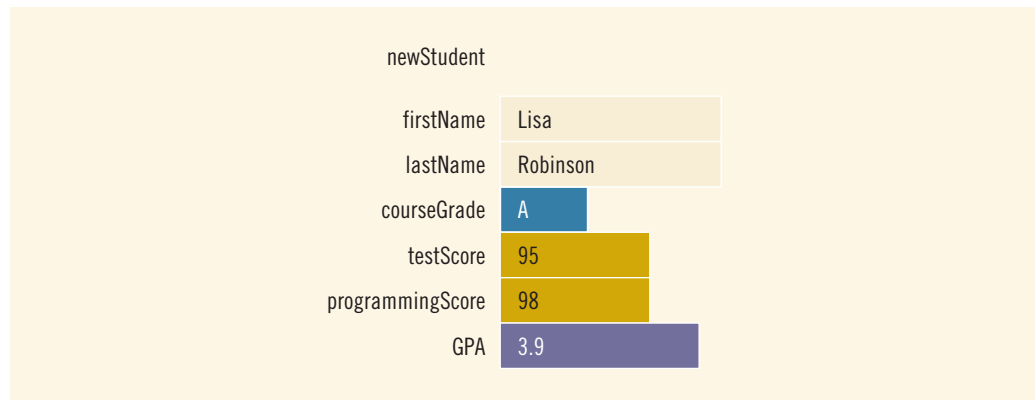
FIGURE 9-3 struct newStudent
