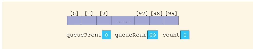
FIGURE 17-35 Empty queue
