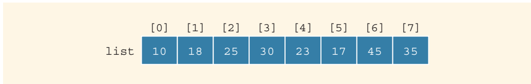
FIGURE 18-11 list
