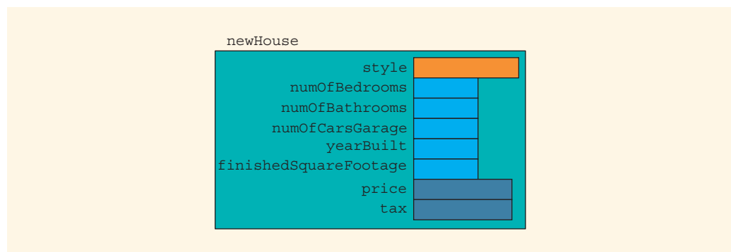
FIGURE 9-1 struct newHouse
