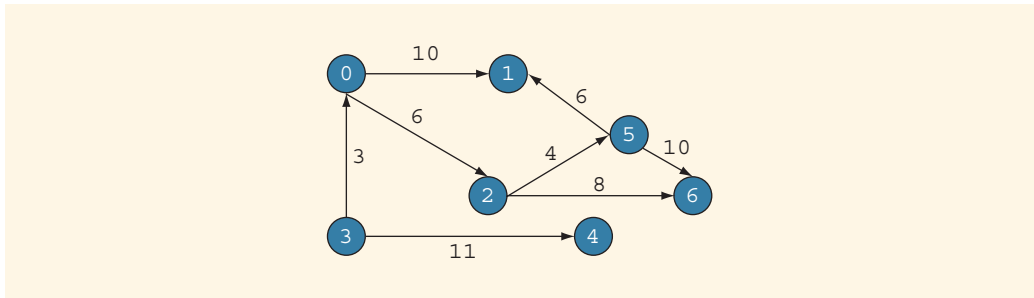
FIGURE 20-19 Graph for Exercise 17
