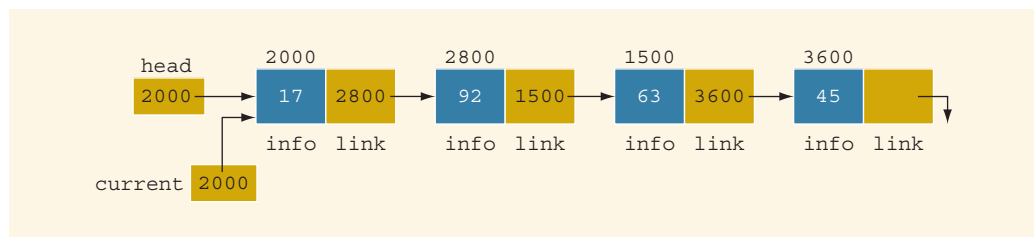
FIGURE 16-5 Linked list after the statement current = head; executes
