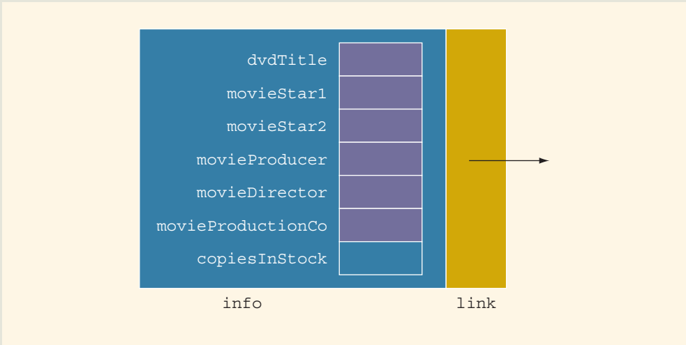
FIGURE 16-48 DVD list node showing components of info
