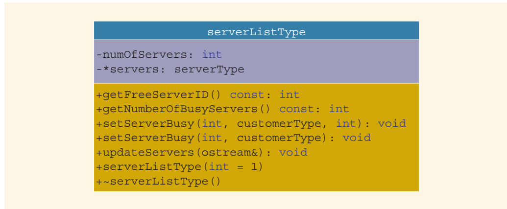
FIGURE 17-38 UML class diagram of the class serverListType
