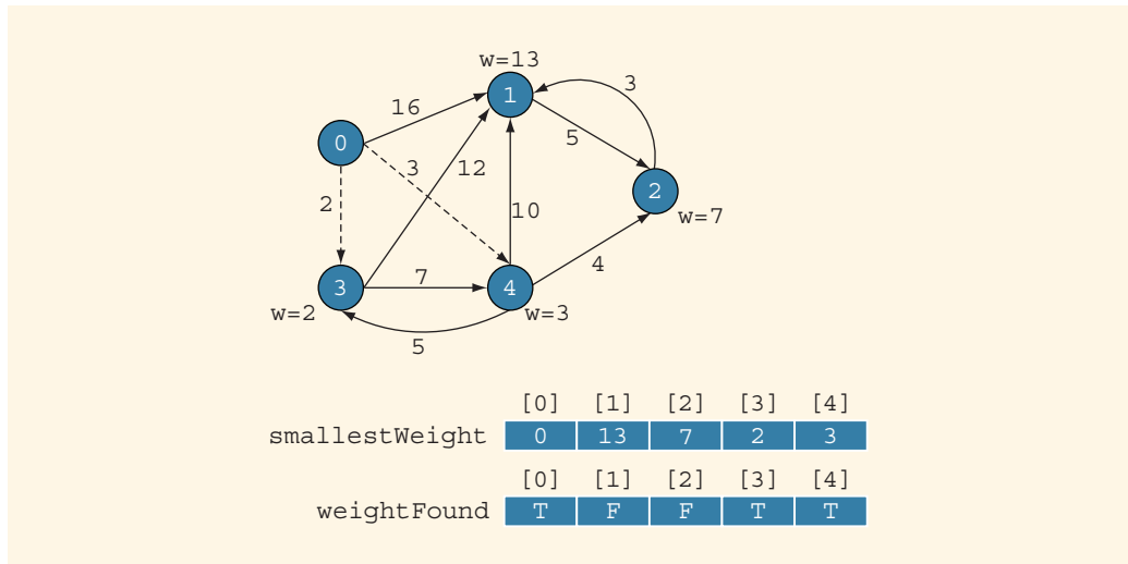
FIGURE 20-10 Graph after the second iteration of Steps 3, 4, and 5
