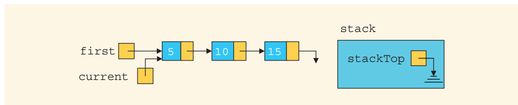
FIGURE 17-19 List after the statement current = first; executes
