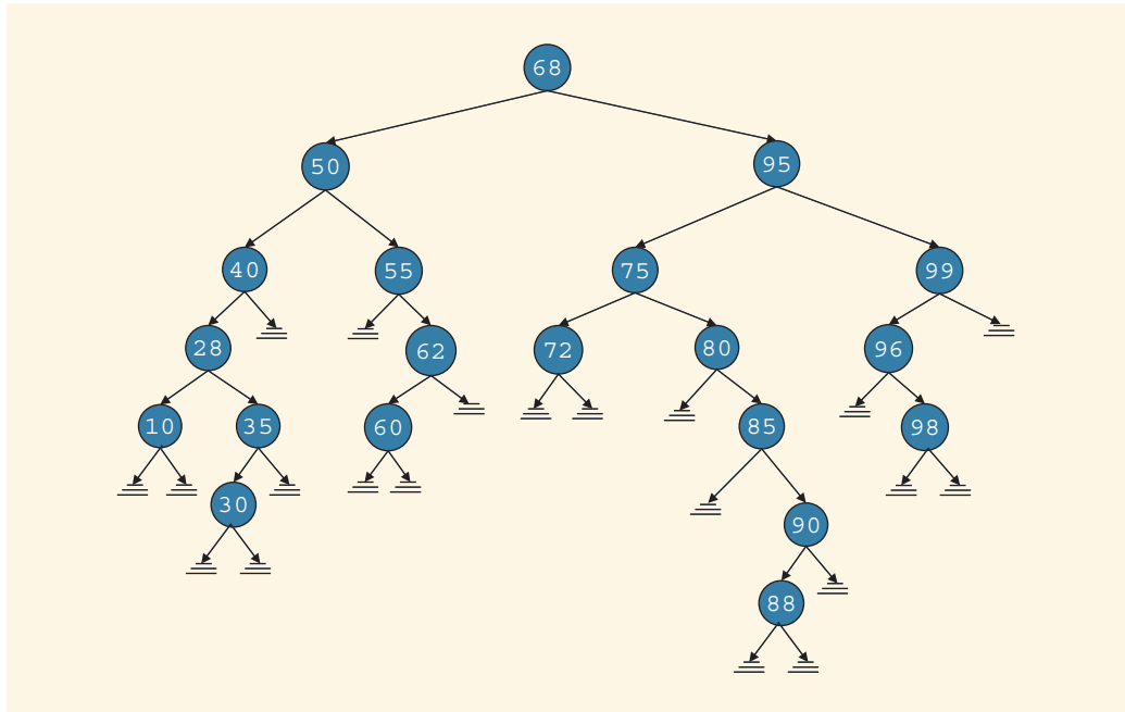
FIGURE 19-14 Figure for Exercises 21 to 25
