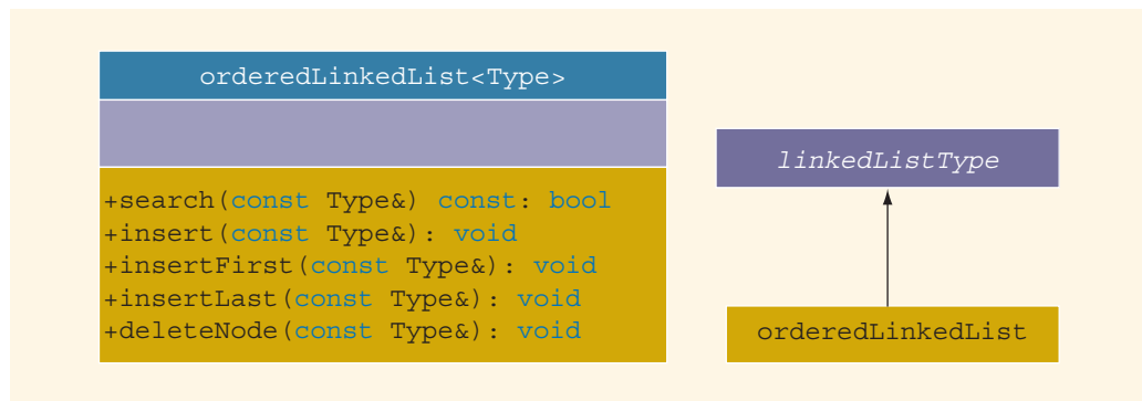
FIGURE 16-29 UML class diagram of the class orderedLinkedList and the inheritance hierarchy
