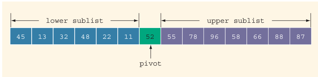
FIGURE 18-29 List after swapping 52 with 45
