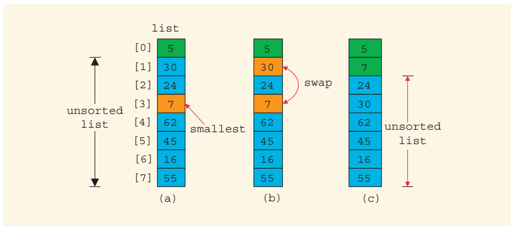
FIGURE 8-11 Elements of list during the second iteration
