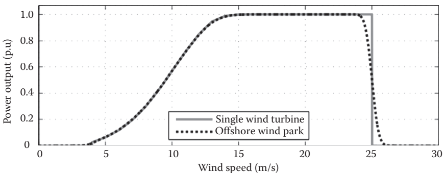
FIGURE 9.6 Example of a multiturbine power curve for an offshore wind park. (Adapted from A. J. Brand, M. Gibescu, and W. W. de Boer. in Wind Power , S M Mueyen (ed.). Croatia: InTech, 2010. ISBN: 978-953-7619-81-7; Available at: http://www.intechopen.com/articles/show/title/variability-and-predictability-of-large-scale-wind-energy-in-the-netherlands .)
