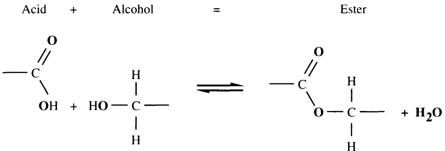
Figure 1.3 An ester is the result of a reaction of an alcohol with an acid (such as carboxylic acid). The sign \rightleftharpoons indicates that the reaction can proceed in both direction. Proceeding from left to right, an ester and a water molecule are products, while from right to left, a water molecule is broken down, a process called hydrolysis .
