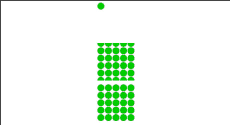
Figure 2-38. no-repeat , repeat-x , and repeat-y in Chrome
