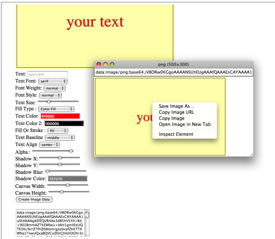
Figure 3-11. Canvas exported image with toDataURL()
