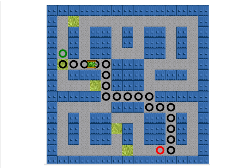
Figure 8-18. A* tank moving through path with no diagonal nodes
