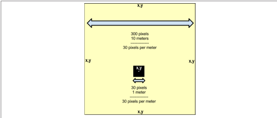
Figure 5-25. MTS conversion to pixels in Box2D
