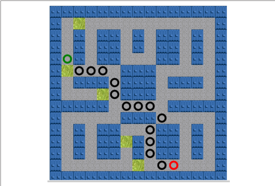
Figure 8-17. A* with grass tiles and diagonals
