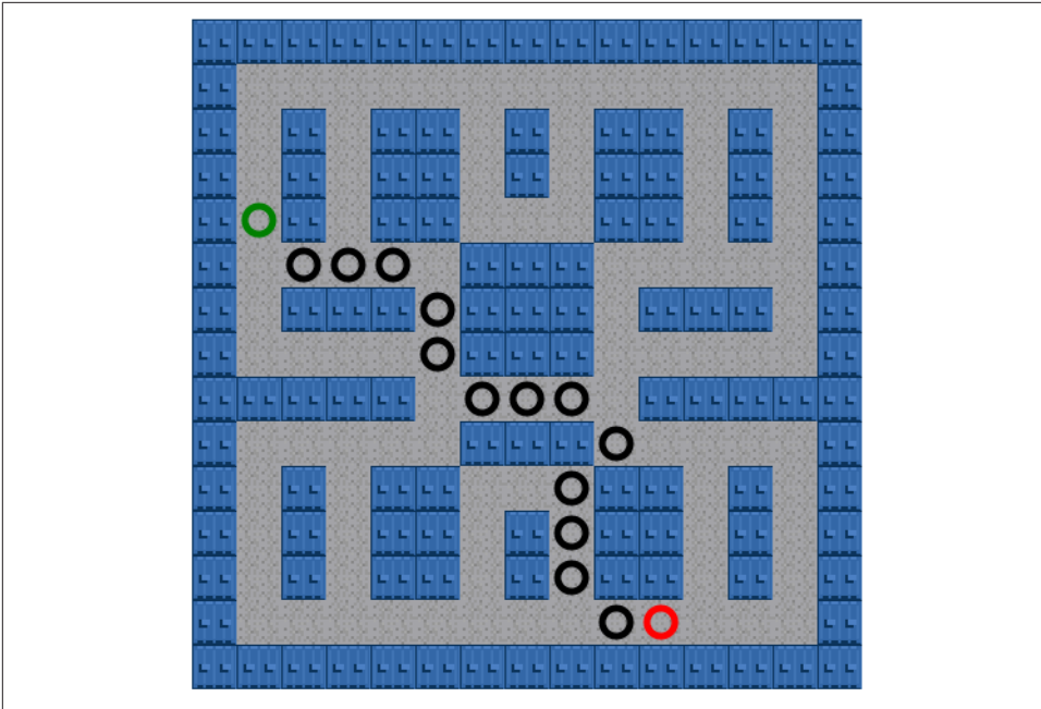
Figure 8-15. A* applied to the 15x15 tile map with diagonals
