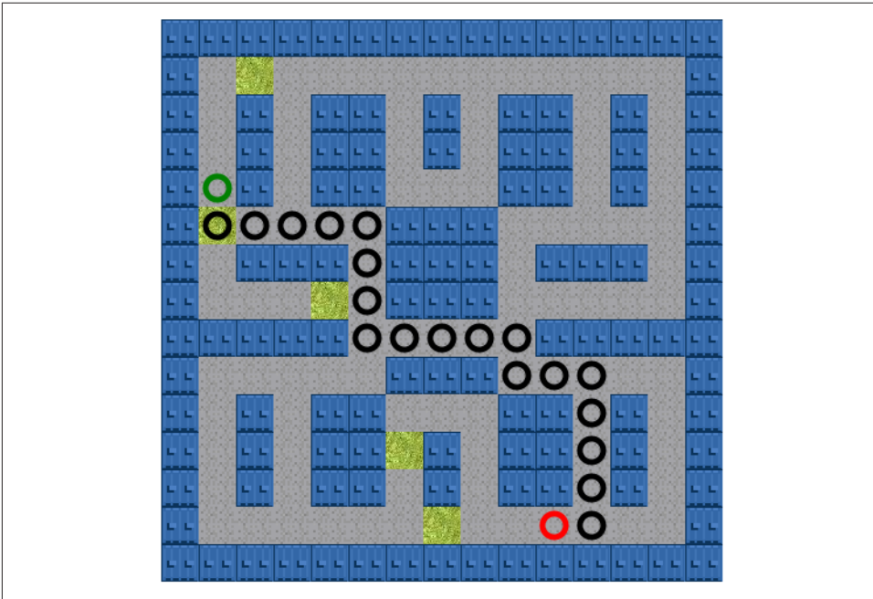
Figure 8-16. Example 8-16—A* with grass tiles
