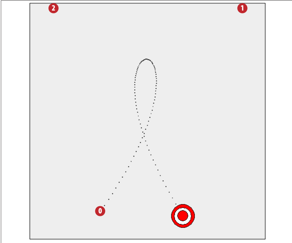
Figure 5-17. Moving an object in a loop using a cubic Bezier curve
