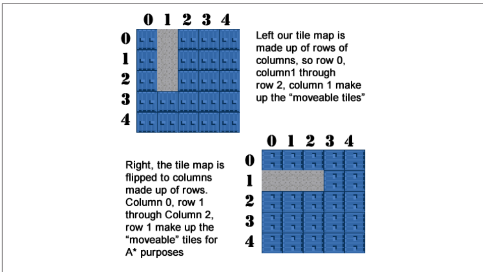
Figure 8-11. The Example 8-13 tile map vs. the A* tile map
