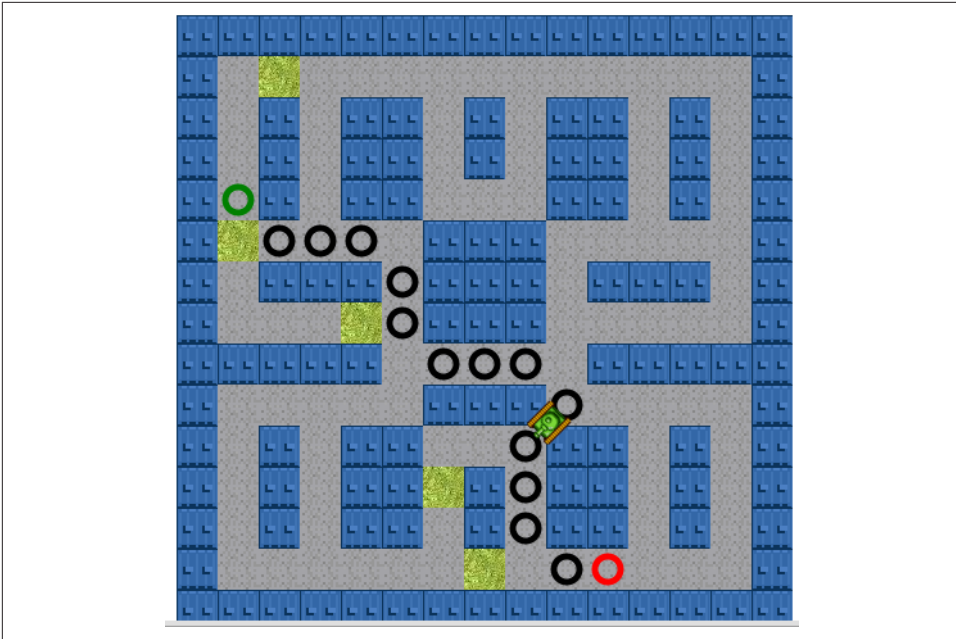
Figure 8-19. A* tank moving through path with diagonal and possible pass through
