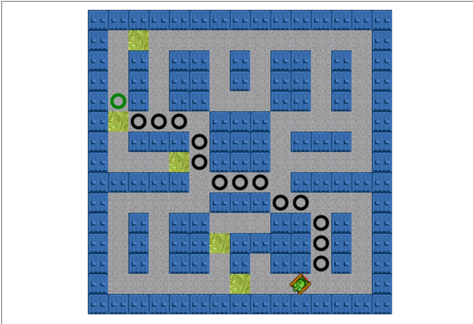
Figure 8-20. A* tank moving through the maze, with added walls to create impassible diagonal barriers
