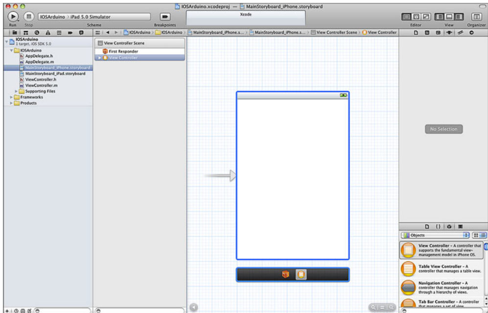
Figure 10.7 MainStoryboard_iPhone.storyboard view
