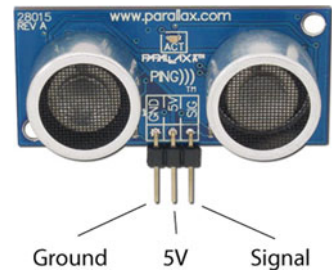
Figure 6.3 The Parallax Ping, an ultrasonic sensor
