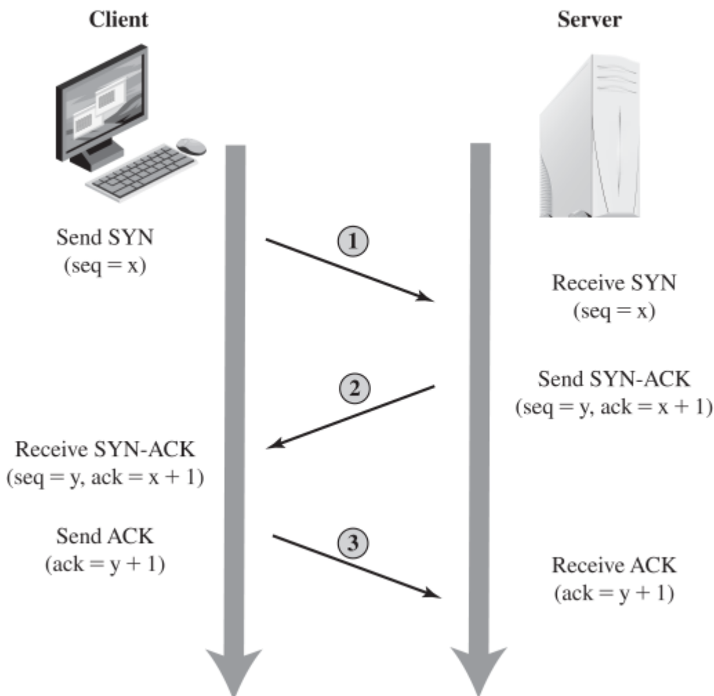
Figure 7.2 TCP Three-Way Connection Handshake
