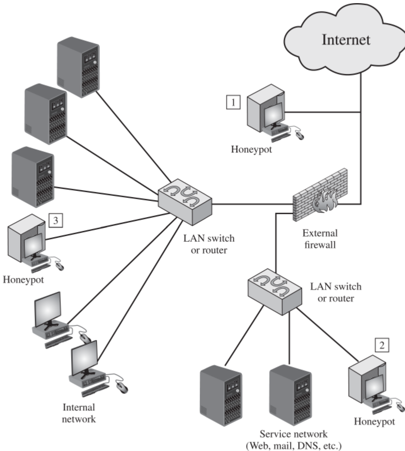
Figure 8.8 Example of Honeypot Deployment
