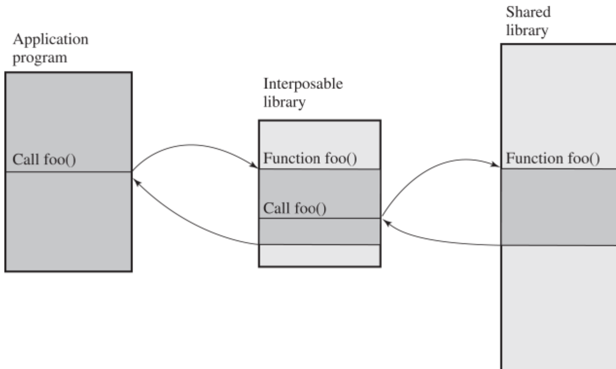
(b) Library call with interposition
