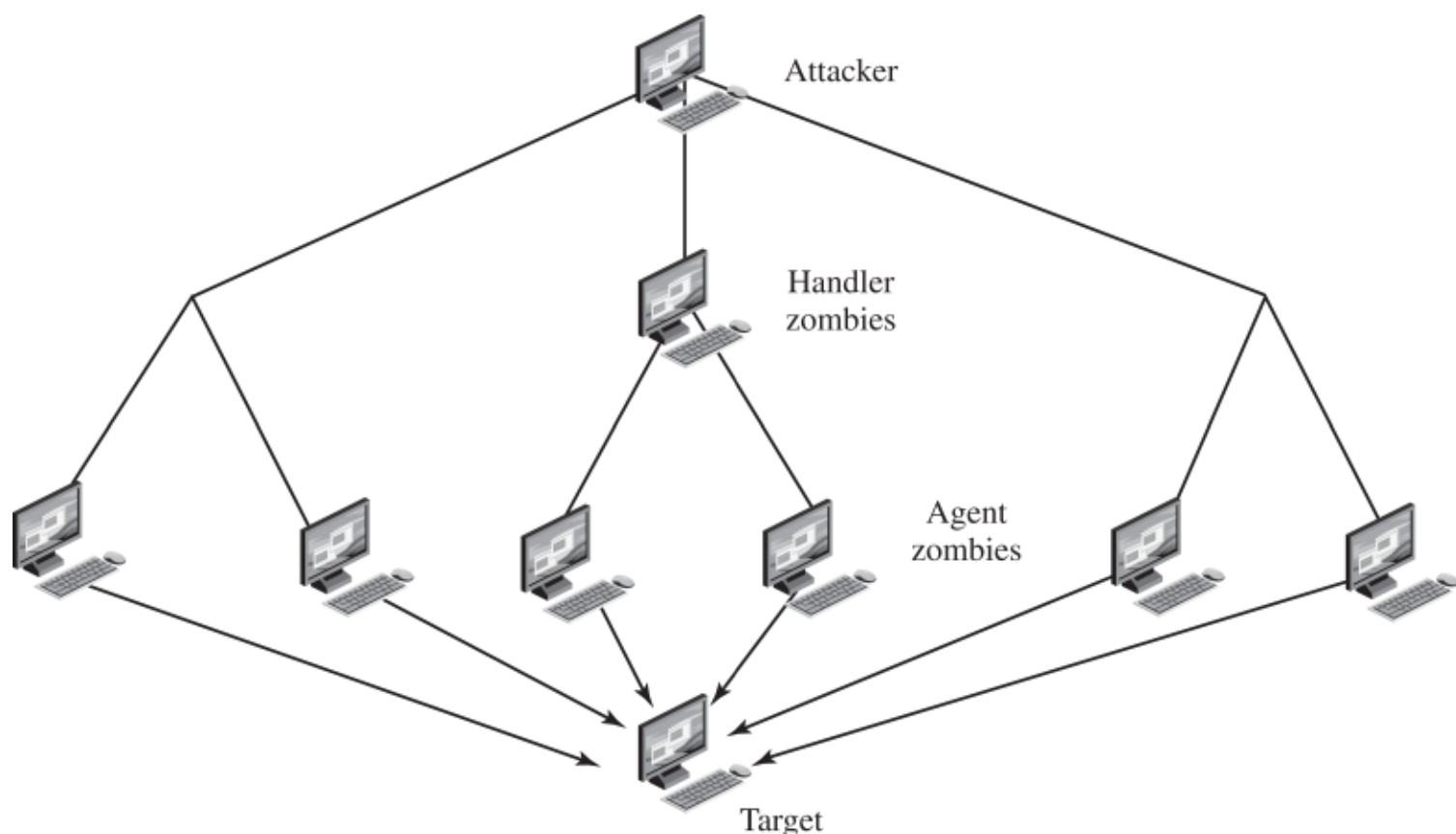
Figure 7.4 DDoS Attack Architecture
