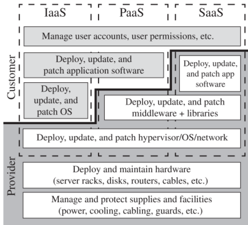
(b) Cloud computing management tasks
