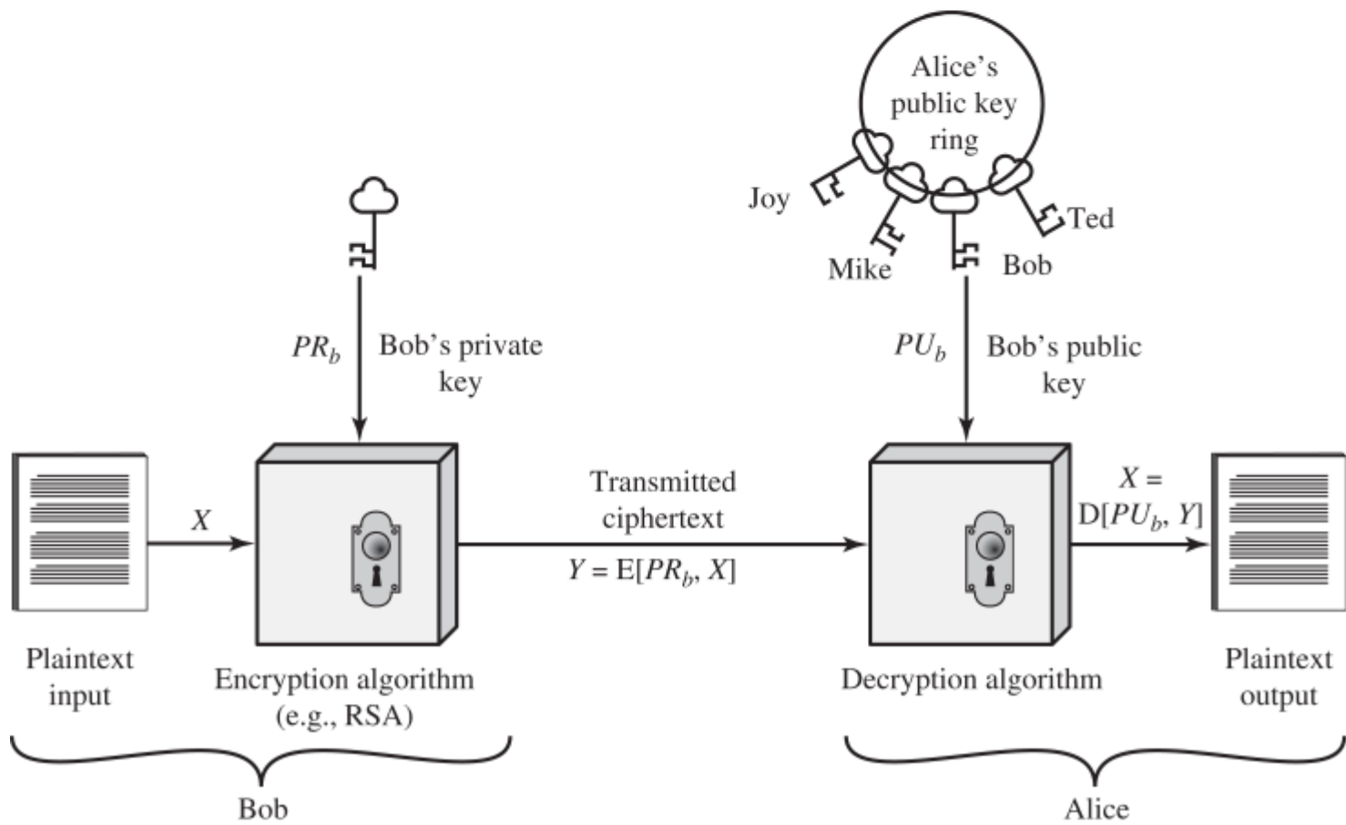
(b) Encryption with private key
