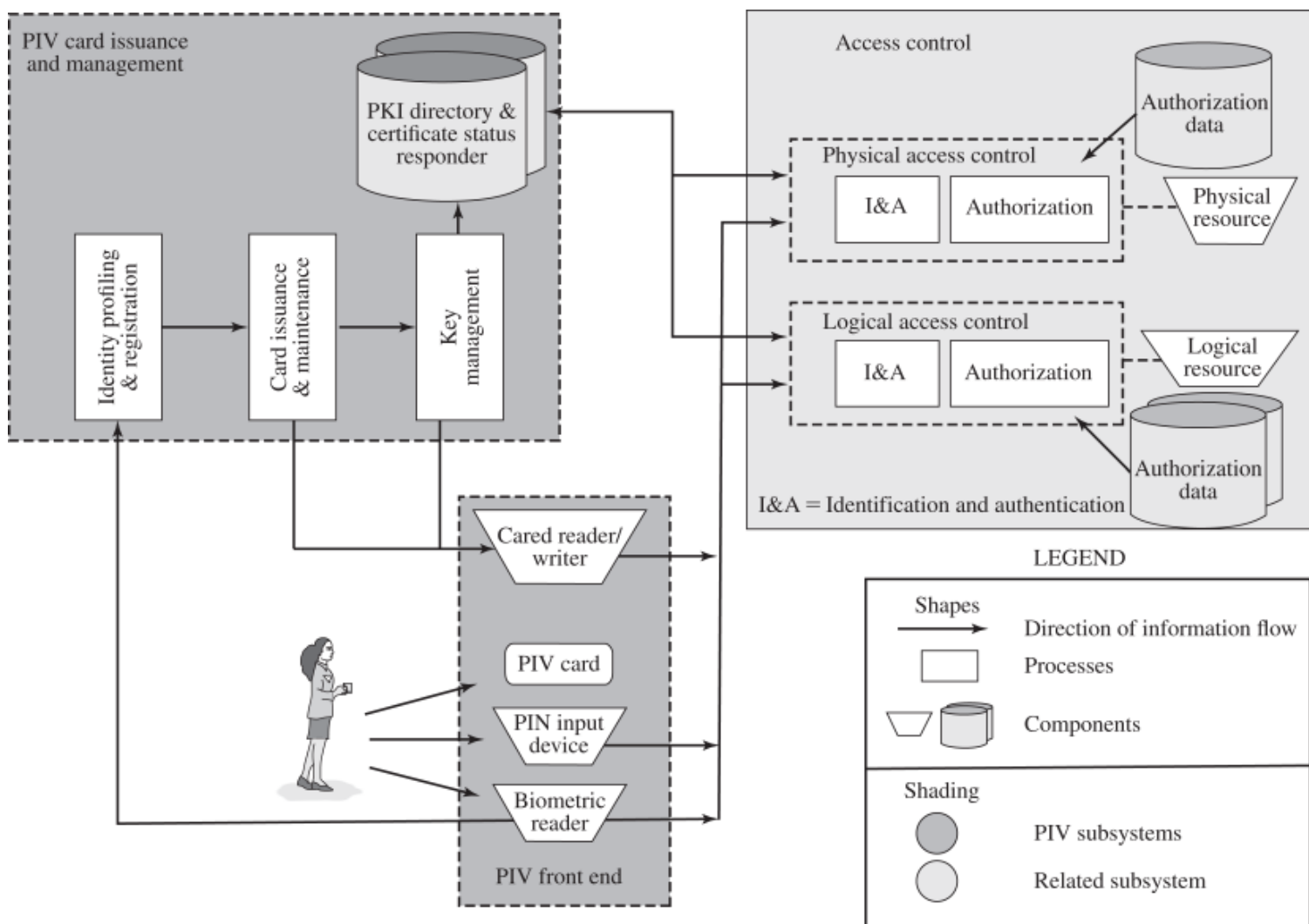
Figure 16.2 FIPS 201 PIV System Model
