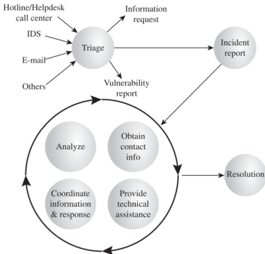
Figure 17.2 Incident Handling Life Cycle
