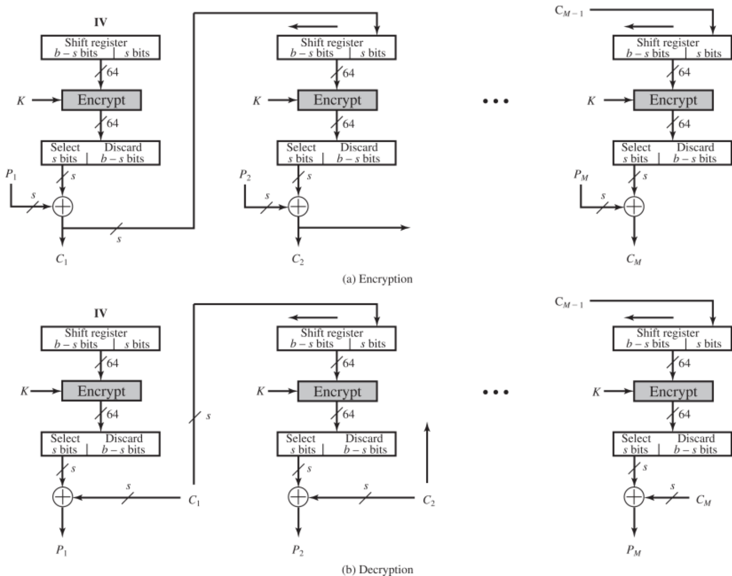
Figure 20.8 s-bit Cipher Feedback (CFB) Mode
