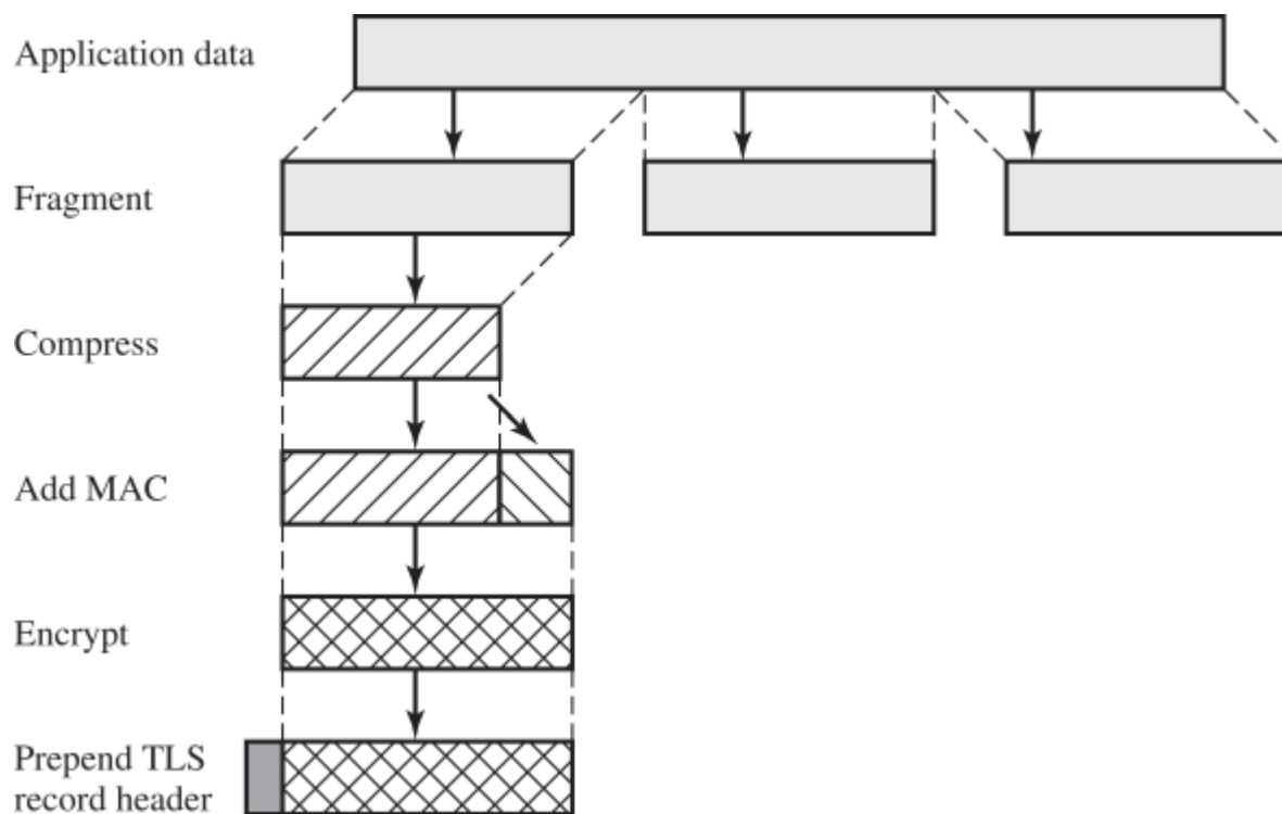
Figure 22.5 TLS Record Protocol Operation
