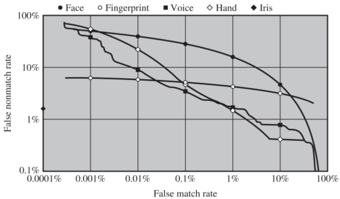
Figure 3.12 Actual Biometric Measurement Operating Characteristic Curves
