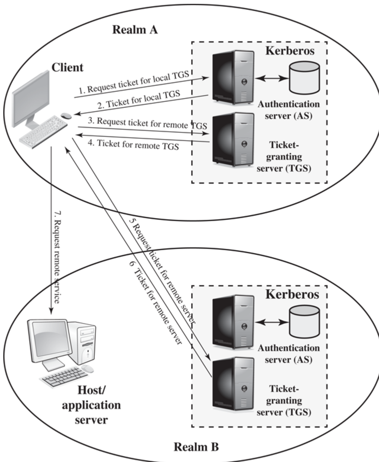
Figure 23.2 Request for Service in Another Realm
