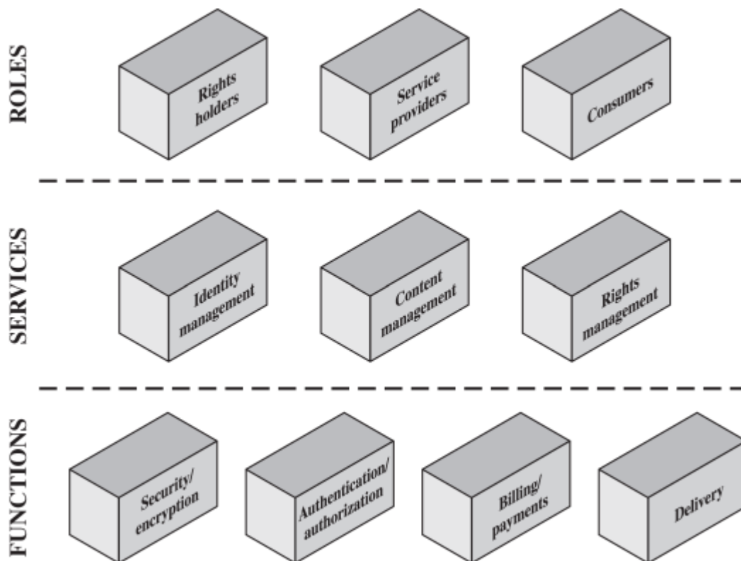
Figure 19.3 DRM System Architecture
