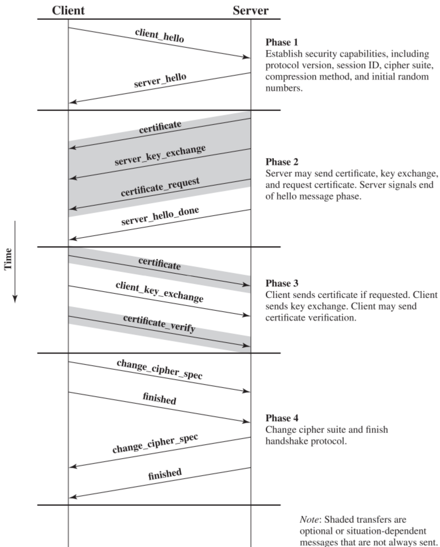
Figure 22.6 Handshake Protocol Action
