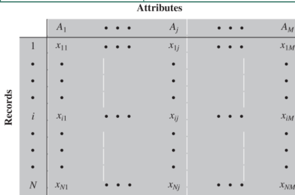
Figure 5.3 Abstract Model of a Relational Database
