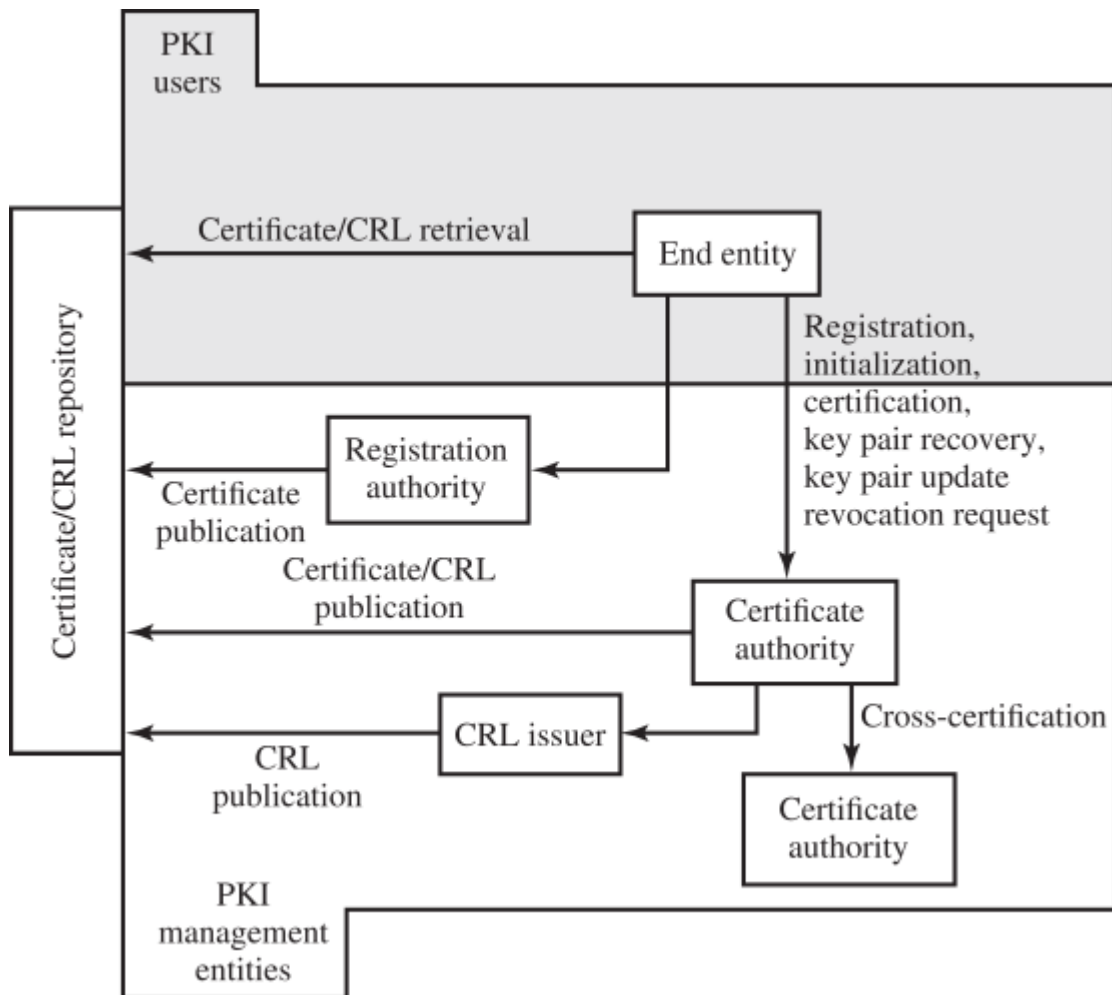
Figure 23.4 PKIX Architectural Model
