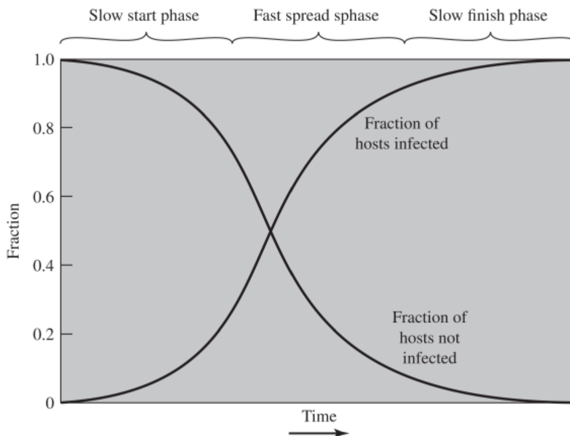
Figure 6.2 Worm Propagation Model
