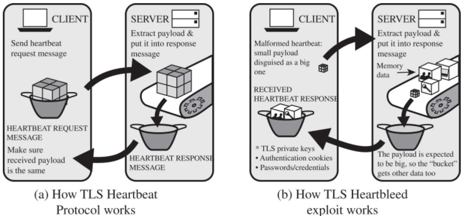
Figure 22.7 The Heartbleed Exploit
