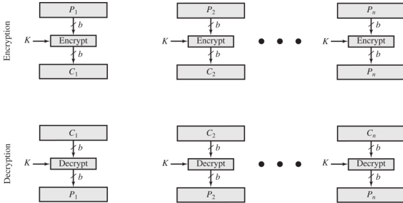
(a) Block cipher encryption (electronic codebook mode)
