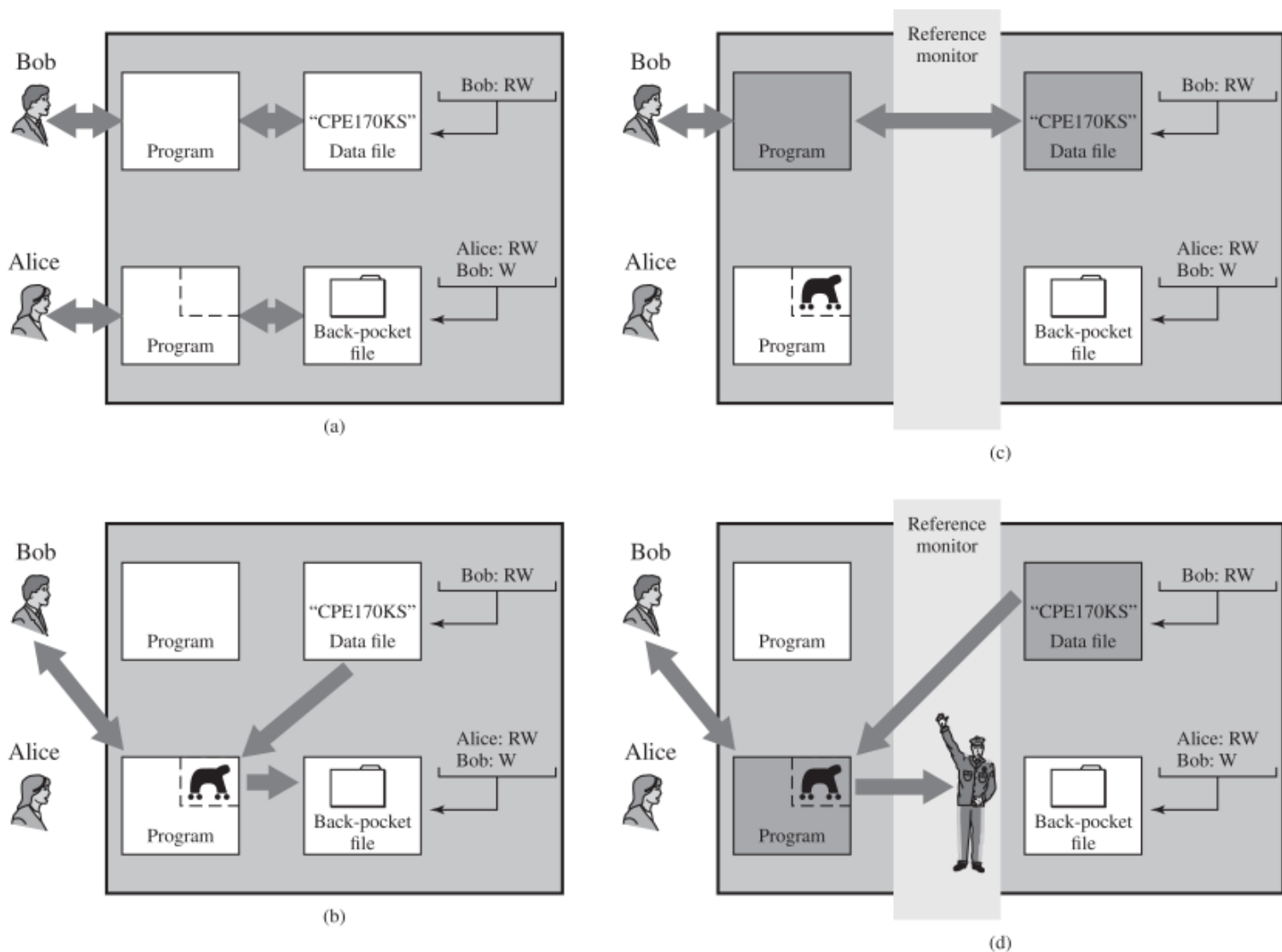
Figure 27.8 Trojan Horse and Secure Operating System
