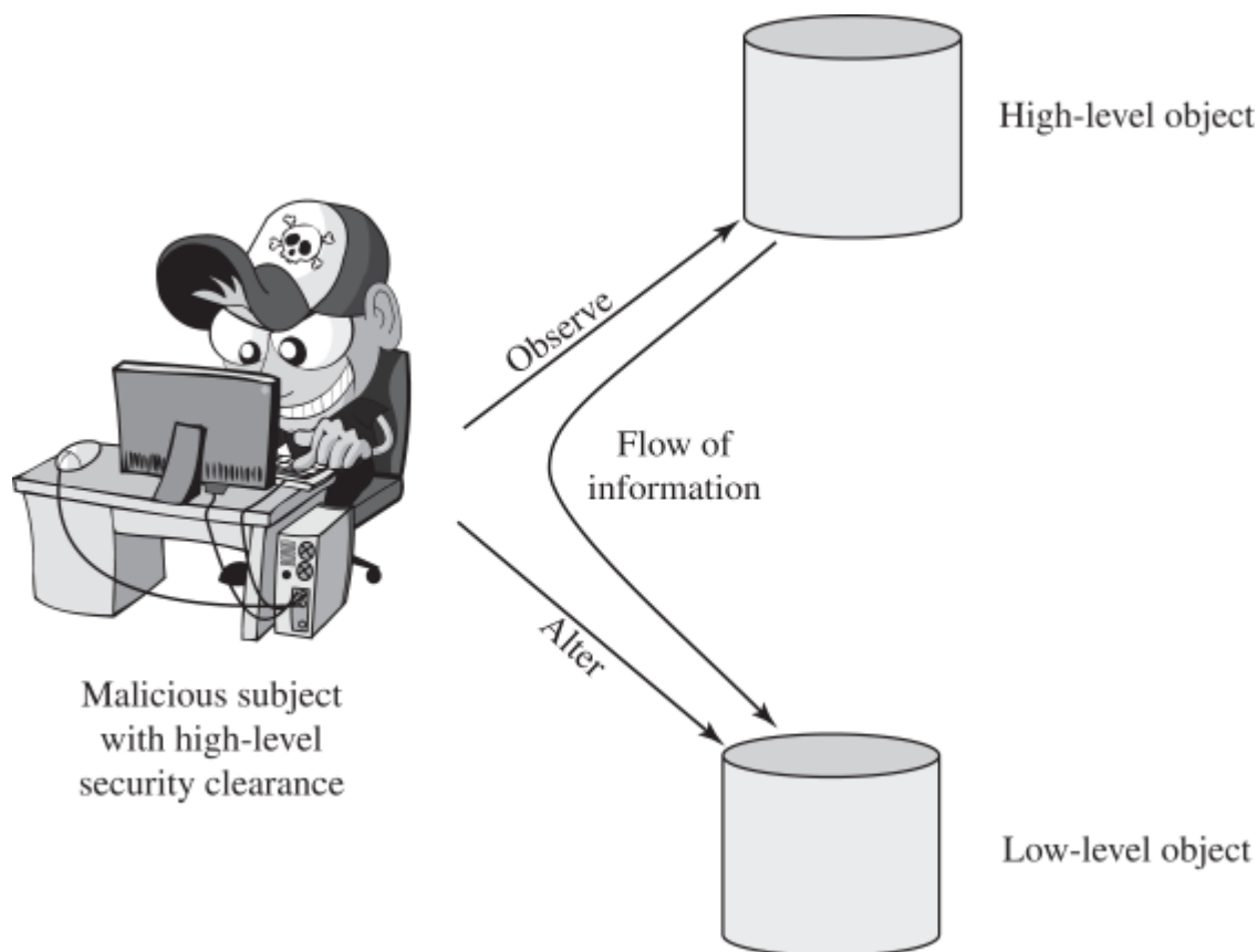
Figure 27.1 Information Flow Showing the Need for the *-Property
