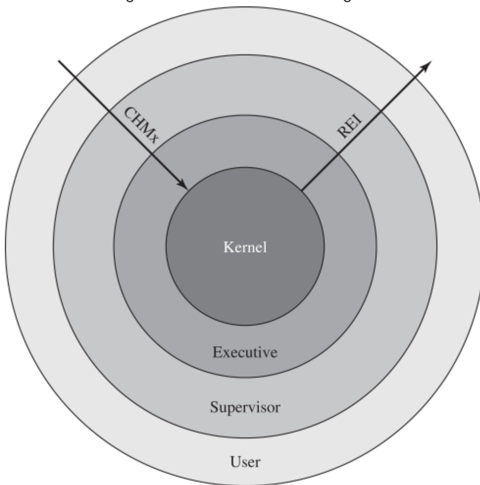
Figure 4.15 VAX/VMS Access Modes
