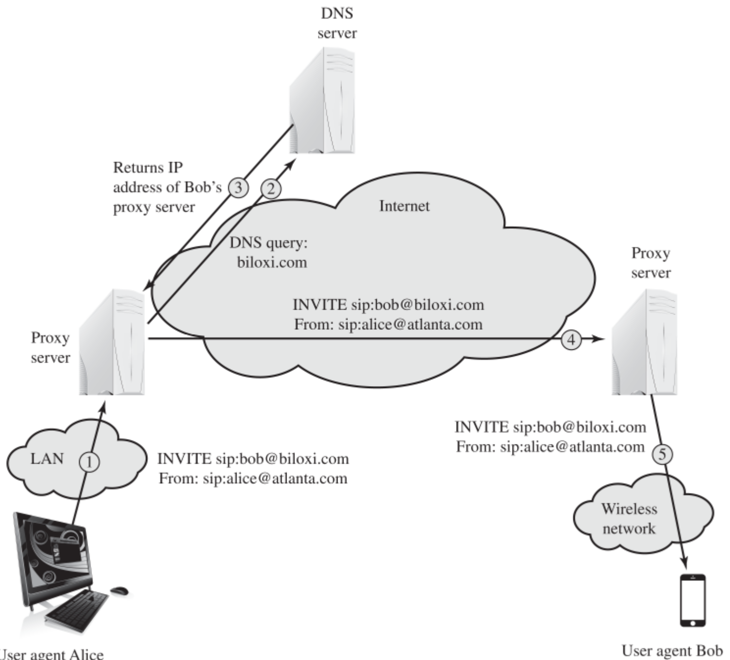
Figure 7.5 SIP INVITE Scenario
