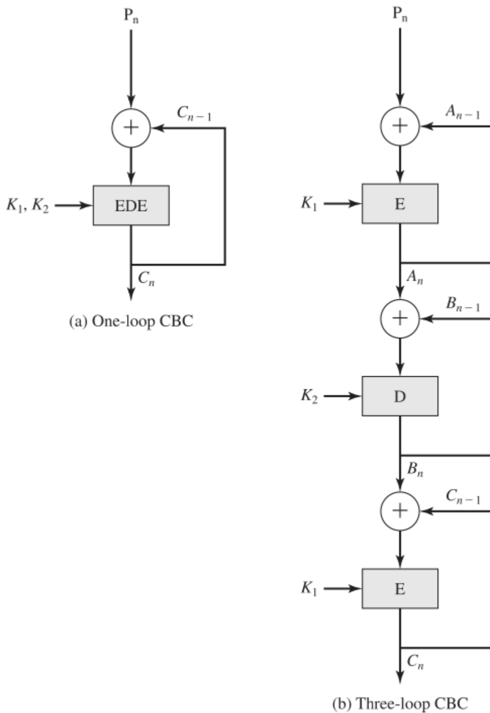
Figure 20.11 Use of Triple DES in CBC Mode
