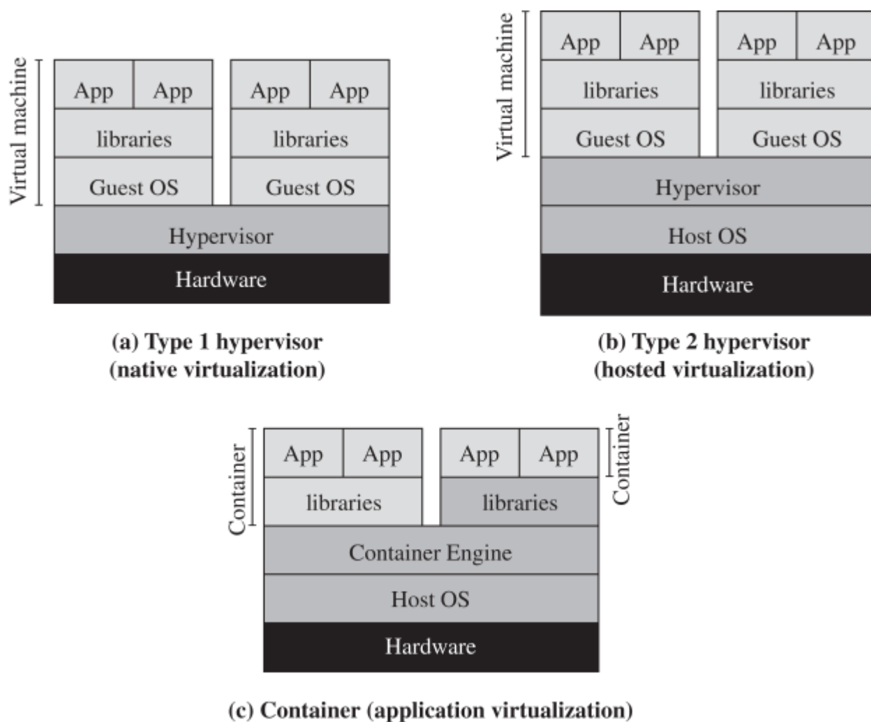
Figure 12.2 Comparison of Virtual Machines and Containers
