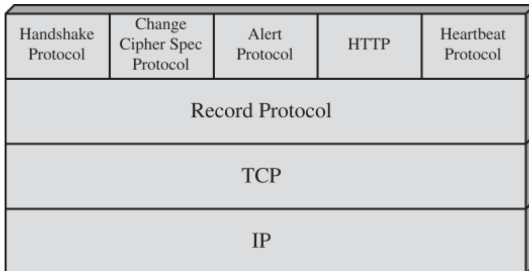
Figure 22.4 SSL/TLS Protocol Stack
