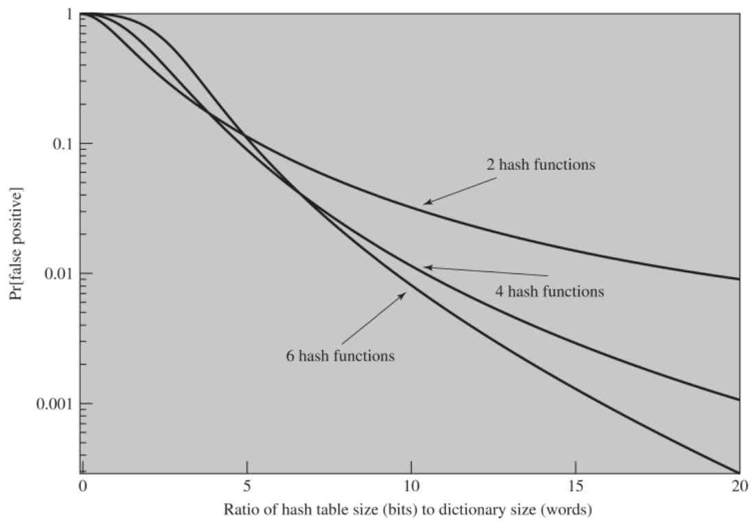
Figure 3.5 Performance of Bloom Filter
