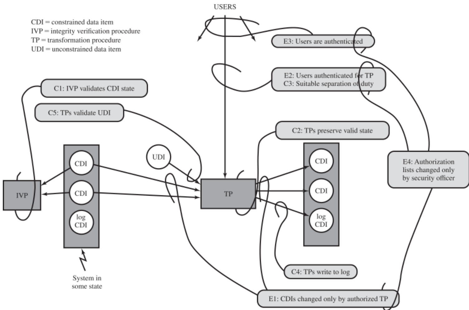
Figure 27.5 Summary of Clark–Wilson System Integrity Rules
