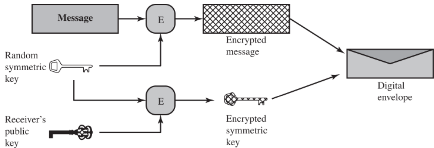
(a) Creation of a digital envelope
