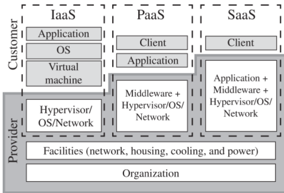
(a) Cloud computing assets
