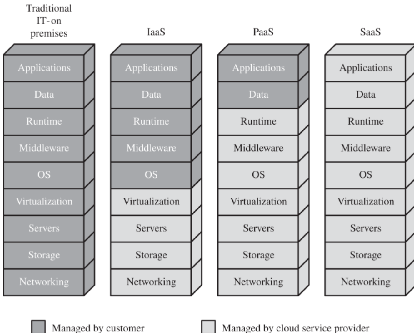
Figure 13.2 Separation of Responsibilities in Cloud Service Models
