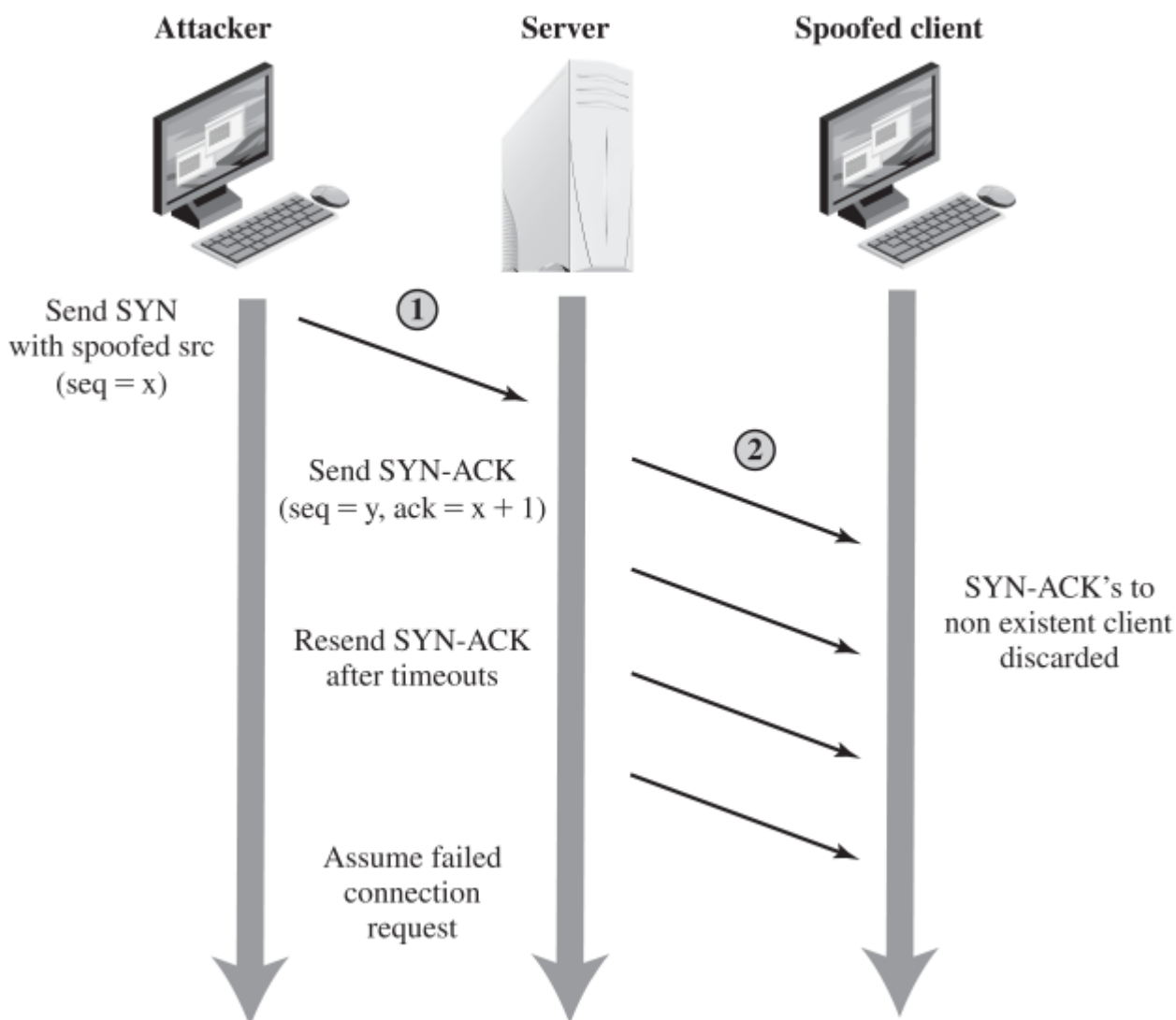
Figure 7.3 TCP SYN Spoofing Attack
