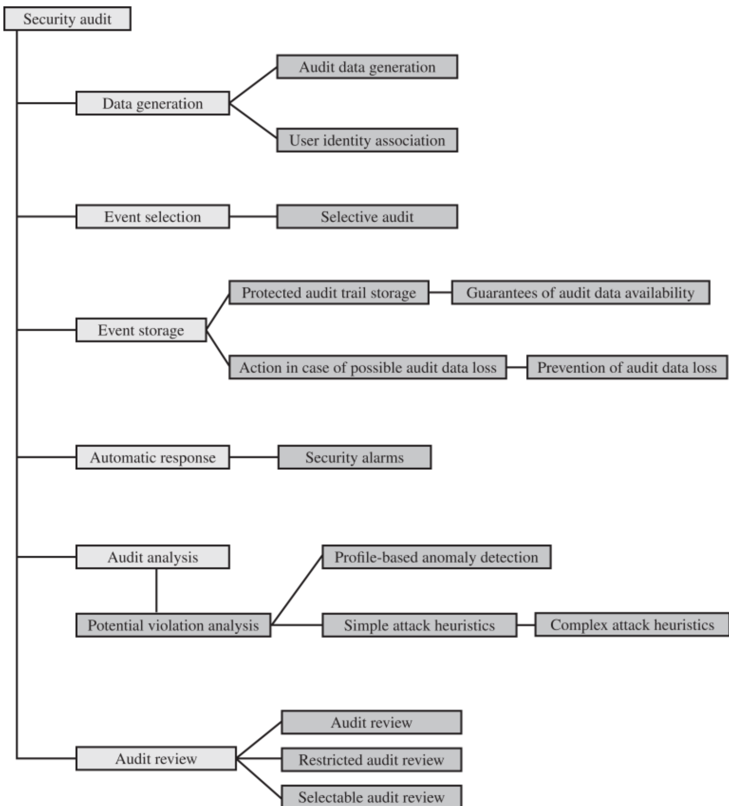
Figure 18.3 Common Criteria Security Audit Class Decomposition
