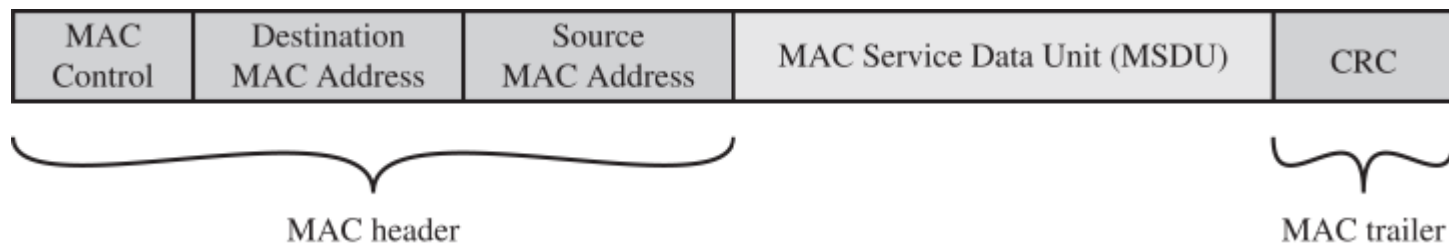
Figure 24.4 General IEEE 802 MPDU Format
