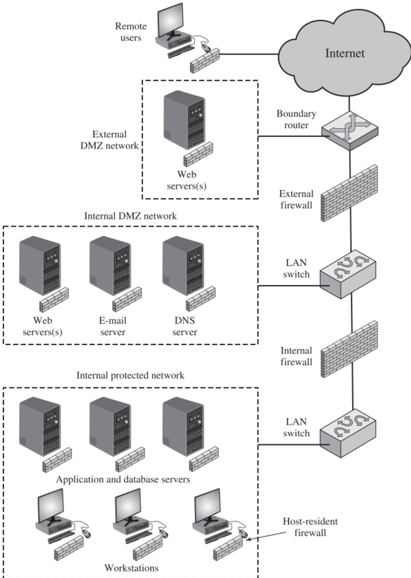
Figure 9.4 Example Distributed Firewall Configuration
