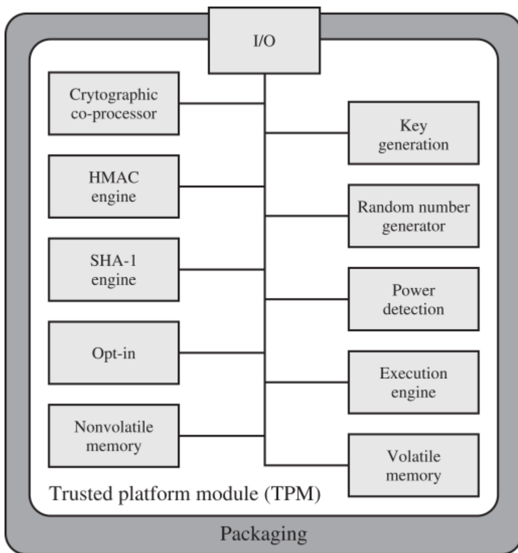
Figure 27.11 TPM Component Architecture
