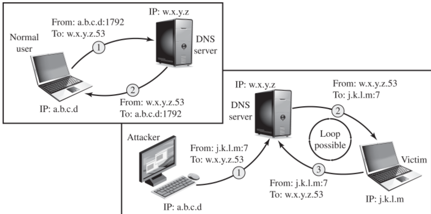
Figure 7.6 DNS Reflection Attack
