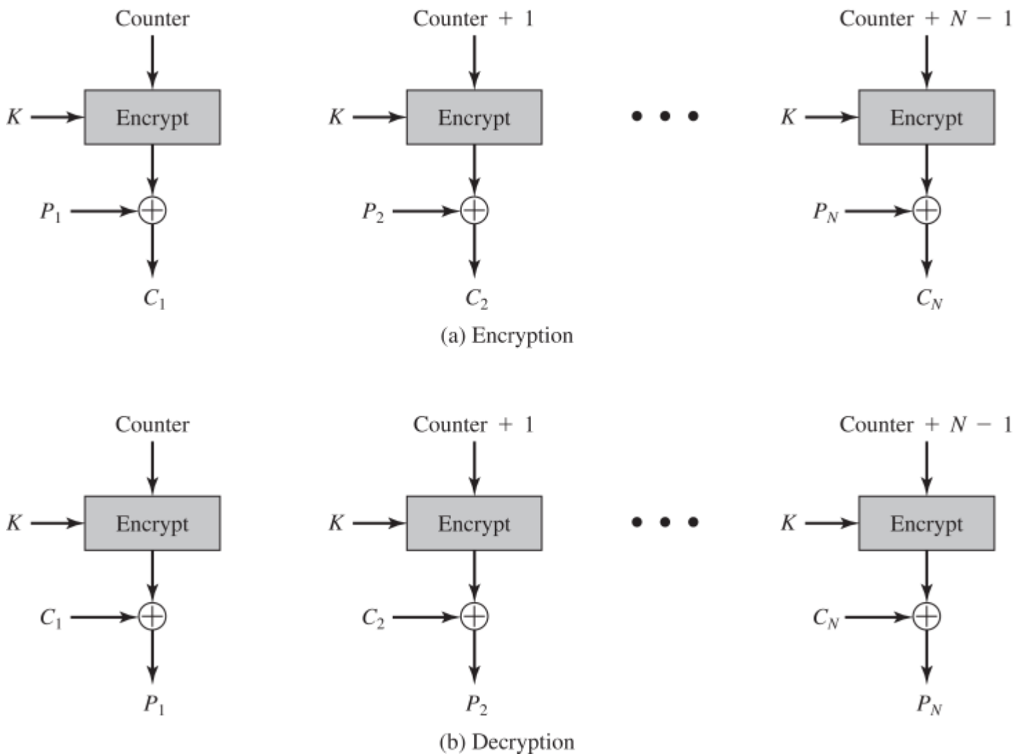
Figure 20.9 Counter (CTR) Mode
