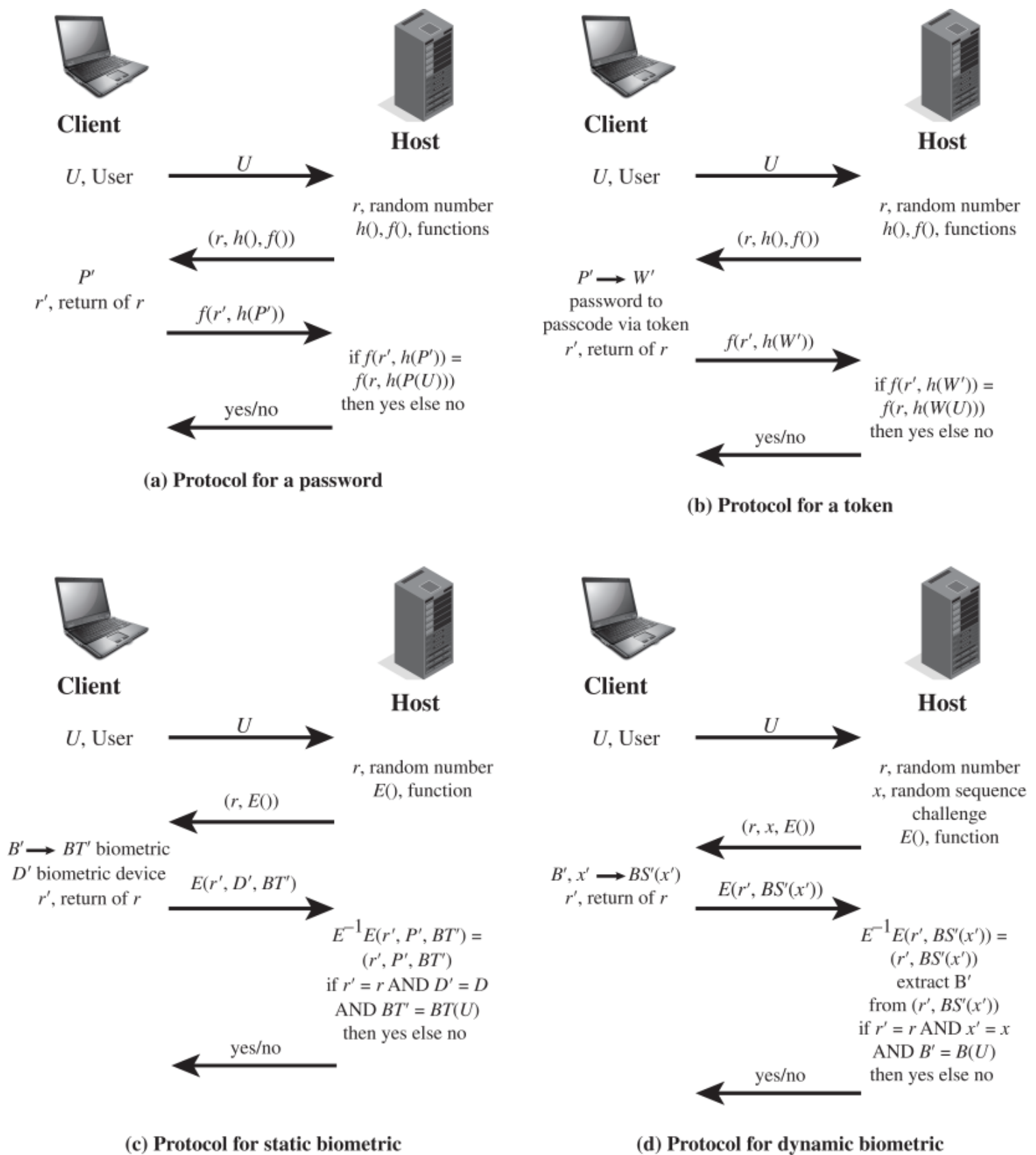
Figure 3.13 Basic Challenge-Response Protocols for Remote User Authentication
