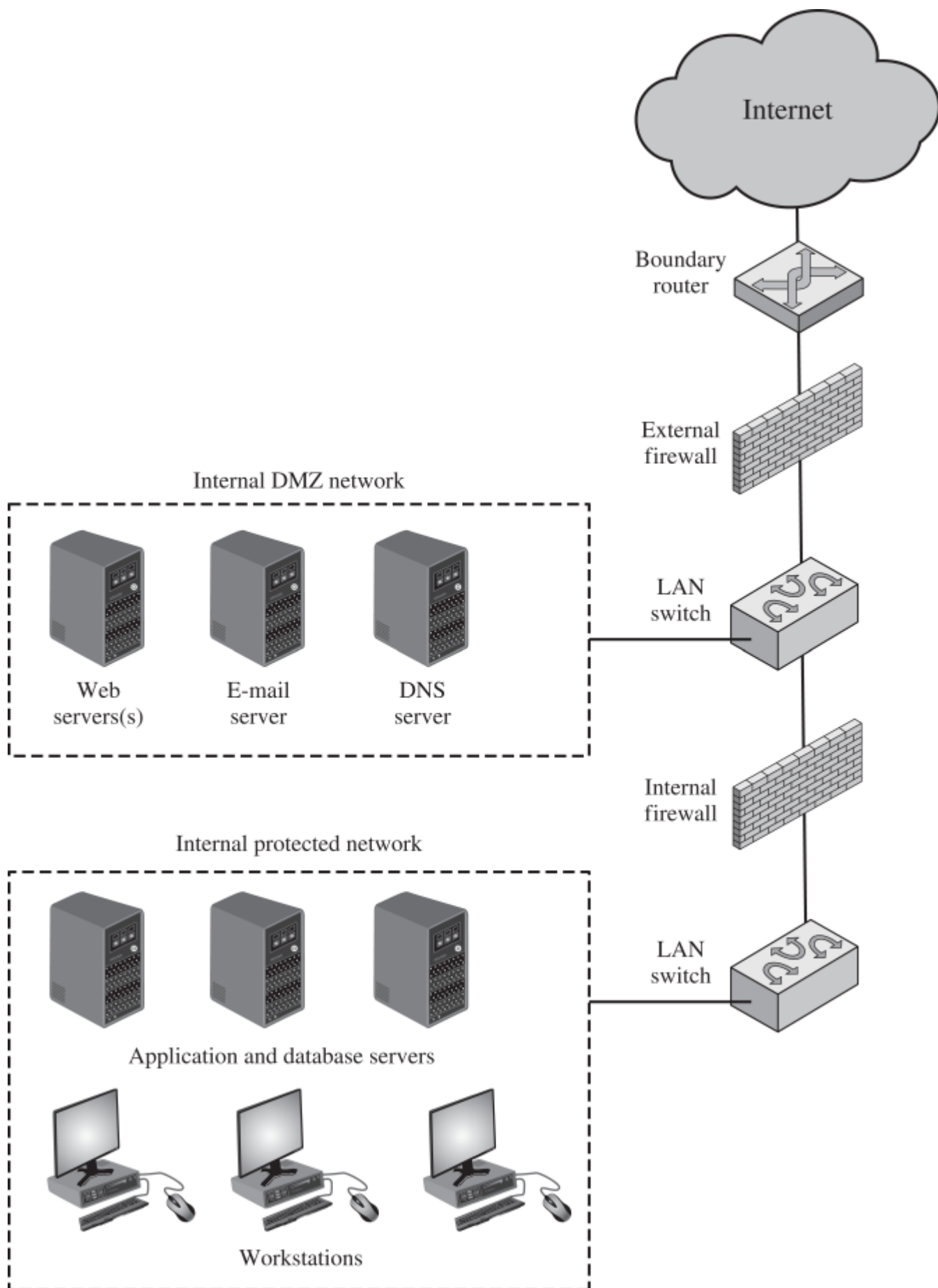
Figure 9.2 Example Firewall Configuration
