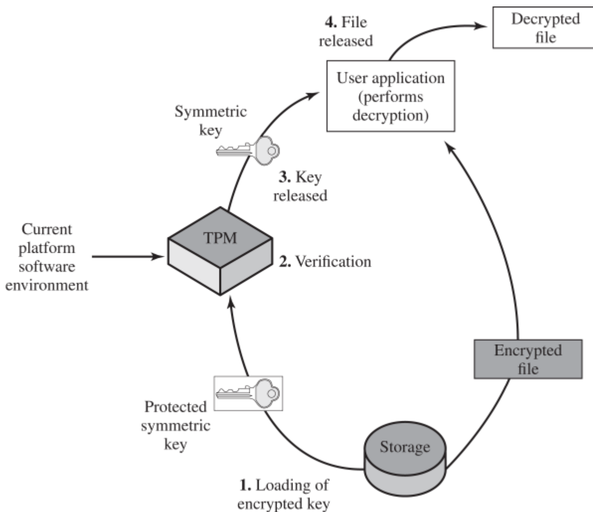
Figure 27.12 Decrypting a File Using a Protected Key
