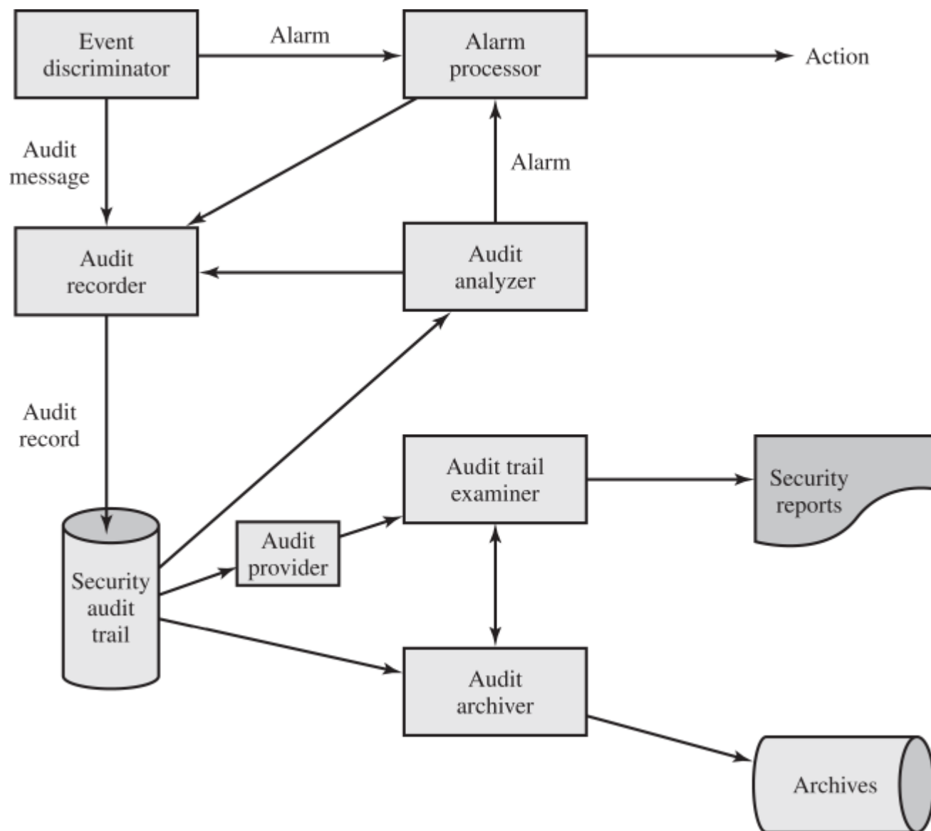
Figure 18.1 Security Audit and Alarms Model (X.816)
