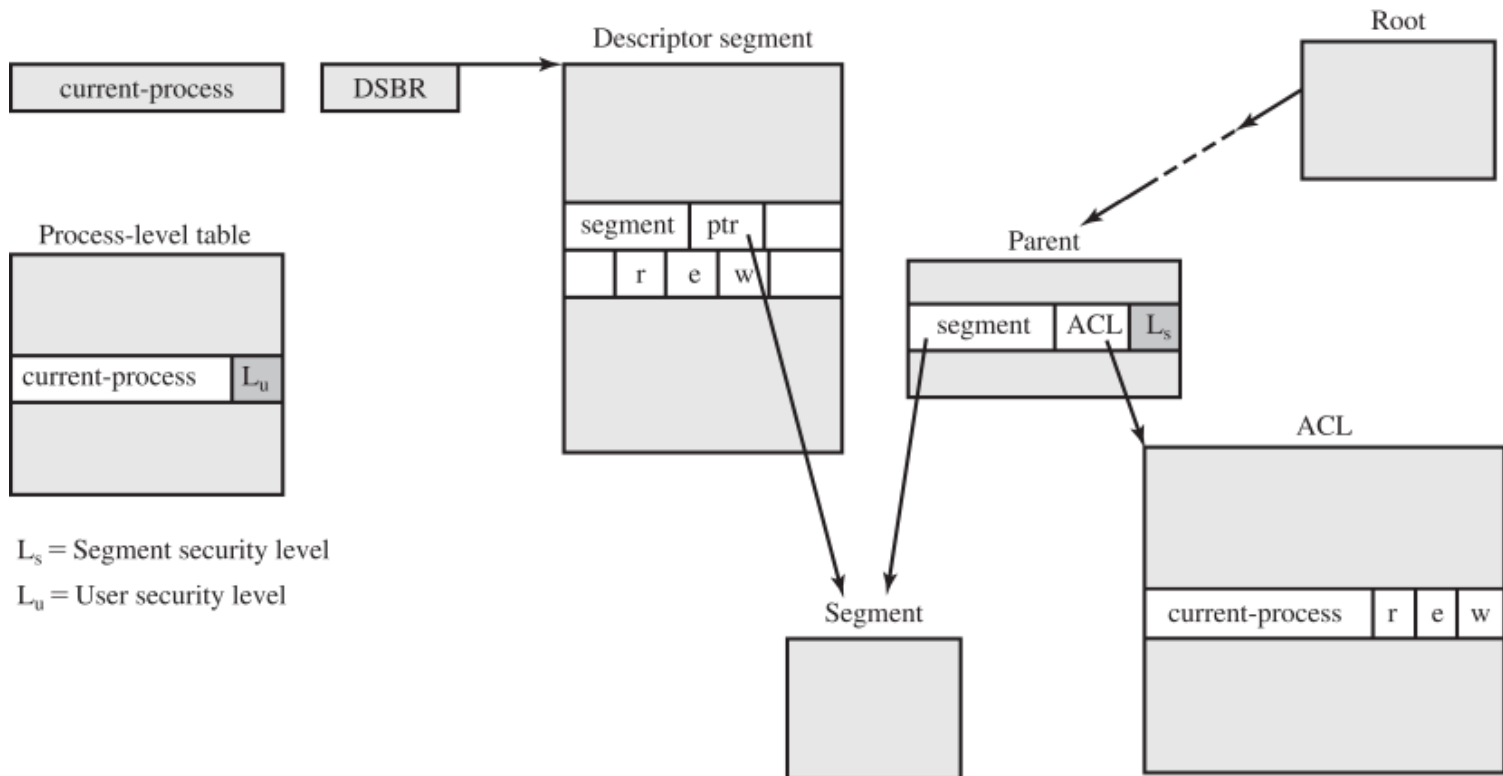
Figure 27.3 Multics Data Structures for MLS
