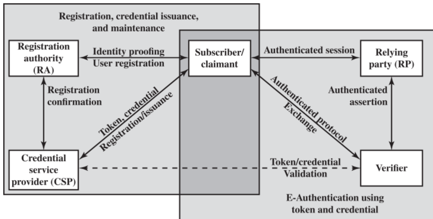
Figure 3.1 The NIST SP 800-63-3 E-Authentication Architectural Model
