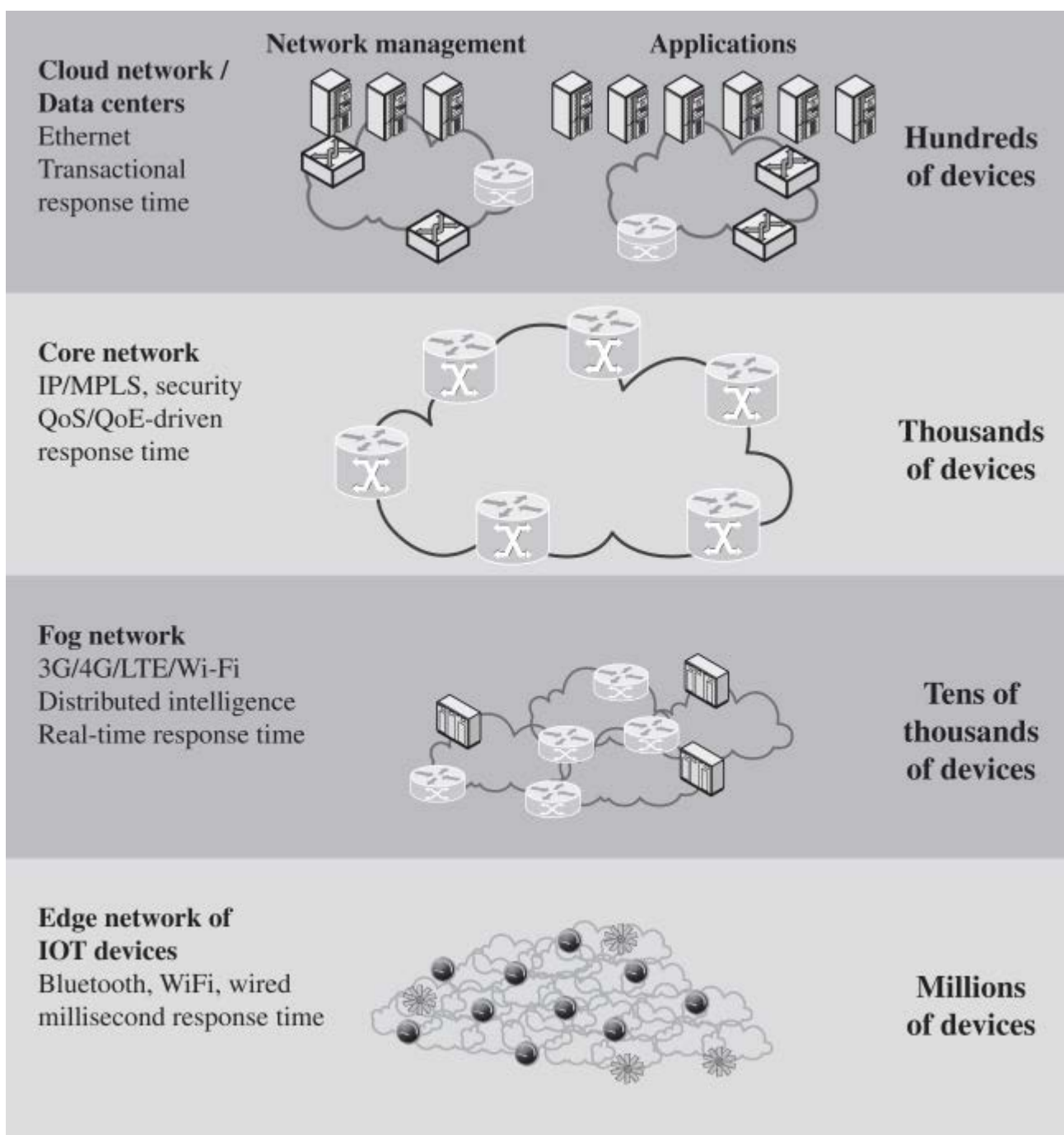
Figure 13.9 The IoT and Cloud Context
