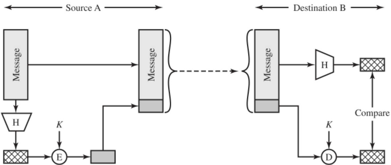
(a) Using symmetric encryption
