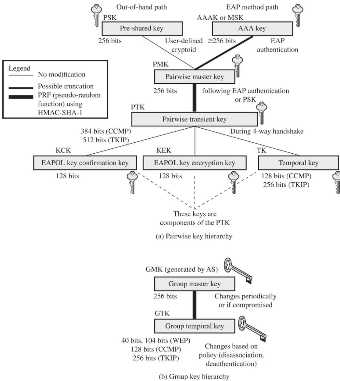
Figure 24.10 IEEE 802.11i Key Hierarchies
