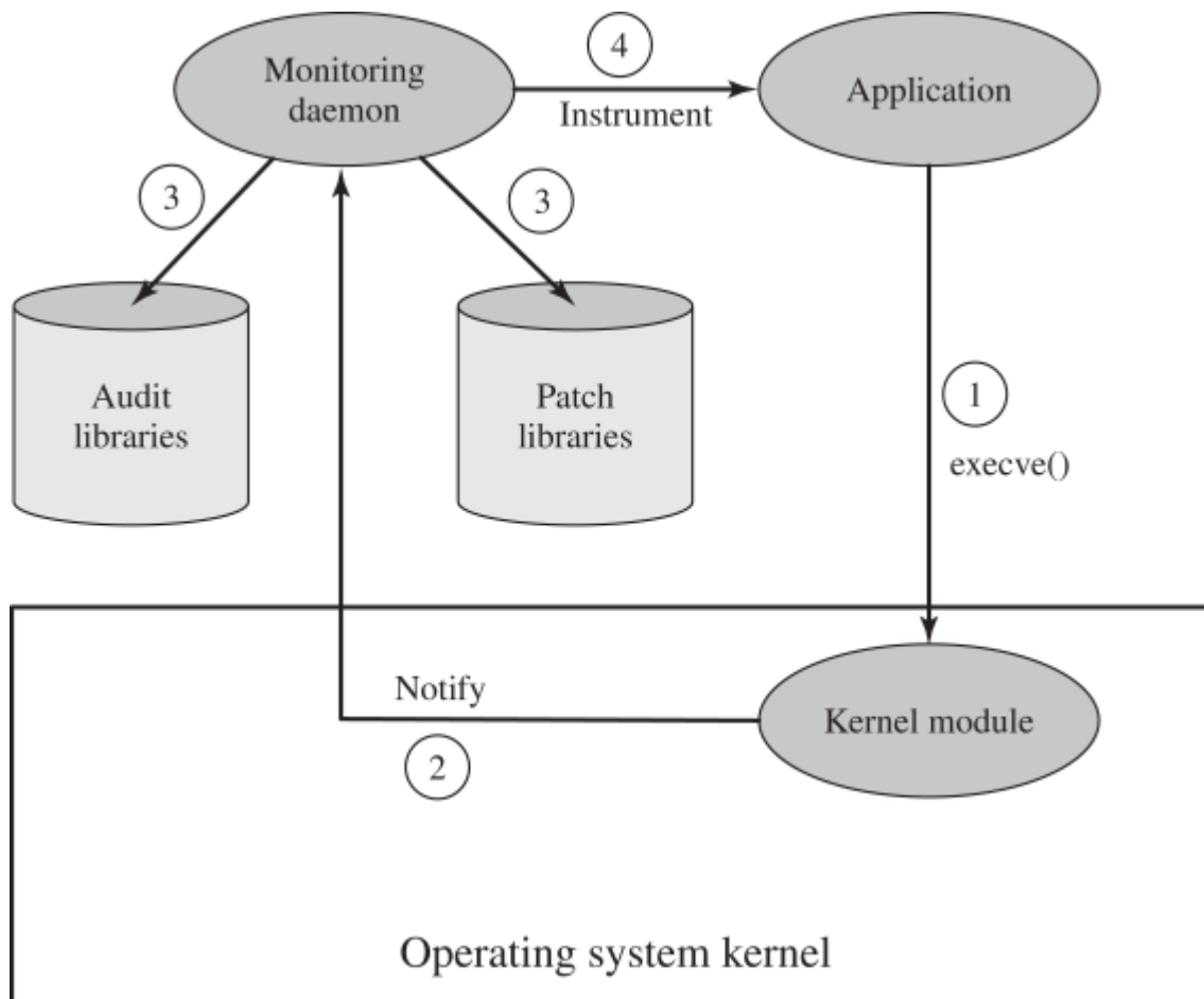
Figure 18.9 Run-Time Environment for Application Auditing
