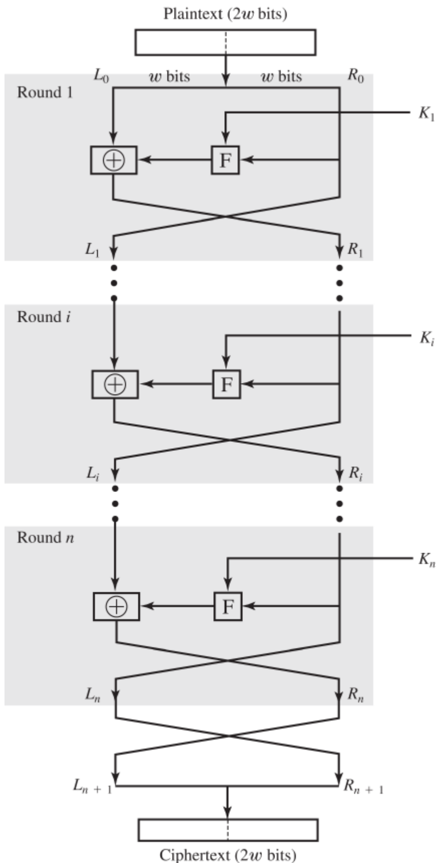
Figure 20.1 Classical Feistel Network
