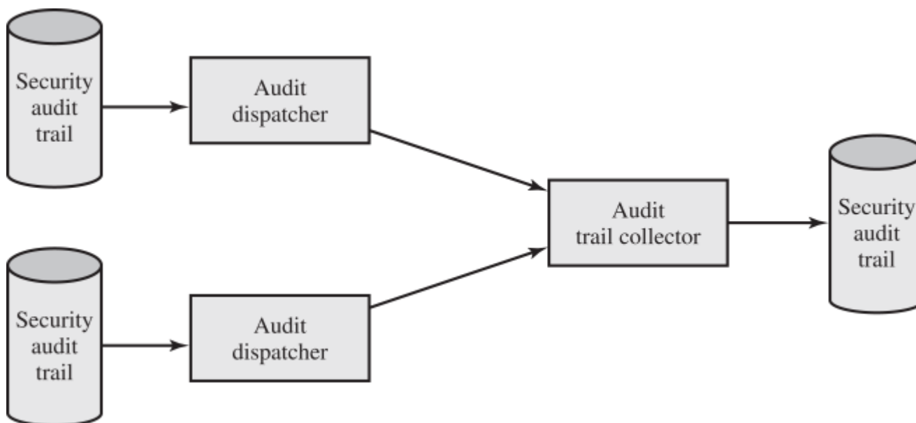
Figure 18.2 Distributed Audit Trail Model (X.816)
