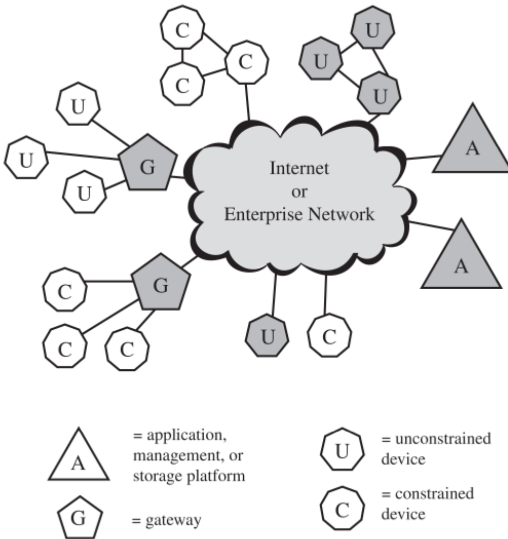
Figure 13.10 IoT Security: Elements of Interest
