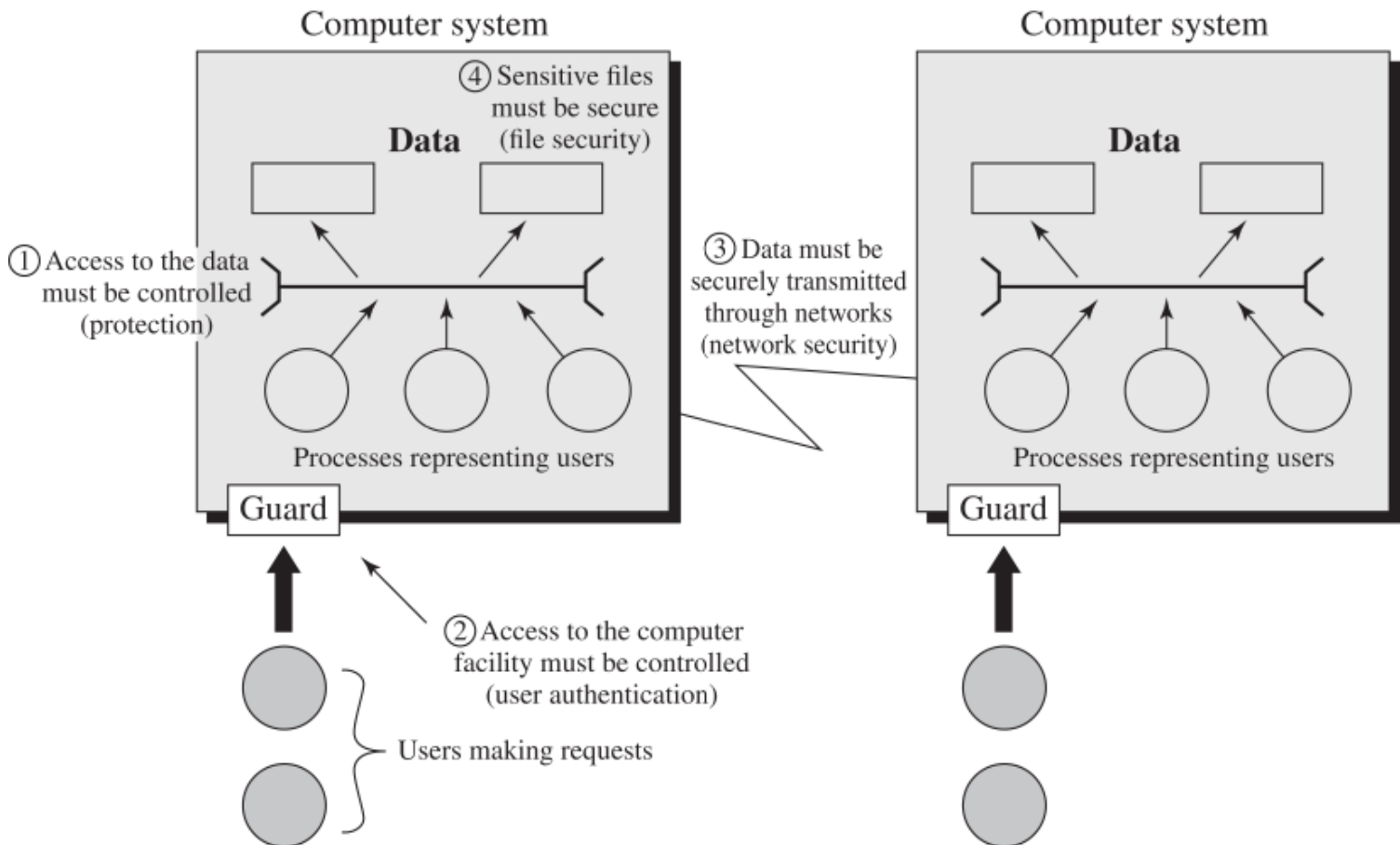
Figure 1.3 Scope of Computer Security
