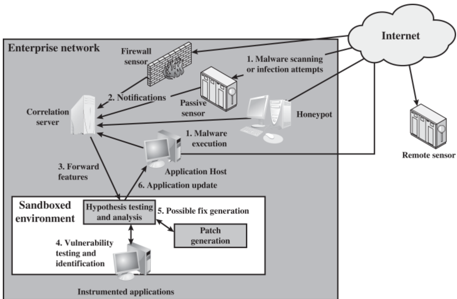
Figure 9.5 Placement of Malware Monitors
