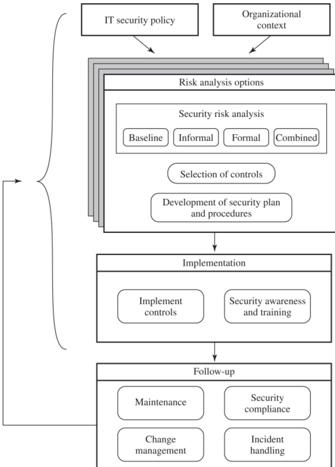
Figure 14.1 Overview of IT Security Management
