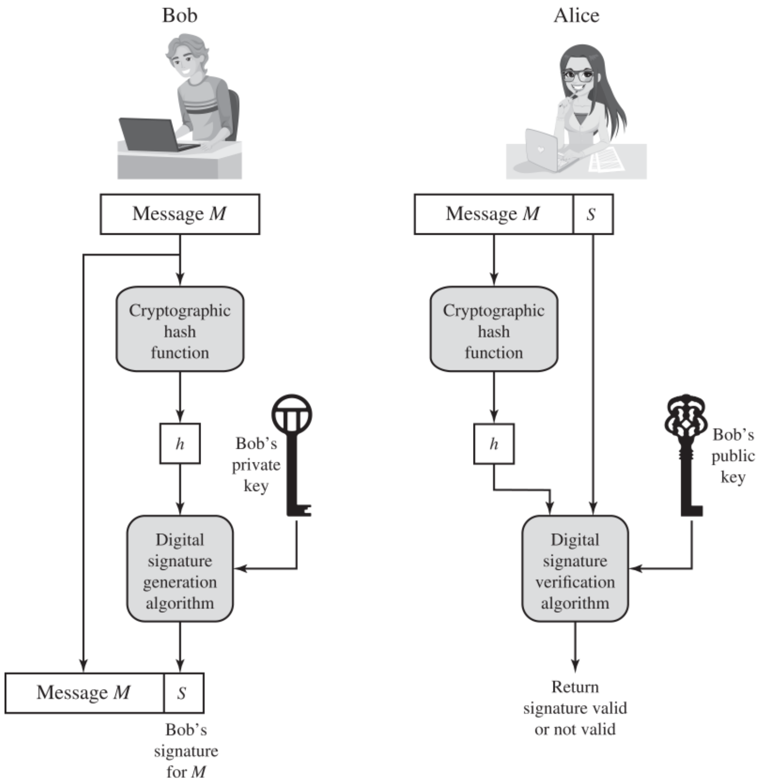
(a) Bob signs a message
