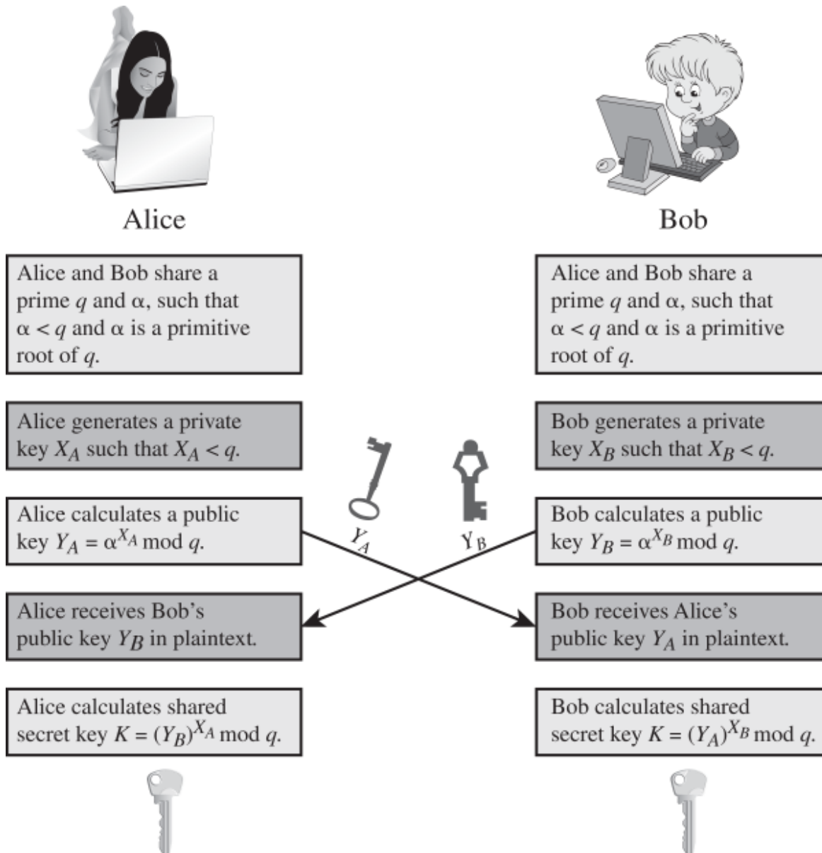
Figure 21.10 Diffie-Hellman Key Exchange
