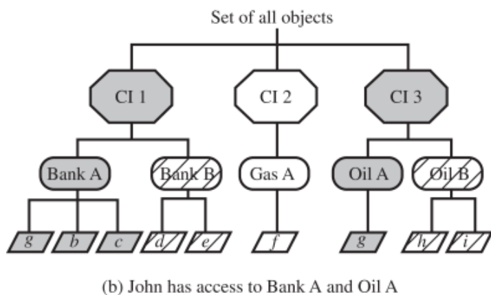
Figure 27.6 Potential Flow of Information between Two CIs
