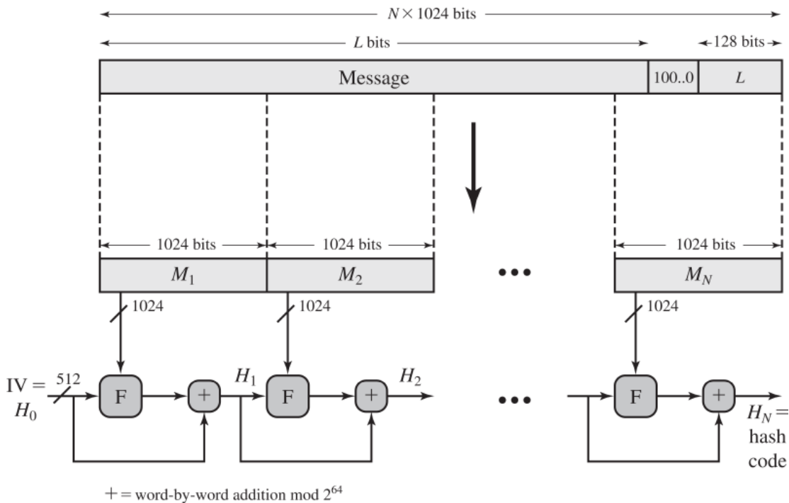
Figure 21.2 Message Digest Generation Using SHA-512
