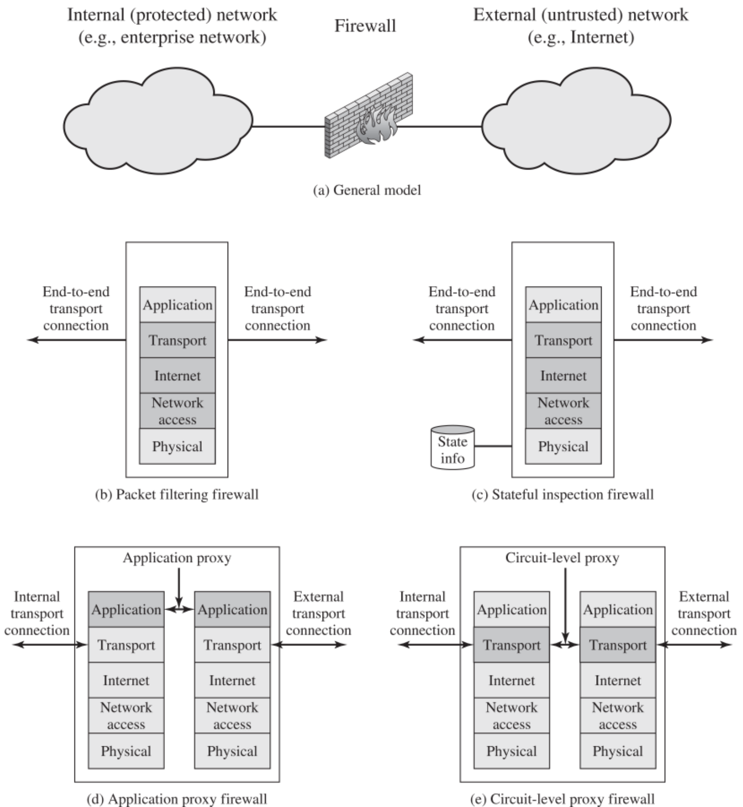
Figure 9.1 Types of Firewalls
