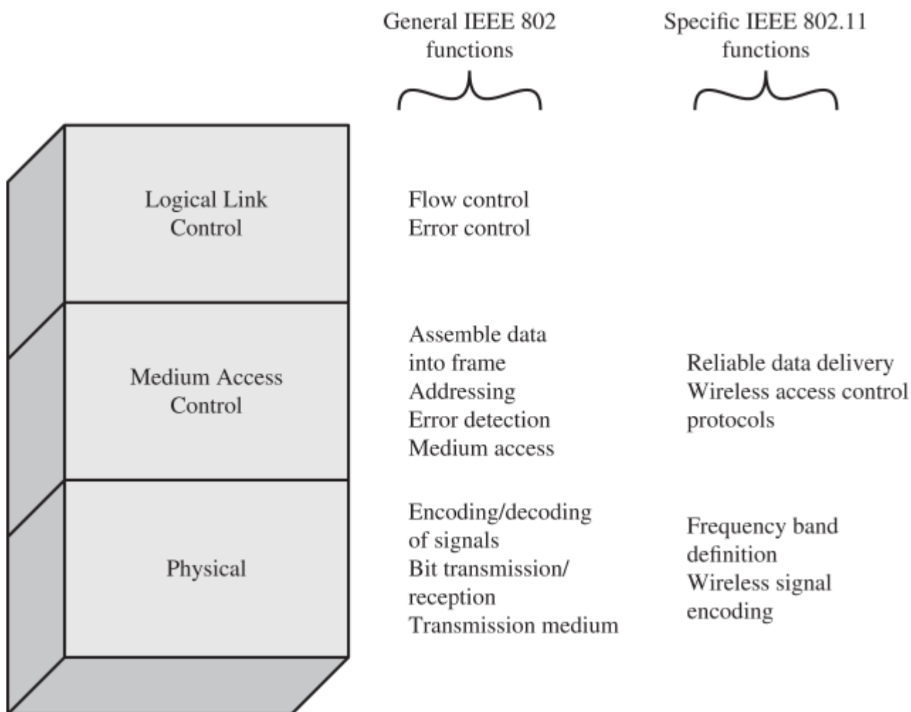
Figure 24.3 IEEE 802.11 Protocol Stack
