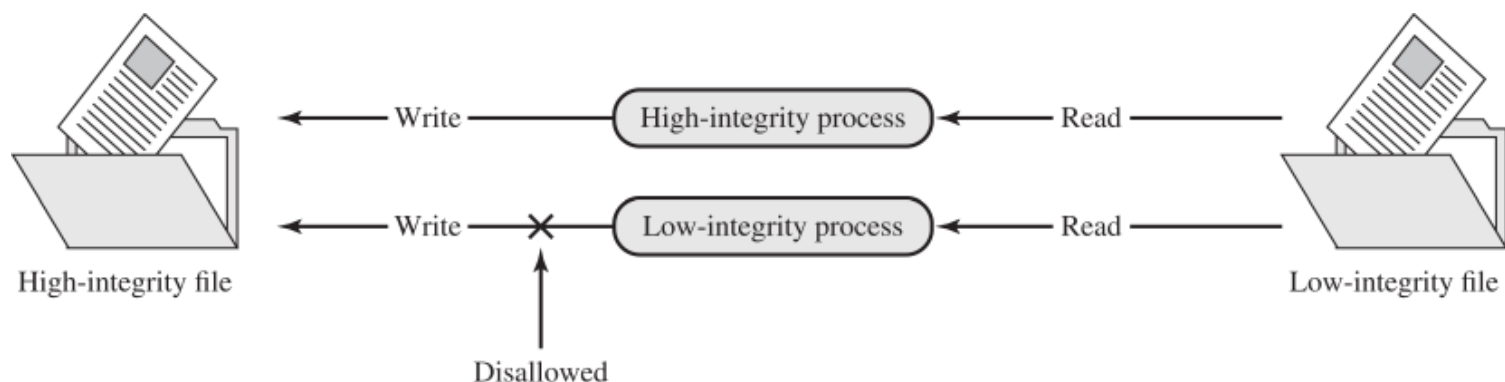
Figure 27.4 Contamination with Simple Integrity Controls
