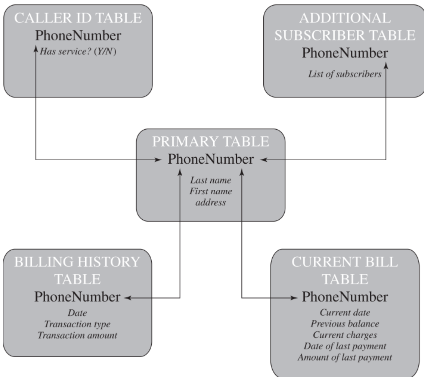
Figure 5.2 Example Relational Database Model
