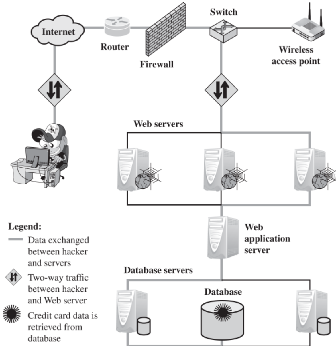
Figure 5.5 Typical SQL Injection Attack
