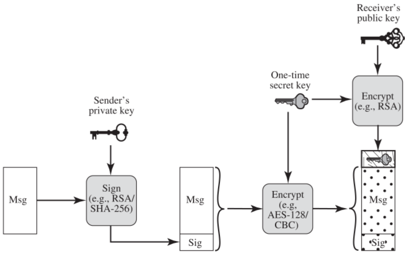
(a) Sender signs, and then encrypts message
