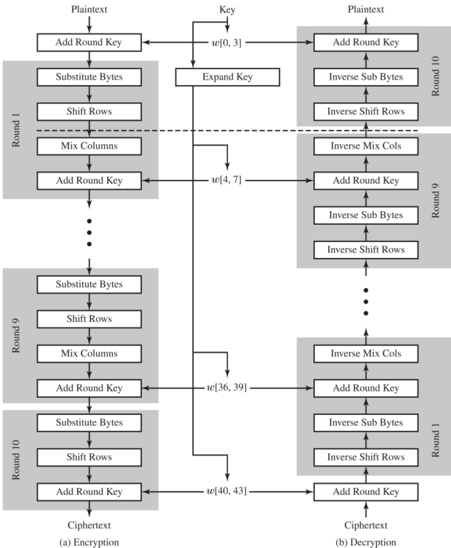
Figure 20.3 AES Encryption and Decryption
