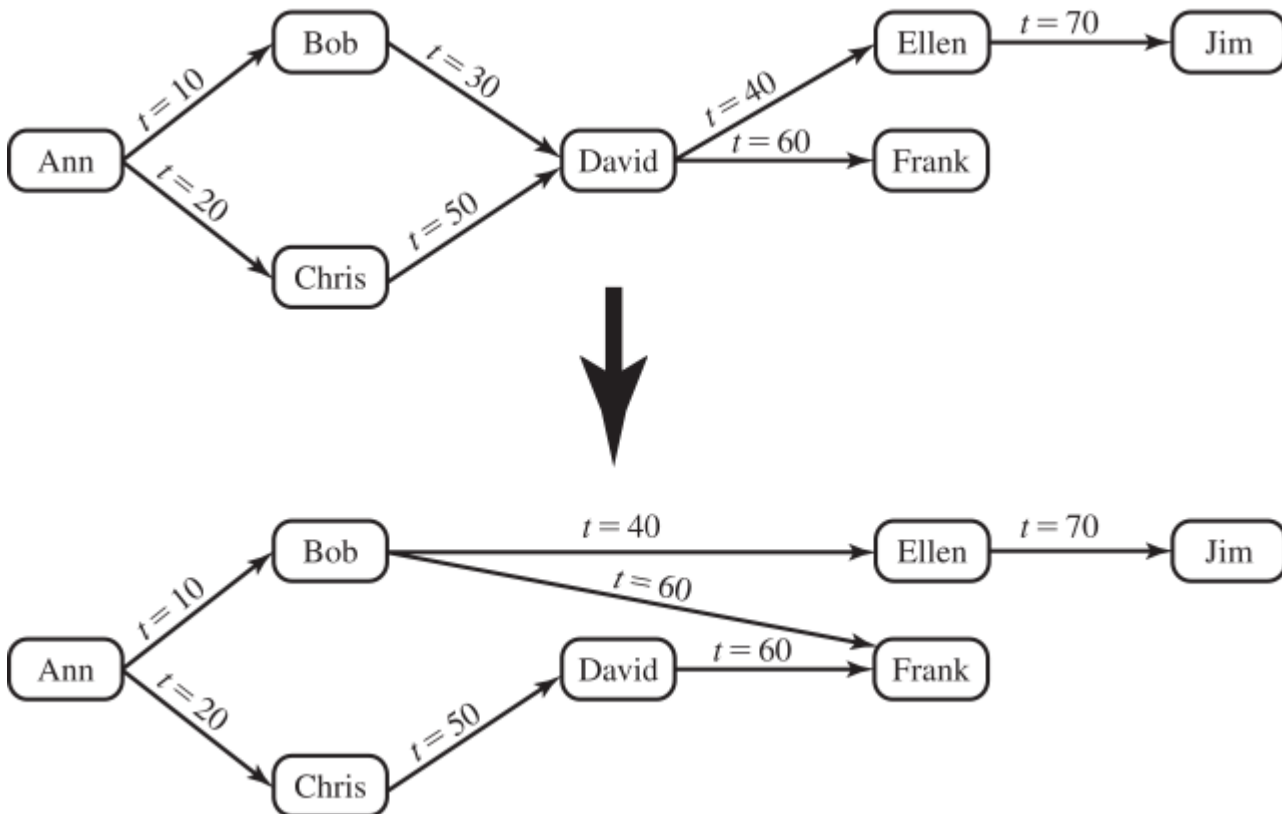
Figure 5.16 Bob Revokes Privilege from David, Second Version
