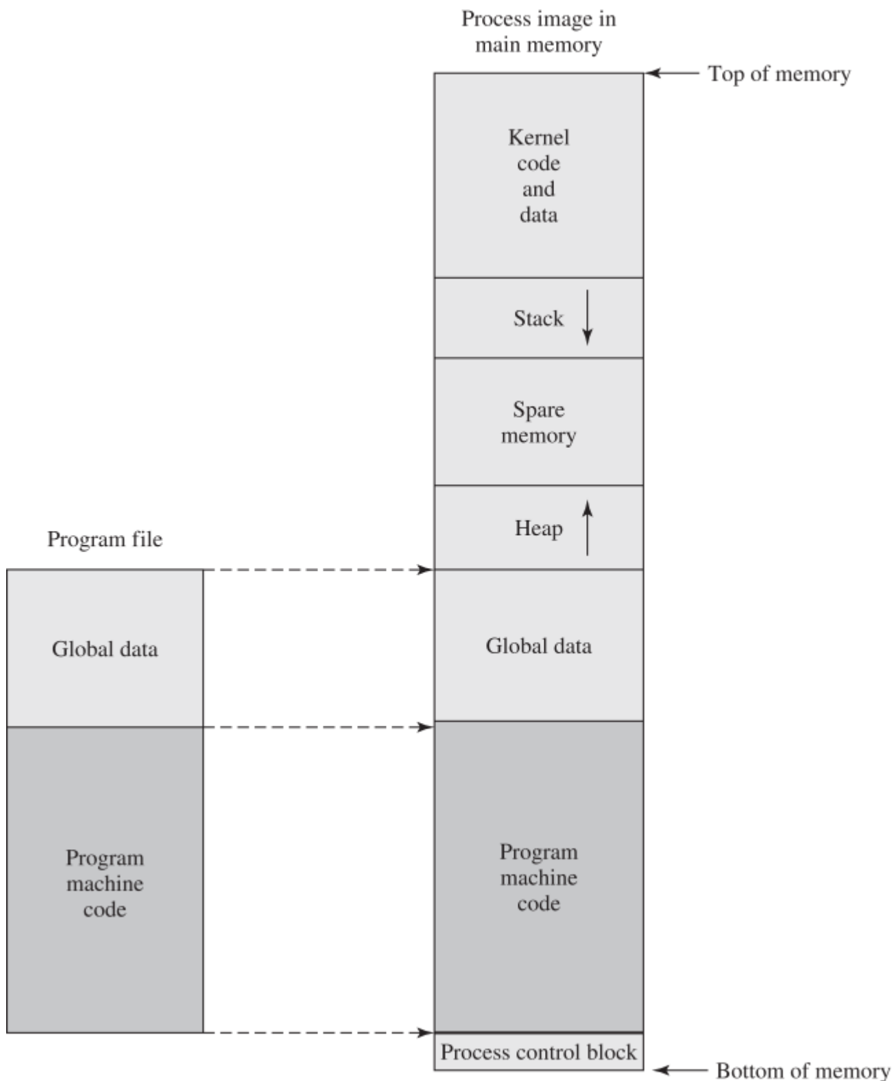
Figure 10.4 Program Loading into Process Memory
