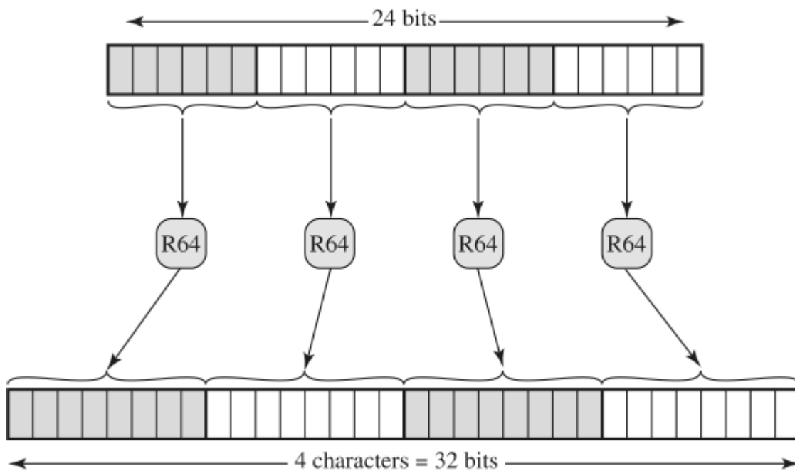
Figure G.1 Printable Encoding of Binary Data into Radix-64 Format
