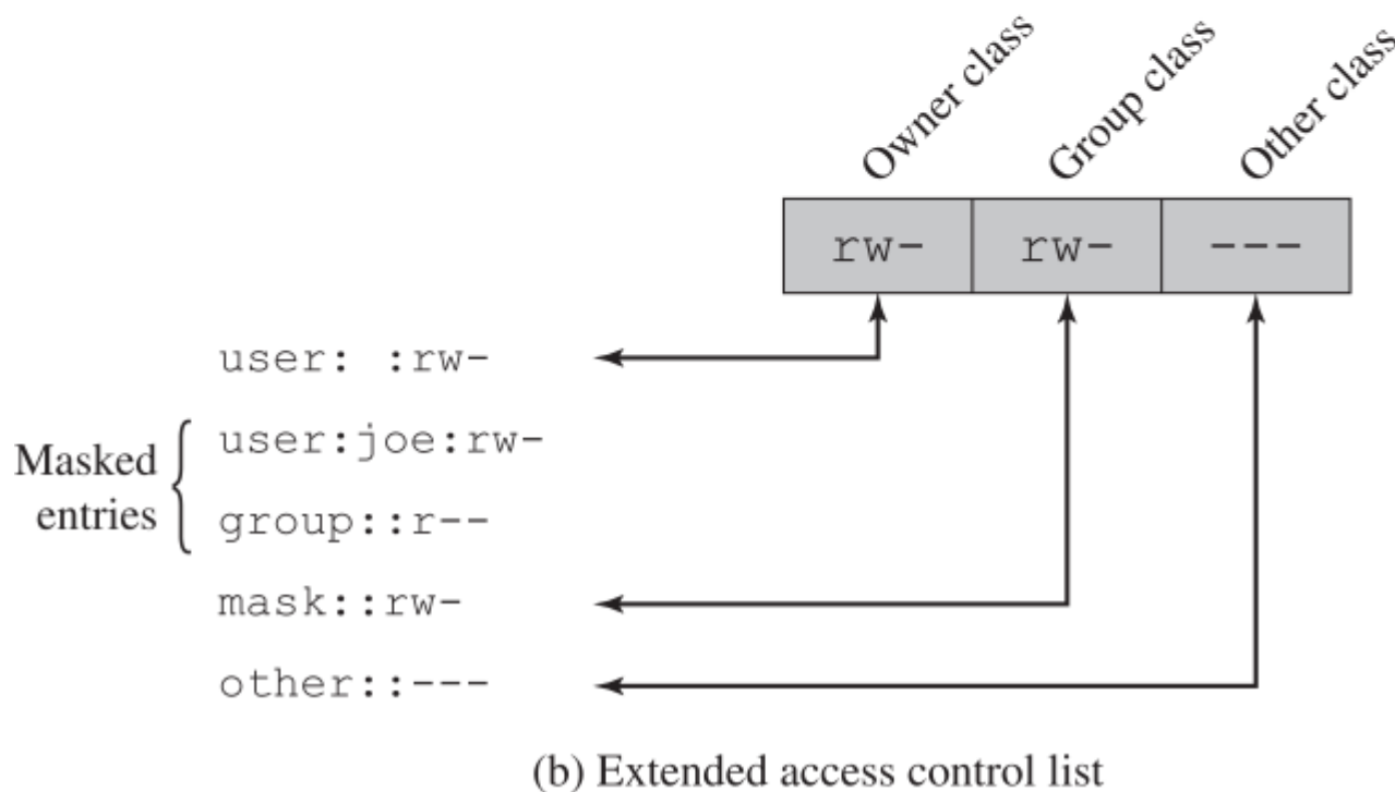
Figure 4.5 UNIX File Access Control
