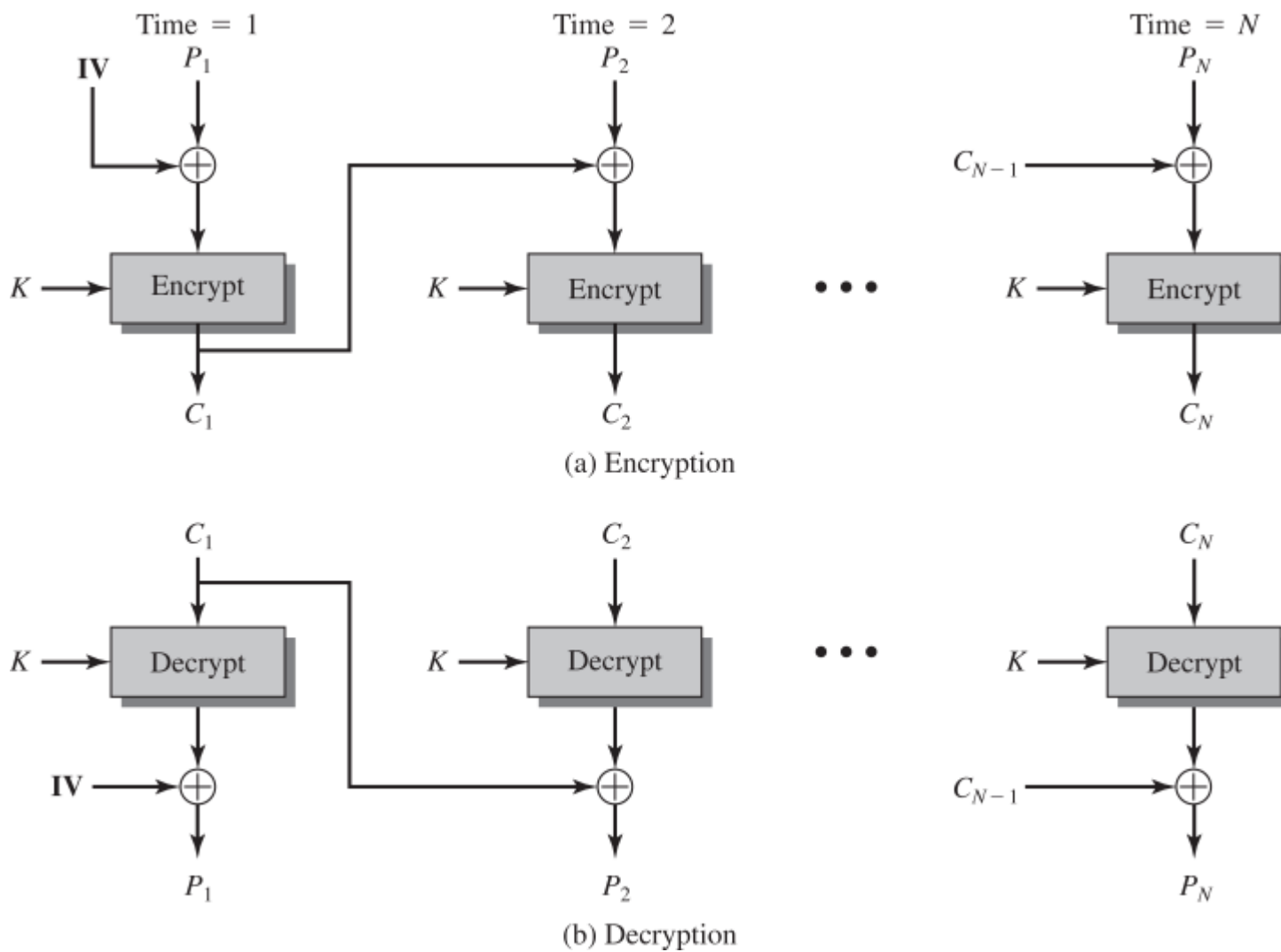
Figure 20.7 Cipher Block Chaining (CBC) Mode
