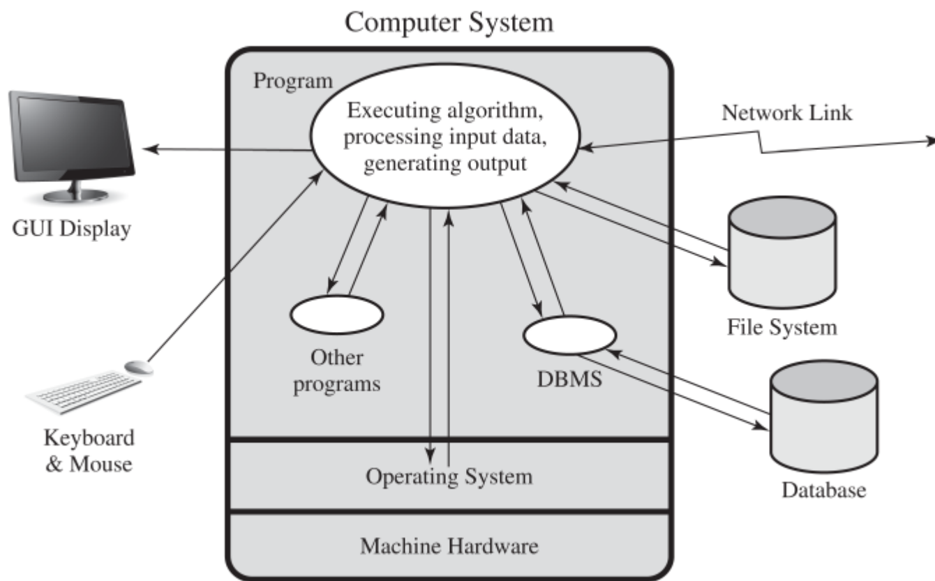
Figure 11.1 Abstract View of Program
