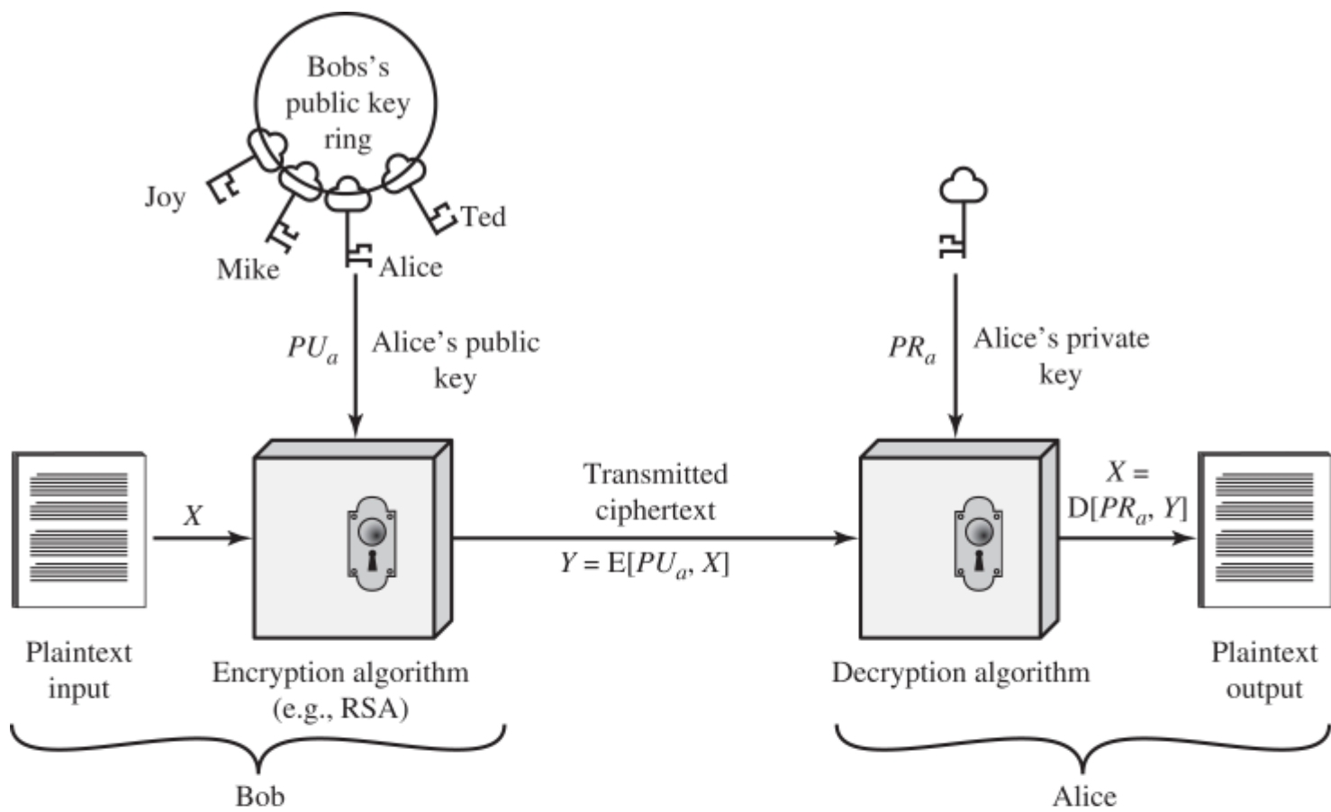
(a) Encryption with public key
