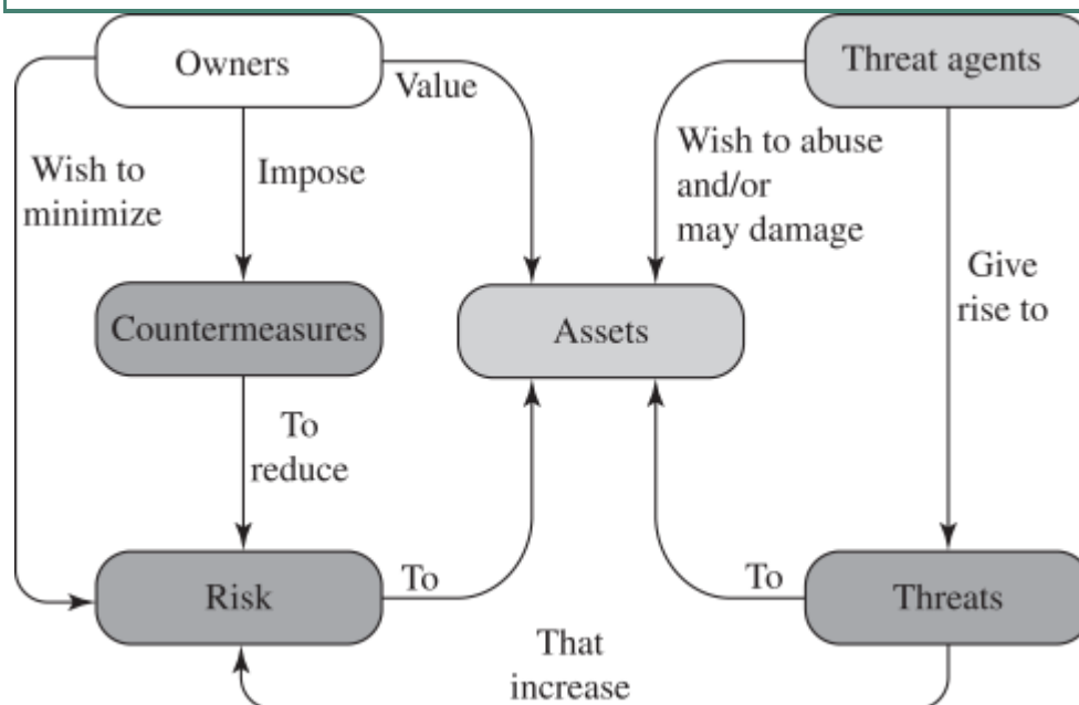
Figure 1.2 Security Concepts and Relationships
