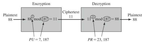
Figure 21.8 Example of RSA Algorithm
