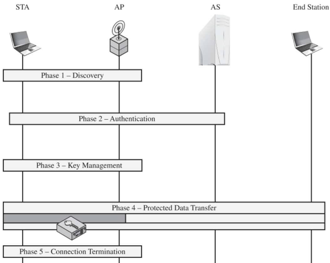
Figure 24.7 IEEE 802.11i Phases of Operation
