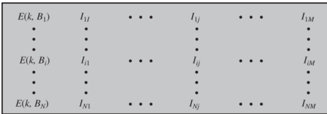
Figure 5.10 Encryption Scheme for Database of Figure 5.3
