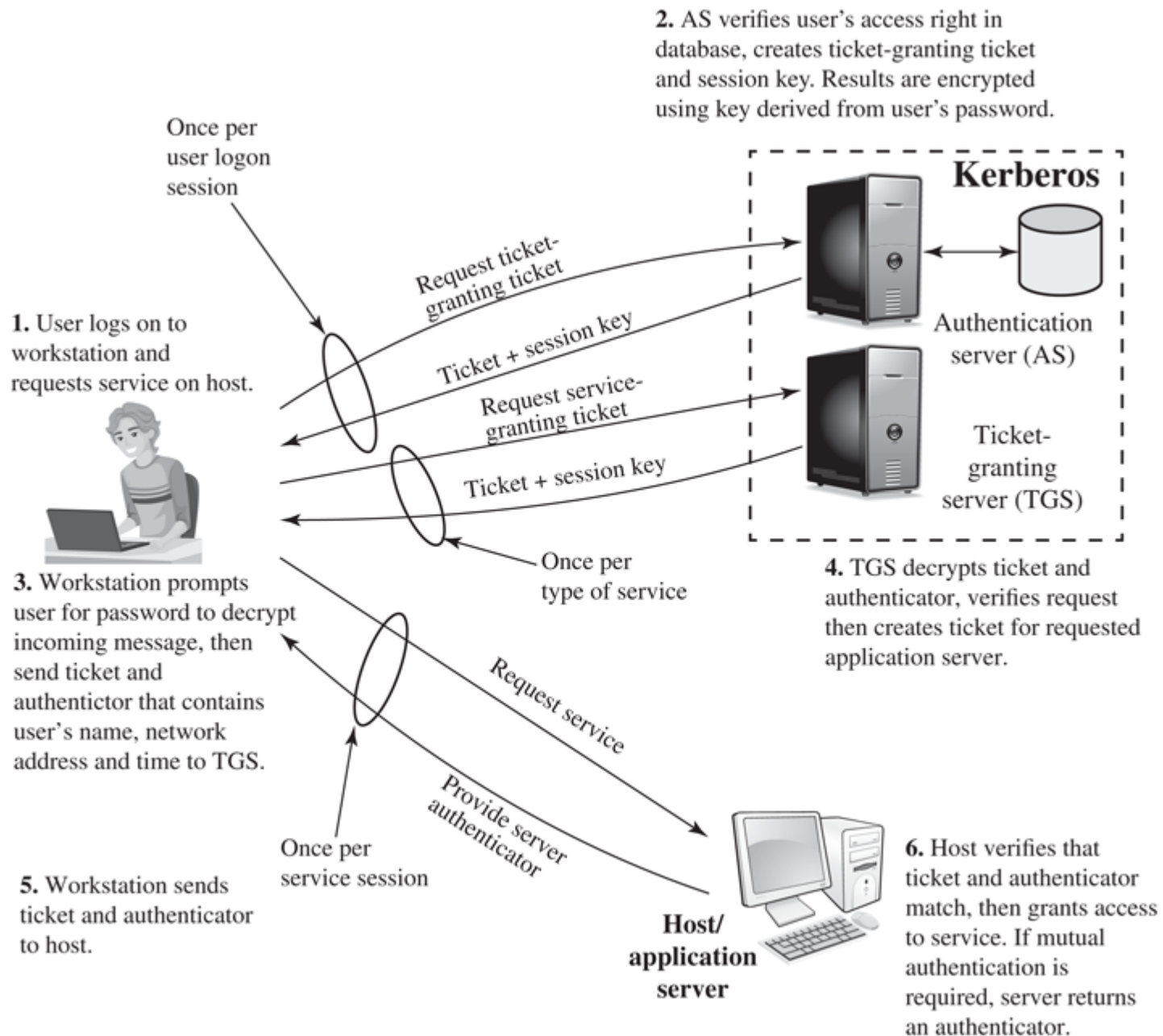
Figure 23.1 Overview of Kerberos
