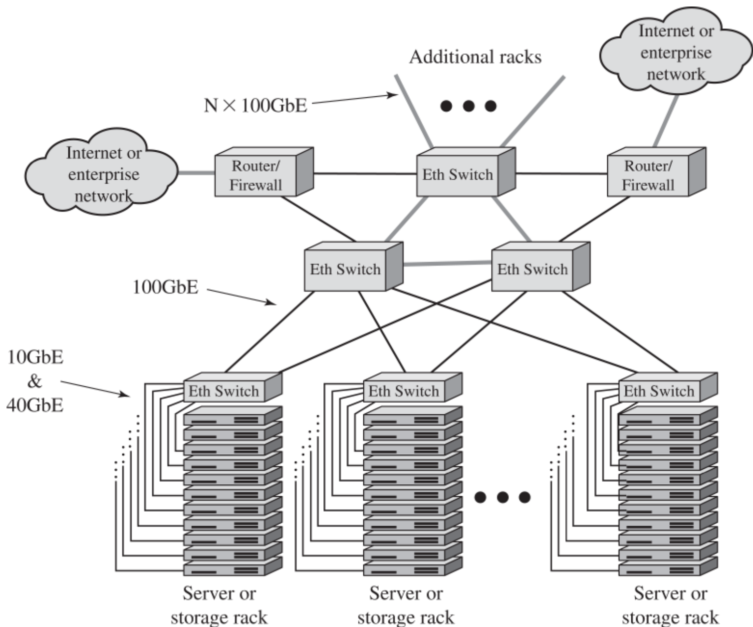
Figure 5.11 Key Data Center Elements
