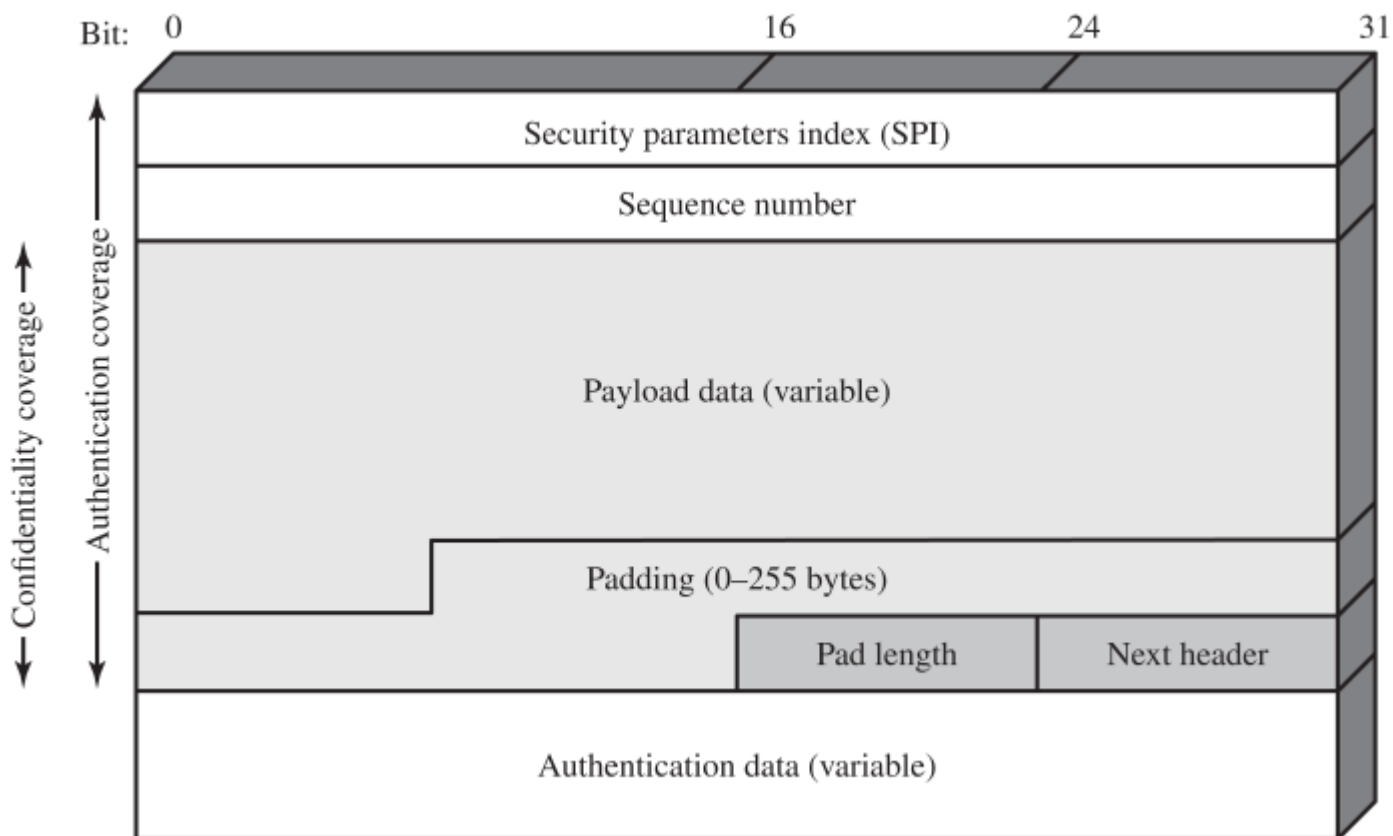
Figure 22.8 IPsec ESP Format
