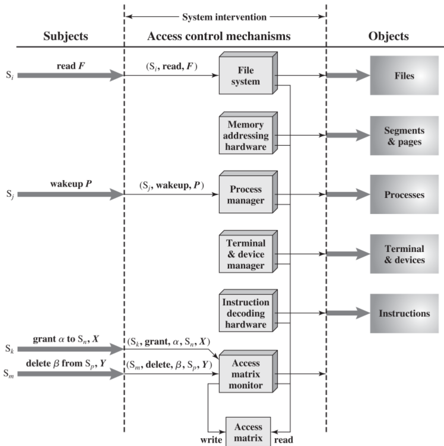
Figure 4.4 An Organization of the Access Control Function
