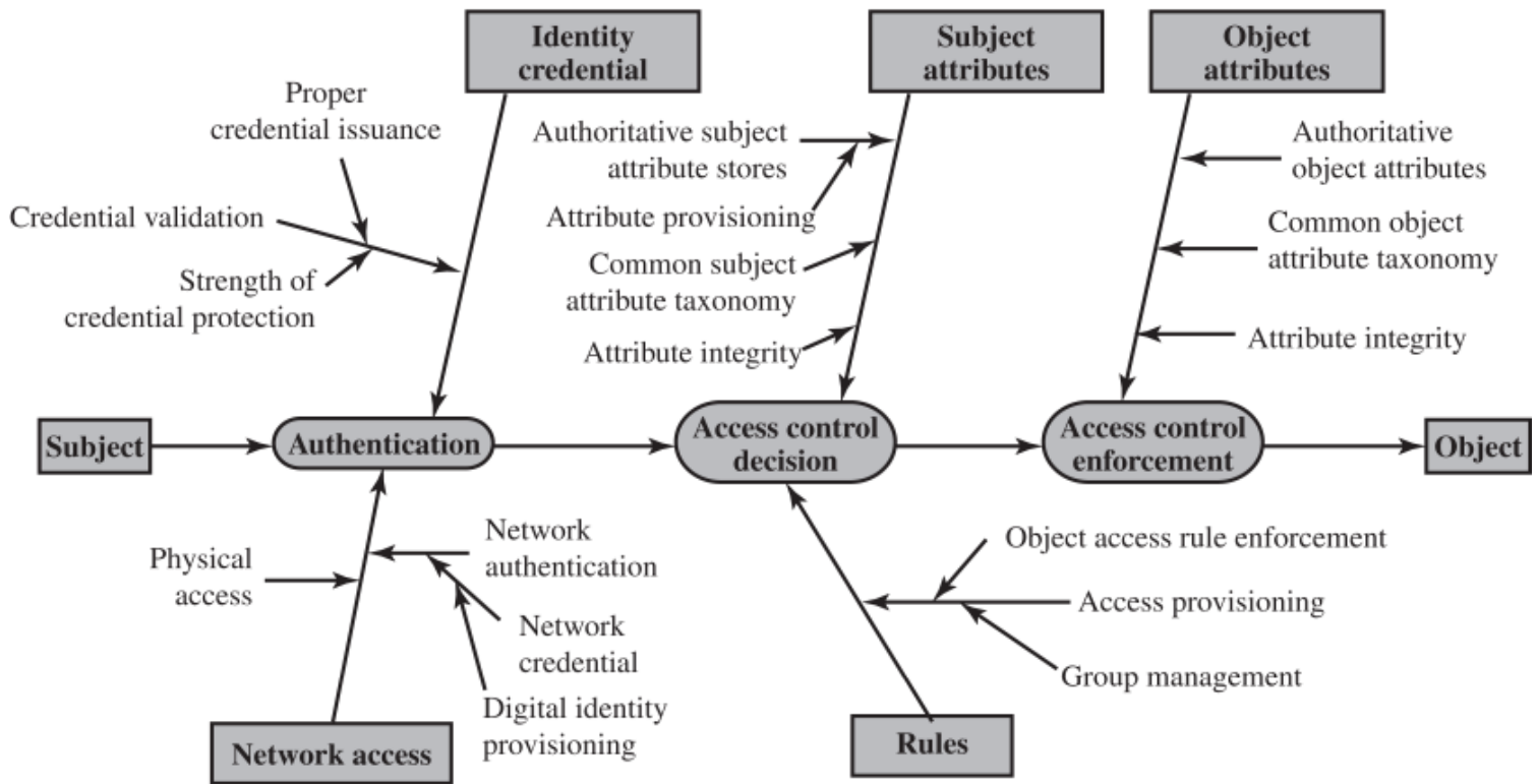
(b) ABAC Trust Chain
