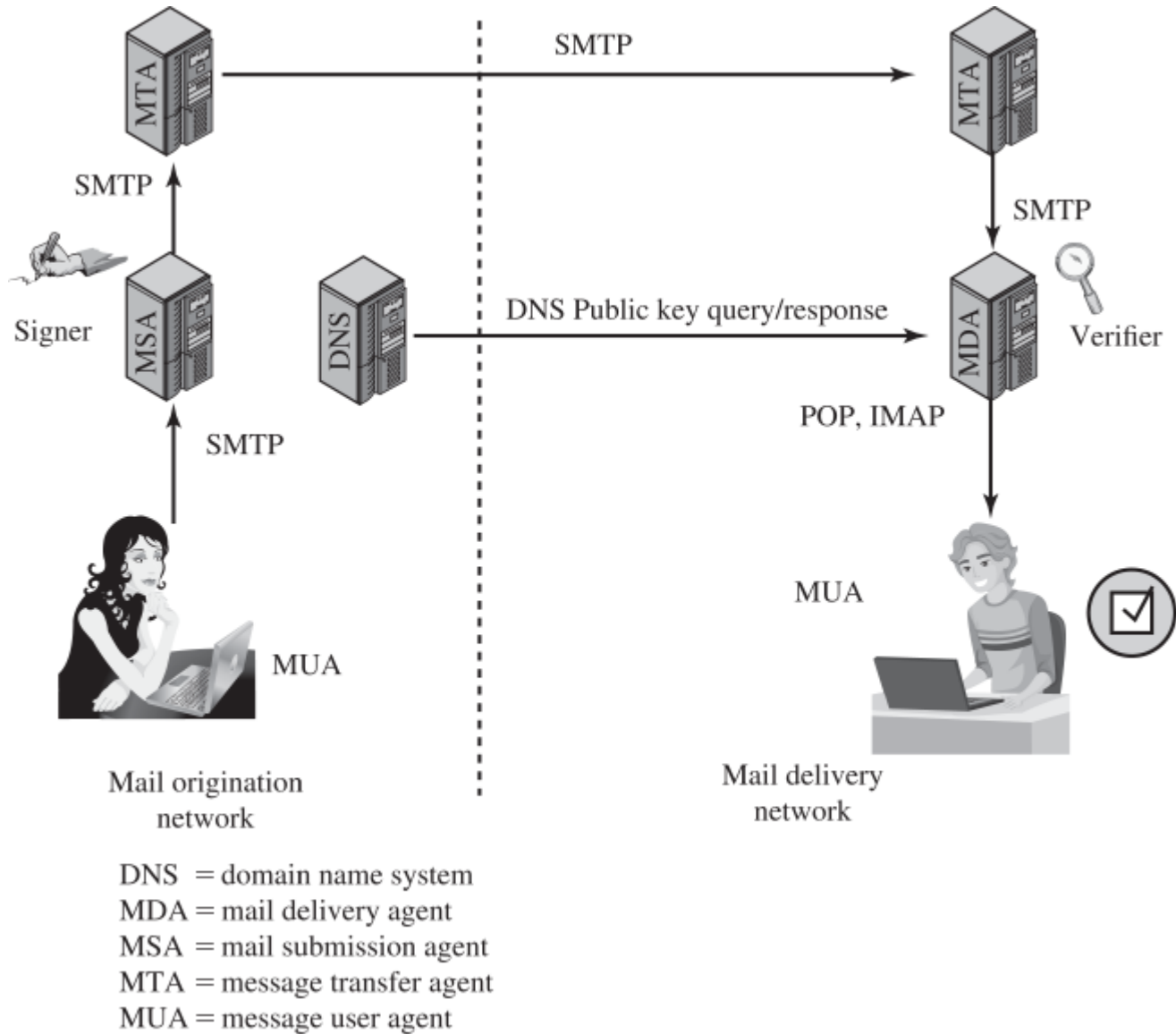
Figure 22.3 Simple Example of DKIM Deployment
