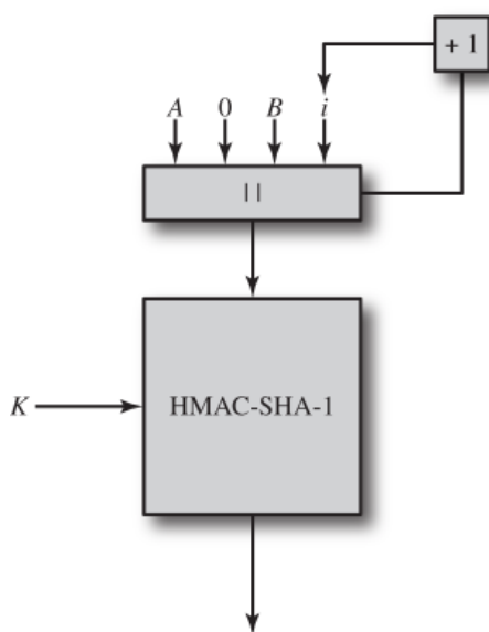
Figure 24.12 IEEE 802.11i Pseudorandom Function
