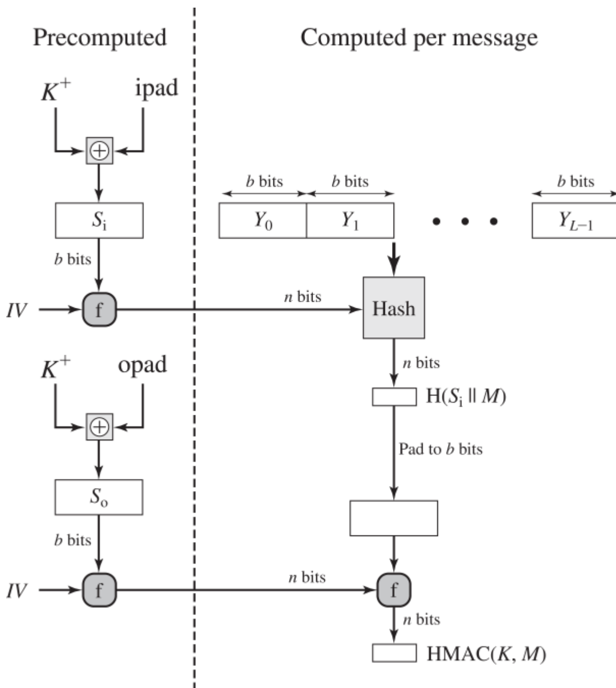
Figure 21.11 Alternative Implementation of HMAC
