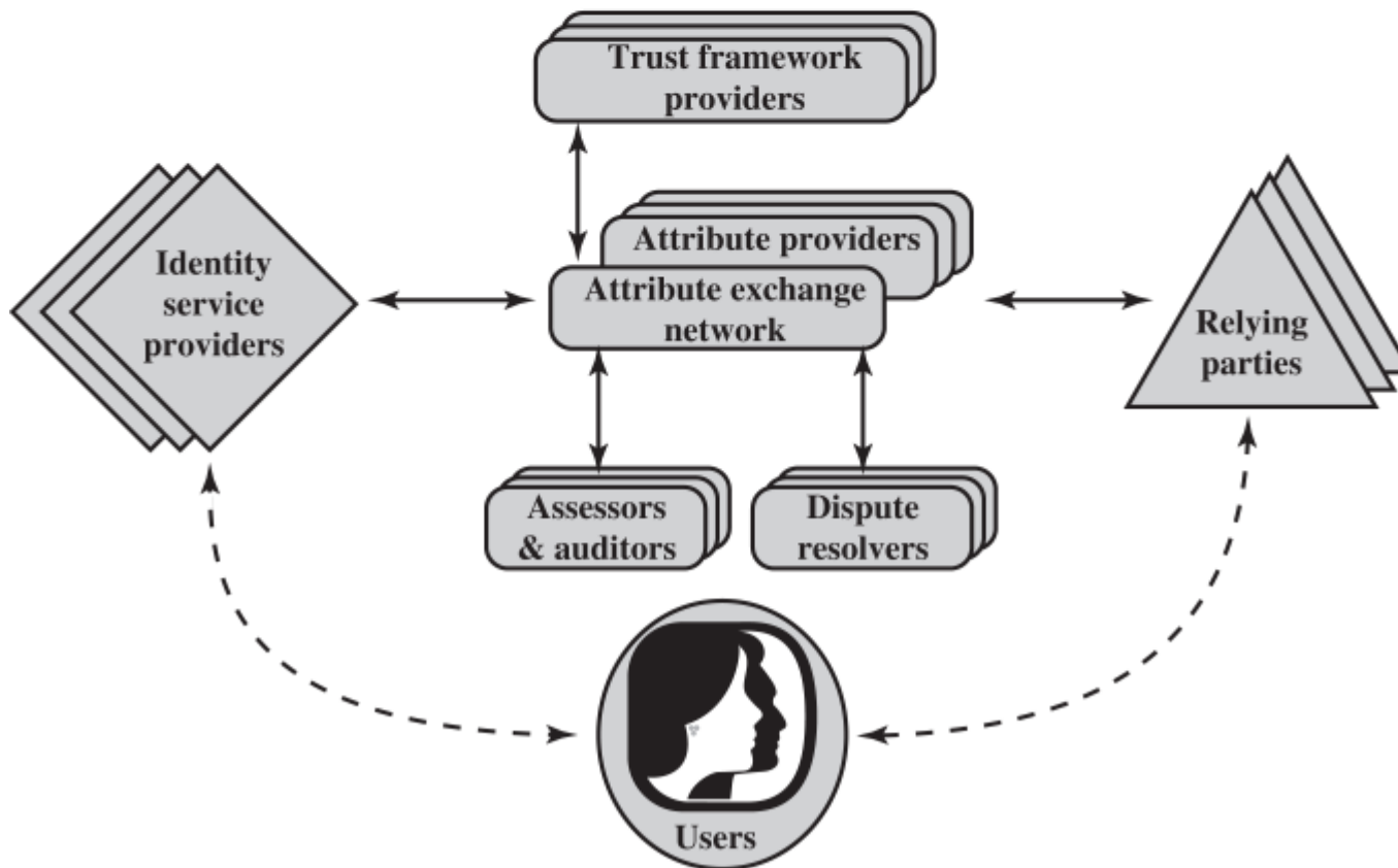
(b) Identity attribute exchange elements
