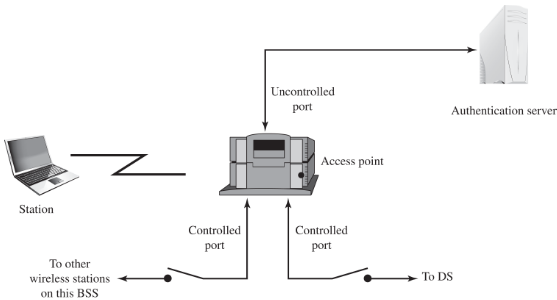
Figure 24.9 802.1X Access Control
