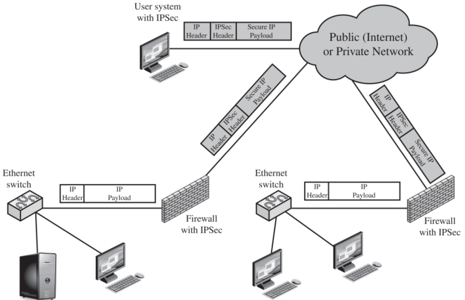
Figure 9.3 A VPN Security Scenario
