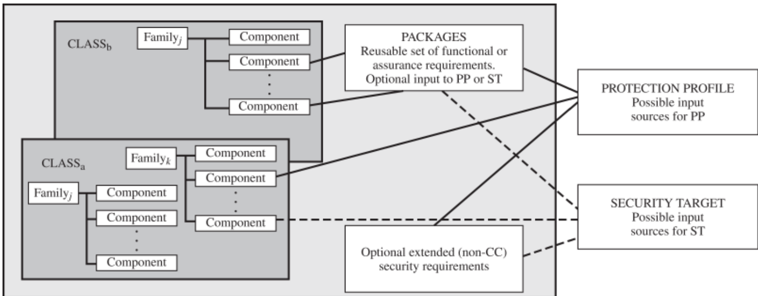
Figure 27.13 Organization and Construction of Common Criteria Requirements
