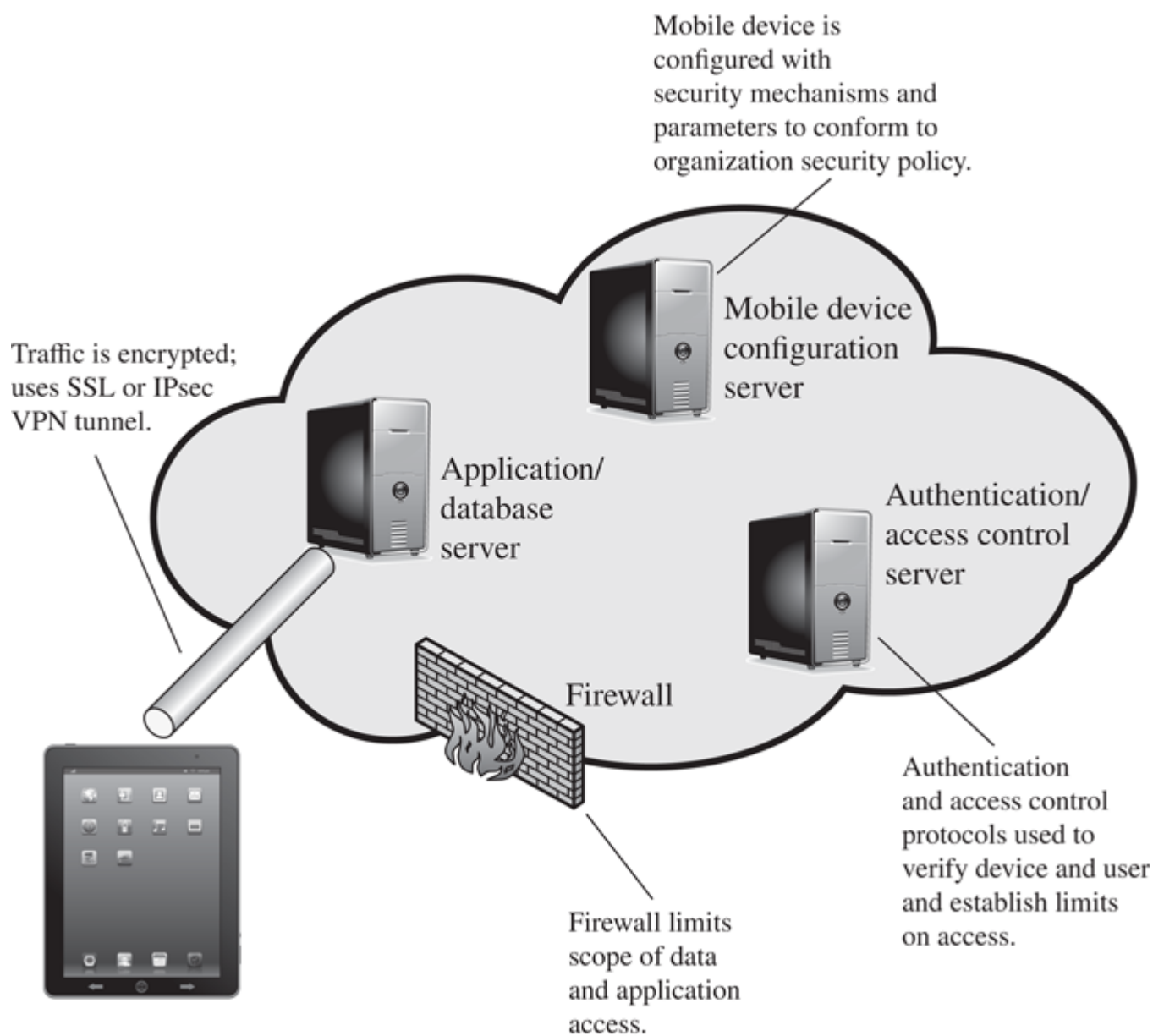
Figure 24.2 Mobile Device Security Elements
