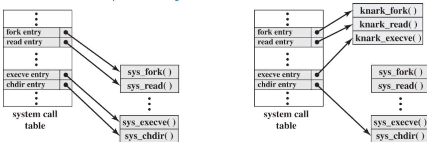
(a) Normal kernel memory layout
