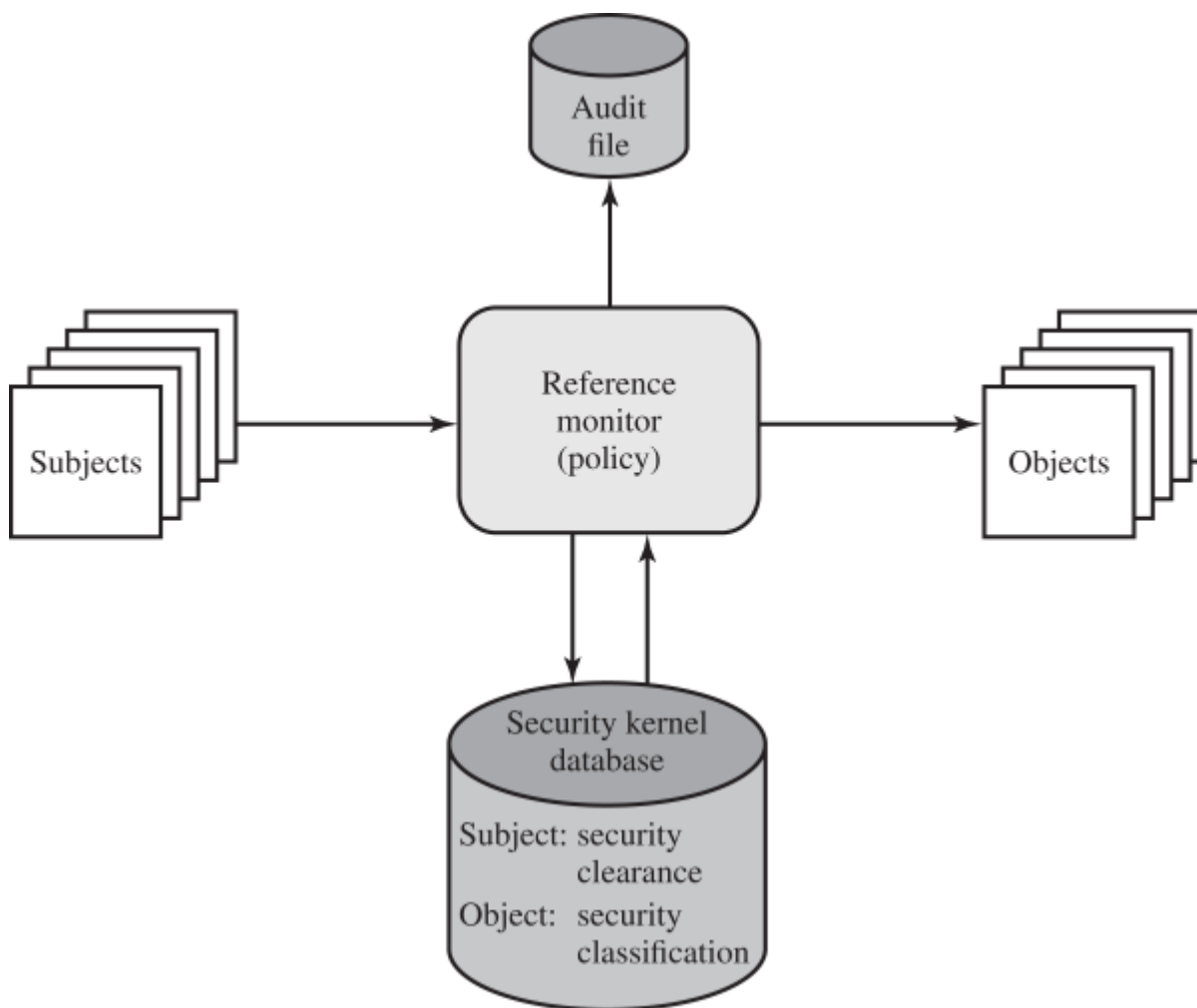
Figure 27.7 Reference Monitor Concept
