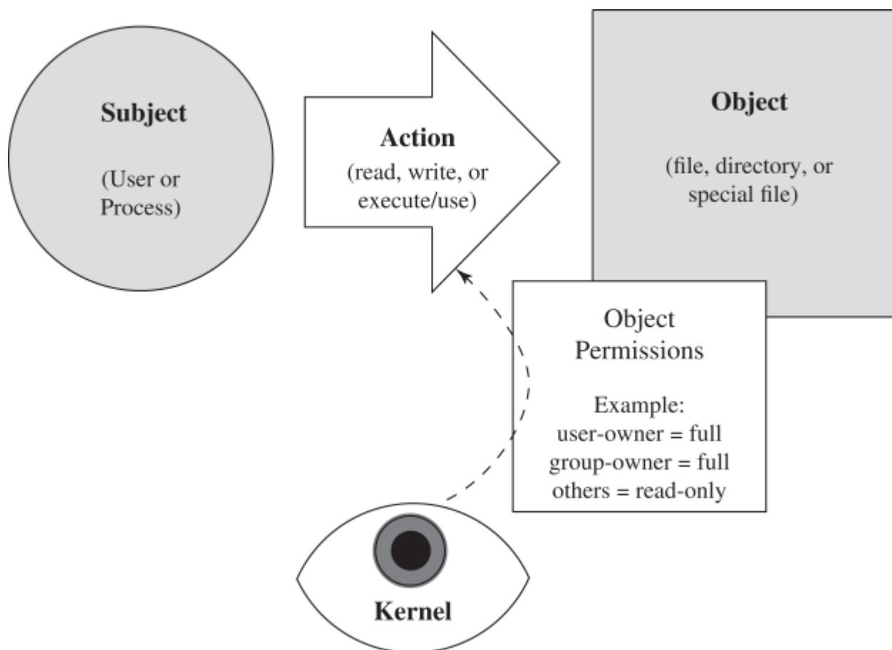
Figure 25.1 Linux Security Transactions
