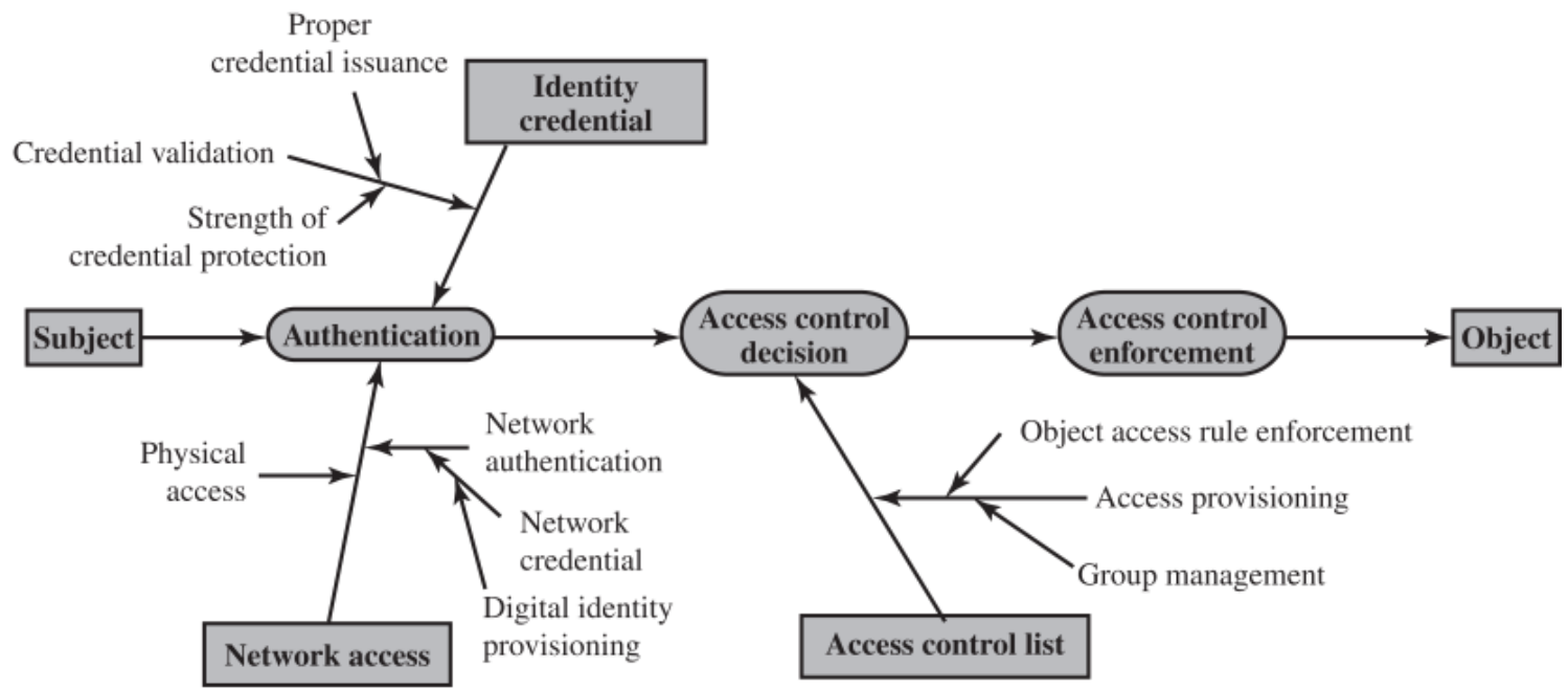
(a) ACL Trust Chain
