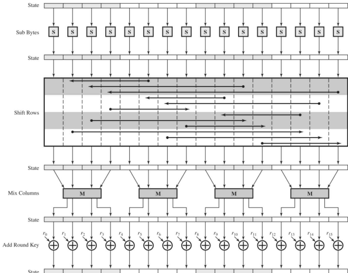
Figure 20.4 AES Encryption Round
