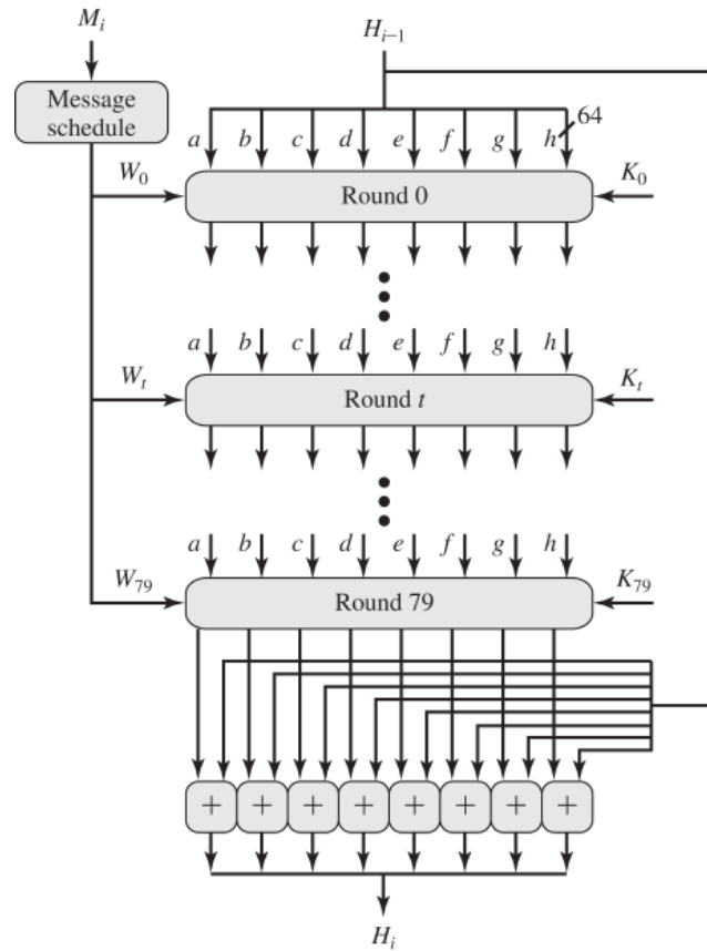
Figure 21.3 SHA-512 Processing of a Single 1024-Bit Block
