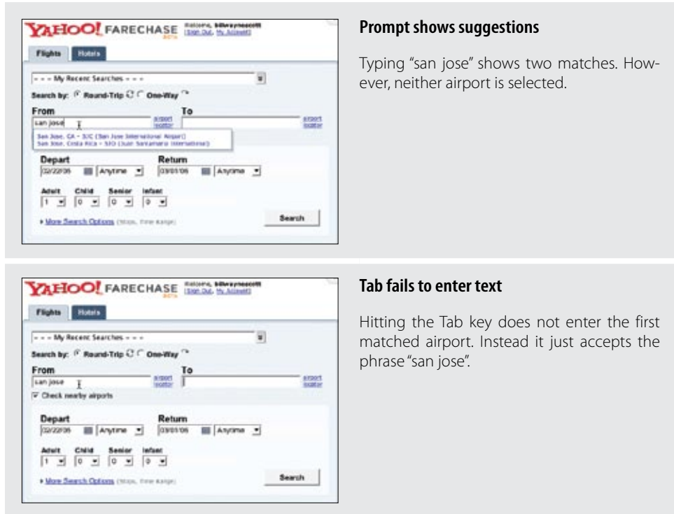
Figure 13-2. Farechase’s implementation of Auto Complete makes selection tedious
