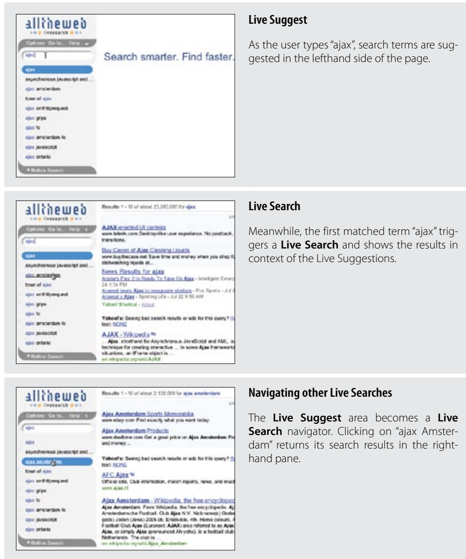
Figure 13-12. AllTheWeb.com LiveSearch was an experimental combination of Live Suggest and Live Search
