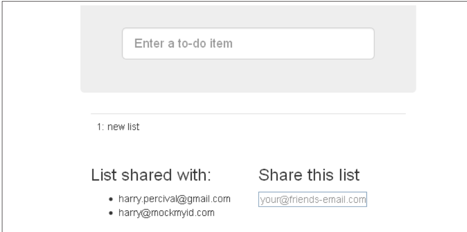
Figure 21-1. Sharing lists
