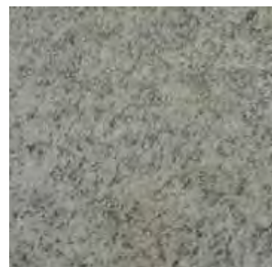
Figure 16.2. Some granite.
