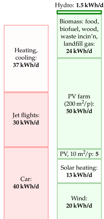
Figure 8.3. Hydroelectricity.
