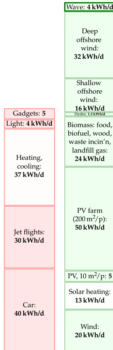
Figure 12.2. Wave.
