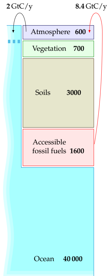
Figure 31.3. The arrows show two extra carbon flows produced by burning fossil fuels. There is an imbalance between the 8.4 GtC/y emissions into the atmosphere from burning fossil fuels and the 2 GtC/y take-up of CO 2 by the oceans. This cartoon omits the less-well quantified flows between atmosphere, soil, vegetation, and so forth.
