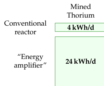
Figure 24.8. Thorium options.
