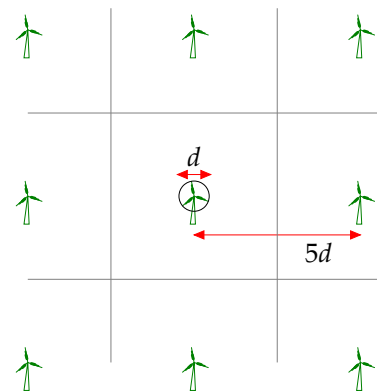
Figure B.4. Wind farm layout.
