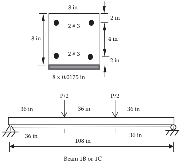
FIGURE 5.24 Example 5.16 showing the beam section and profile.
