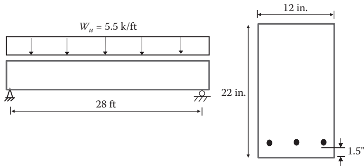
FIGURE 2.16 Beam profile and cross section for Example 2.3.
