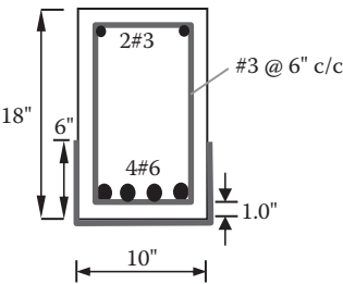
FIGURE 5.4 Example 5.3 showing the cross-section details.
