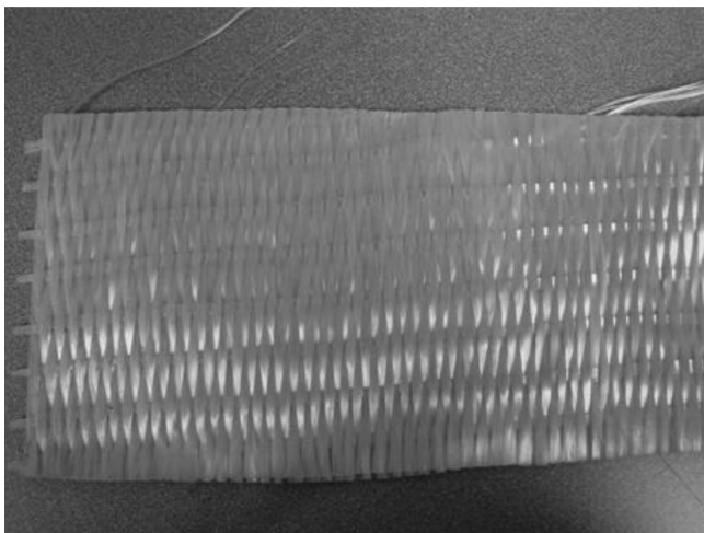
FIGURE 3.2 Unidirectional E-glass fiber sheet used in concrete strengthening.
