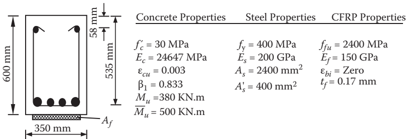
FIGURE 5.9 Design of a doubly reinforced beam example by Chaallal, Nollet, and Perraton (1998).
