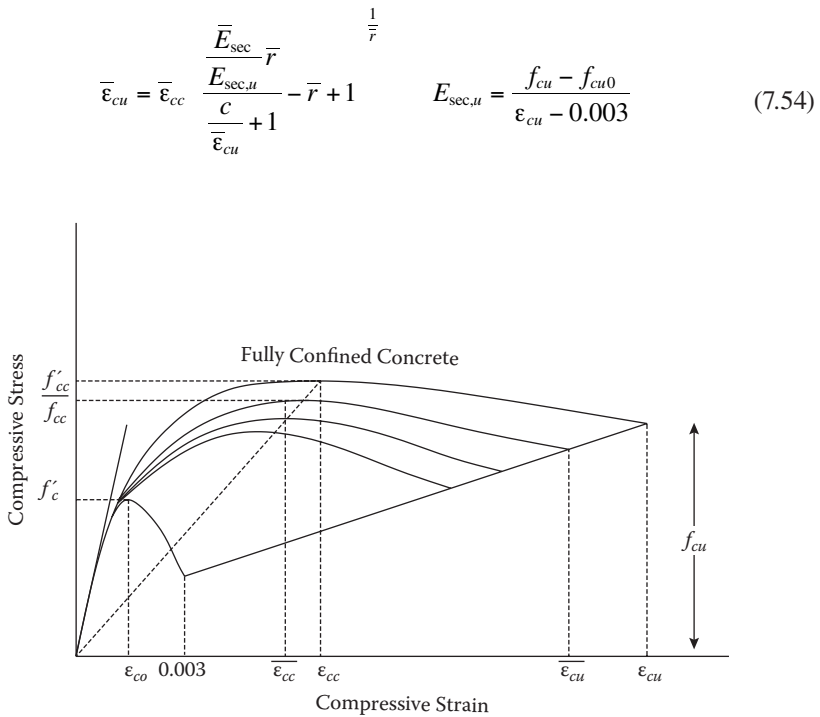
FIGURE 7.9 Eccentricity-based confined Mander model.
