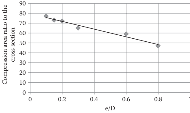
FIGURE 7.7 The relationship between the normalized compression zone size and eccentricity in circular columns. (Courtesy of Abd El Fattah [2012].)
