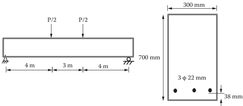
FIGURE 2.21 Beam profile and cross section for Example 2.7.
