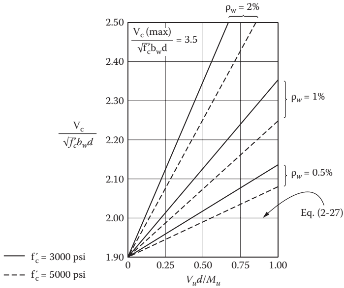
FIGURE 2.14 Concrete shear strength for shear and flexure only. (Courtesy of Portland Cement Association [2013].)
