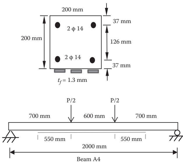
FIGURE 5.22 Example 5.14 showing the beam section and profile.
