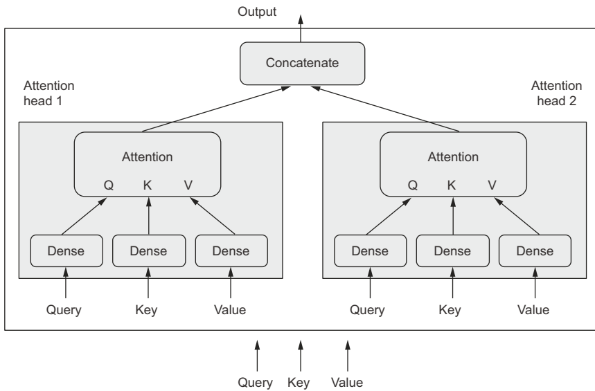
Figure 11.8 The MultiHeadAttention layer
