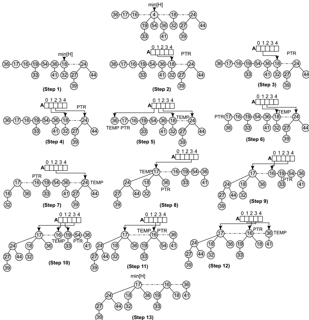
Figure 12.34 Fibonacci heap
