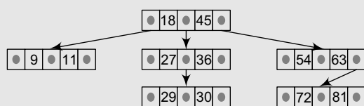
(3-way search tree for Q.13)
