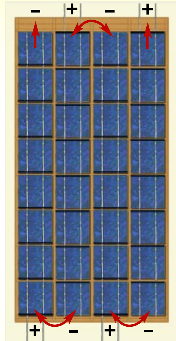
Strings of solar cells laid out on the template
