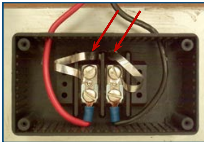
Bus ribbon comes through holes in the panel into the junction box at the back.
