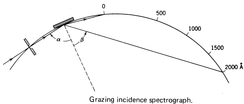
Optical layout of basic spectrograph.
