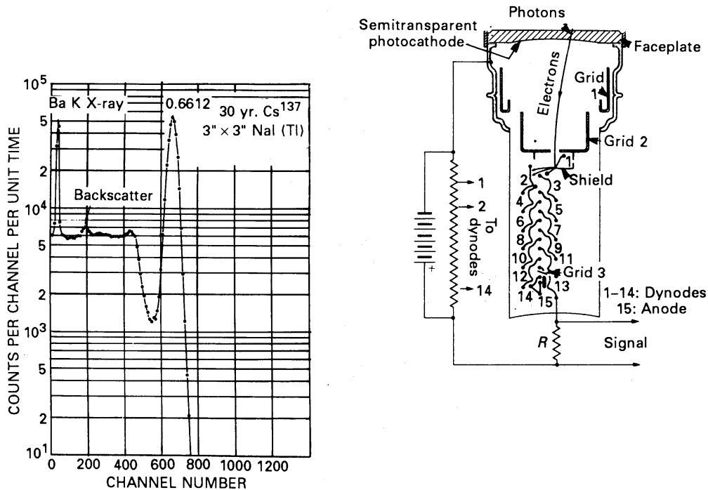
A typical pulse-height spectrum obtained with a NaI(Tl) spectrometer, illustrating the energy response of inorganic scintillators. The scale of the abscissa is 1 keV per channel.
