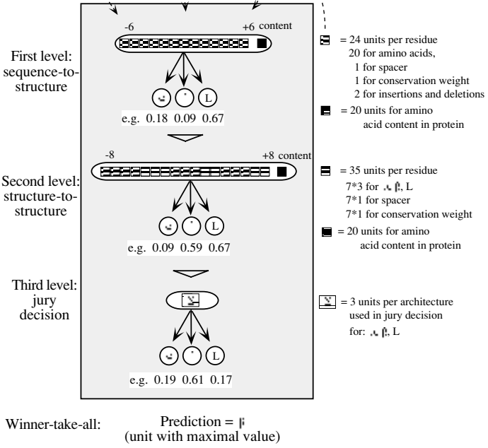
Figure 6.2: The PHD Architecture for Secondary Structure Prediction Developed by Rost and Sander. The input is based not on a conventional orthogonal encoding of the query sequence, but on a profile made from amino acid occurrences in columns of a multiple alignment of sequences with high similarity to the query sequence.
