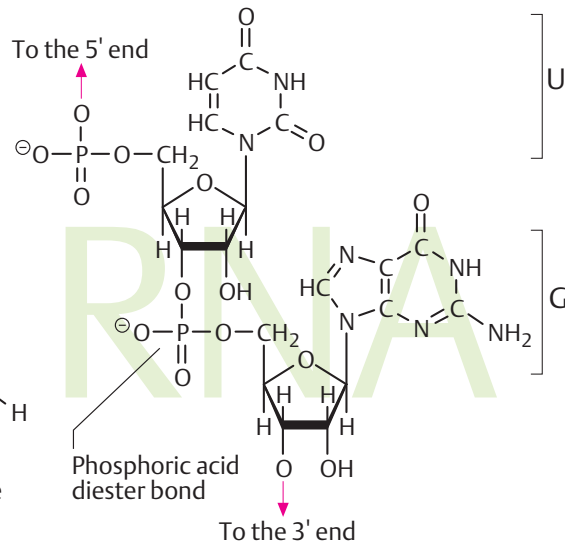
2. RNA (section)
