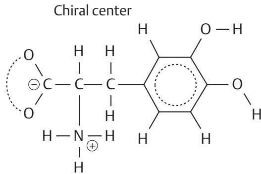
1. Formula illustration
