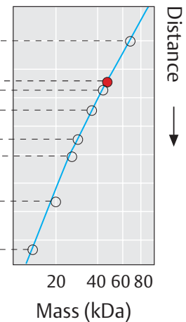
4. Analysis
