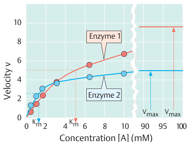
1. Hyperbolic plot
