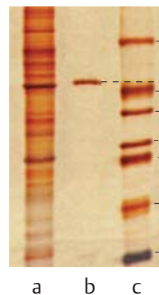
3. Stained gel
