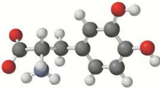
2. Ball- and-stick model
