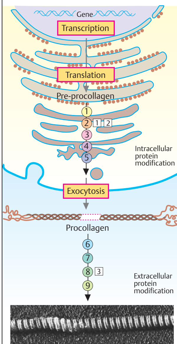
Type I tropocollagen ~285 kDa
