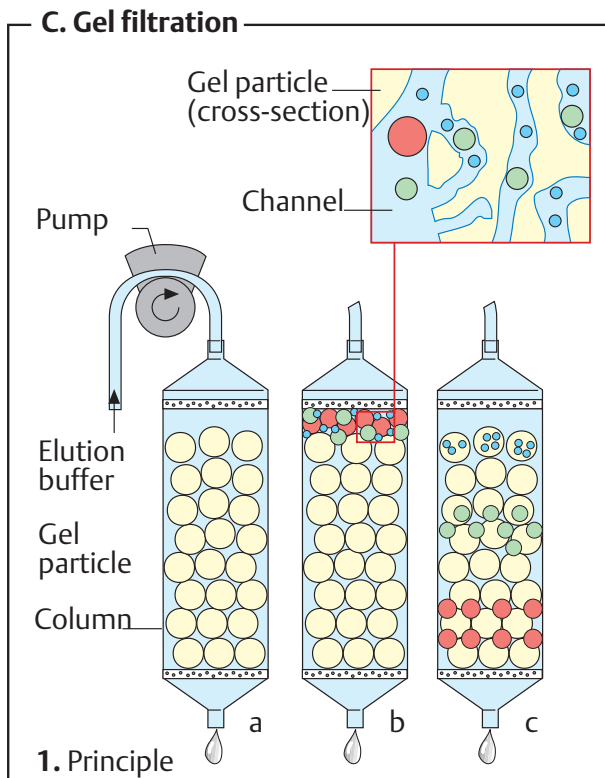
1. Principle
