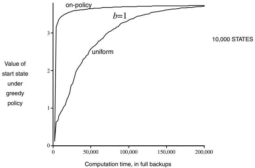
Figure 9.14 Relative efficiency of backups distributed uniformly across the state space versus focused on simulated on-policy trajectories. Results are for randomly generated tasks of two sizes and various branching factors, b .
