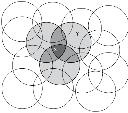
Figure 8.2 Coarse coding. Generalization from state X to state Y depends on the number of their features whose receptive fields (in this case, circles) overlap. These states have one feature in common, so there will be slight generalization between them.
