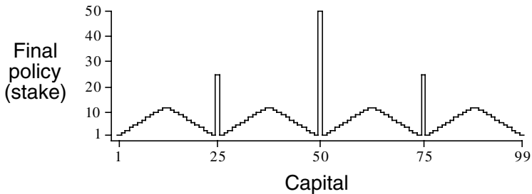
Figure 4.6 The solution to the gambler's problem for p = 0.4 . The upper graph shows the value functions found by successive sweeps of value iteration. The lower graph shows the final policy.
