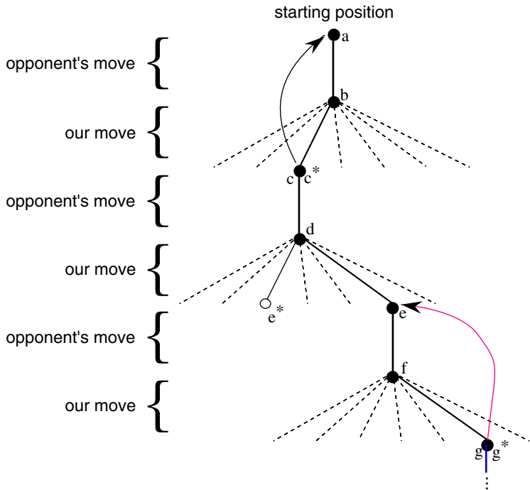
Figure 1.1 A sequence of tic-tac-toe moves. The solid lines represent the moves taken during a game; the dashed lines represent moves that we (our reinforcement learning player) considered but did not make. Our second move was an exploratory move, meaning that it was taken even though another sibling move, the one leading to e^* , was ranked higher. Exploratory moves do not result in any learning, but each of our other moves does, causing backups as suggested by the curved arrows and detailed in the text.
