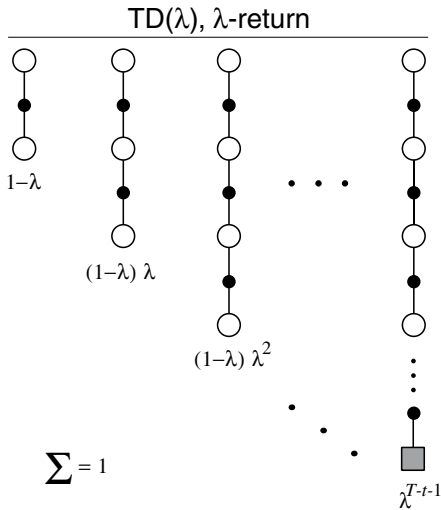
Figure 7.3 The backup digram for TD( \lambda ). If \lambda = 0 , then the overall backup reduces to its first component, the one-step TD backup, whereas if \lambda = 1 , then the overall backup reduces to its last component, the Monte Carlo backup.
