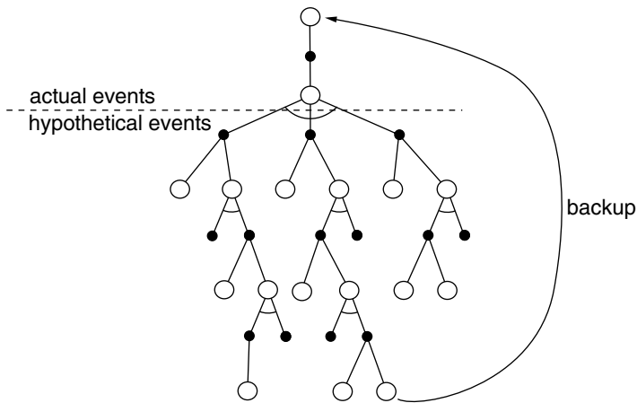
Figure 11.3 The backup diagram for Samuel's checkers player.
