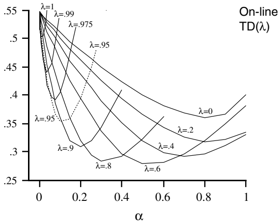
Figure 7.9 Performance of on-line TD( \lambda ) on the 19-state random walk task.
