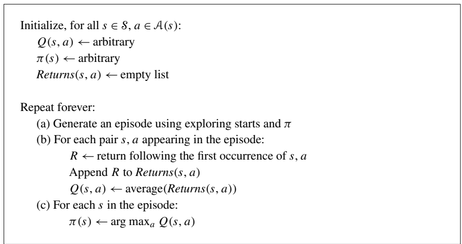
Figure 5.4 Monte Carlo ES: A Monte Carlo control algorithm assuming exploring starts.
