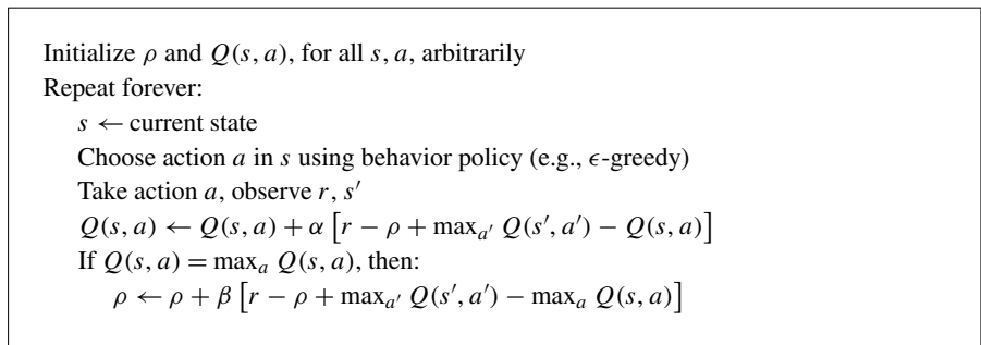
Figure 6.16 R-learning: An off-policy TD control algorithm for undiscounted, continuing tasks. The scalars \alpha and \beta are step-size parameters.
