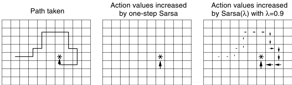
Figure 7.12 Gridworld example of the speedup of policy learning due to the use of eligibility traces.
