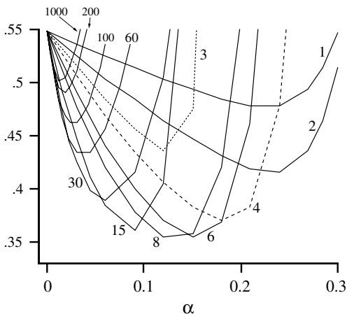
Figure 7.2 Performance of n -step TD methods as a function of \alpha , for various values of n , on a 19-state random walk task. The performance measure shown is the root mean-squared (RMS) error between the true values of states and the values found by the learning methods, averaged over the 19 states, over the first 10 trials, and over 100 different sequences of walks.
