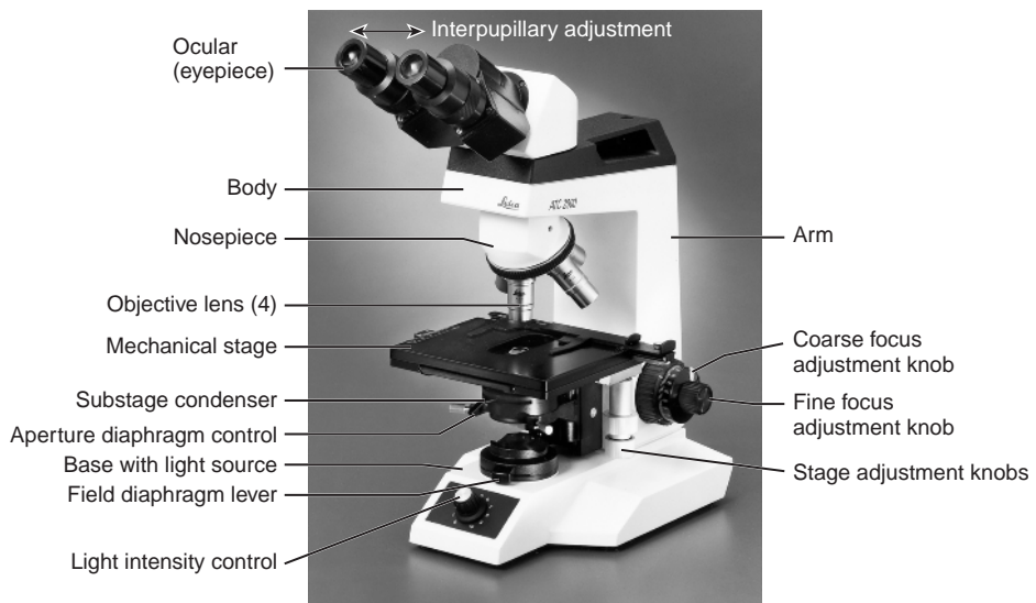
Fig. 3-4. Parts of a compound light microscope.
