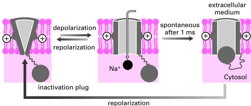
Figure 15.4. The voltage-gated sodium channel.
