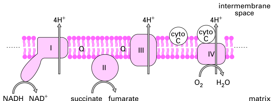
Figure 12.7. The electron transport chain comprises four large multimolecular complexes in the inner mitochondrial membrane, three of which are hydrogen ion carriers.
