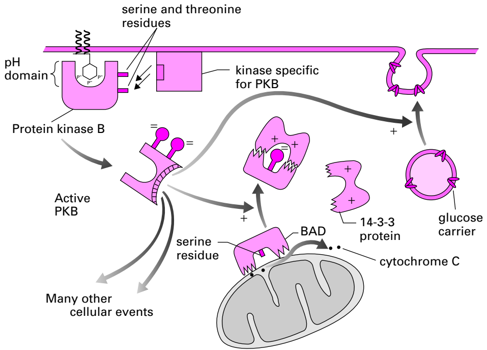
Figure 16.11. \text{PIP}_3 recruits protein kinase B (PKB) to the plasma membrane, where it is activated. Active PKB has many effects including exocytosis of vesicles containing glucose carriers and inactivation of BAD.
