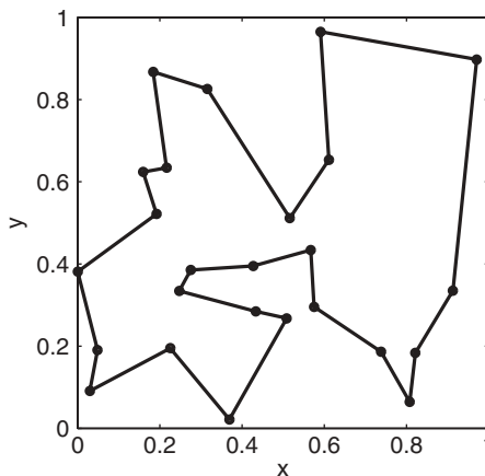
Figure 6.4 GA solution to 25 city traveling salesperson problem.
