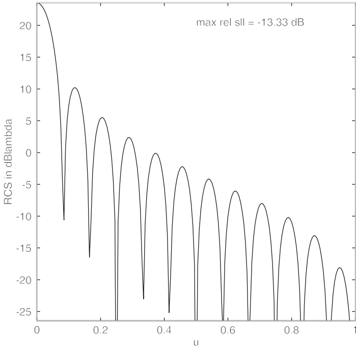
Figure 6.16 Radar cross section of a 6\lambda wide perfectly conducting strip.
