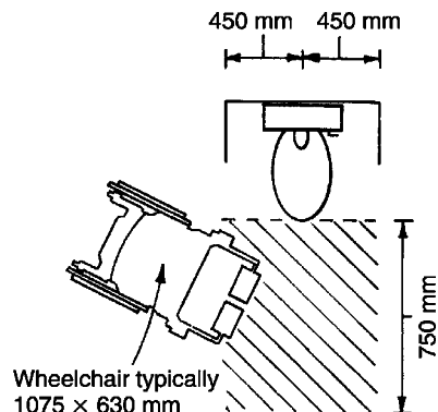
Oblique access to WC
