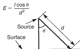
Illumination produced from a light source not perpendicular to the surface
