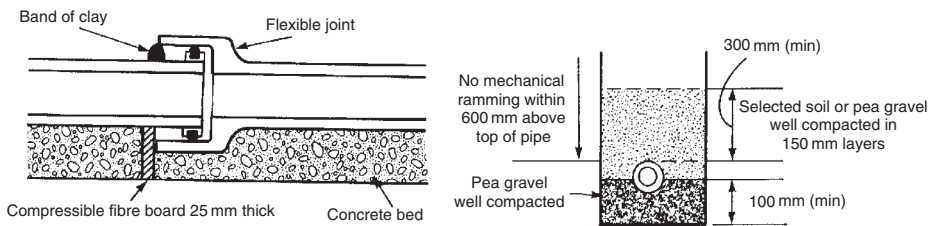
Class A bedding
