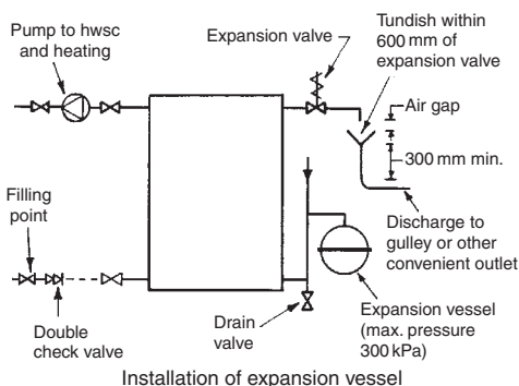
Installation of expansion vessel
