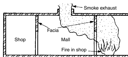
Smoke reservoir formed by facias above open fronted shops
