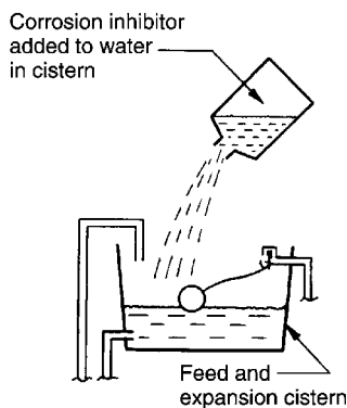
Dosing an open vent system
