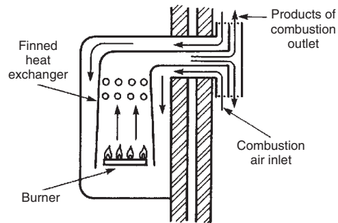
Balanced flue water heater
