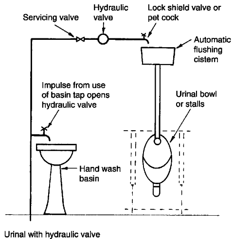
Urinal with hydraulic valve
