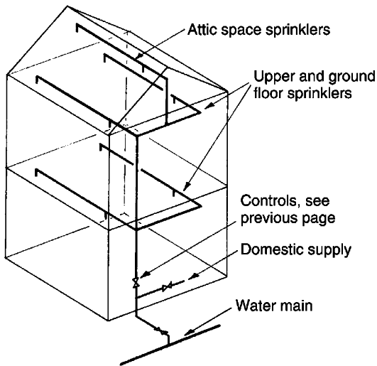
Typical domestic installation
