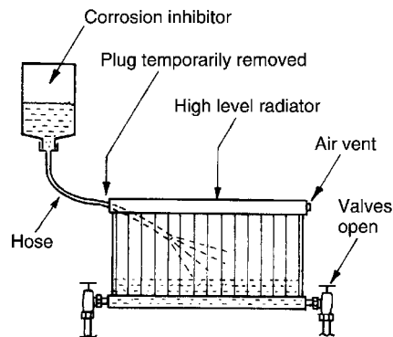
Dosing a sealed system
