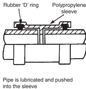
Flexible joint on clay pipe
