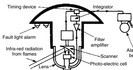
Infra-red detector for large areas
