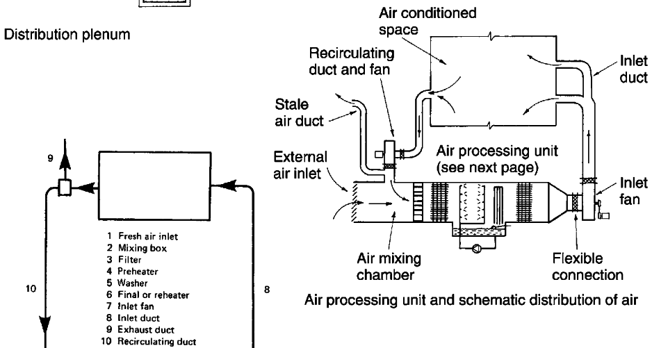
Diagrammatical layout of central plant only system
