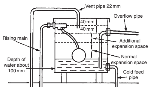
Expansion and feed cistern
