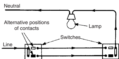
Two-way switching
