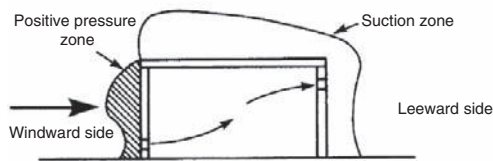
Wind pressure diagram for flat roofs
