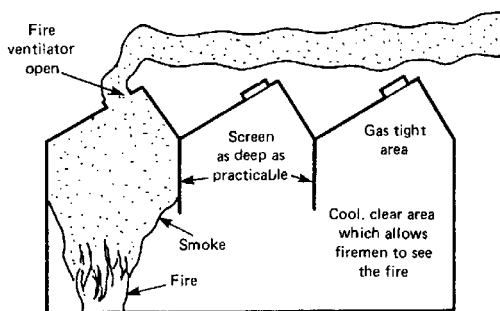
Fire in vented building showing restricted spread of smoke. The fire ventilator may also be used for normal ventilation.
