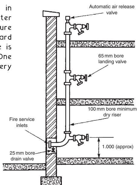
Typical arrangement of a dry riser
