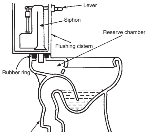
Single-trap type siphonic pan
