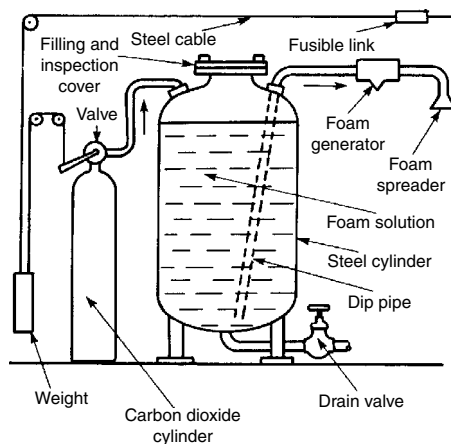
Pre-mixed foam installation
