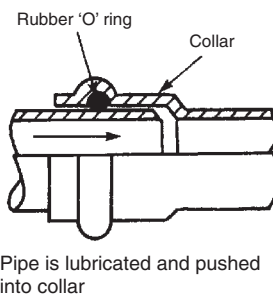
Flexible joint on uPVC pipe
