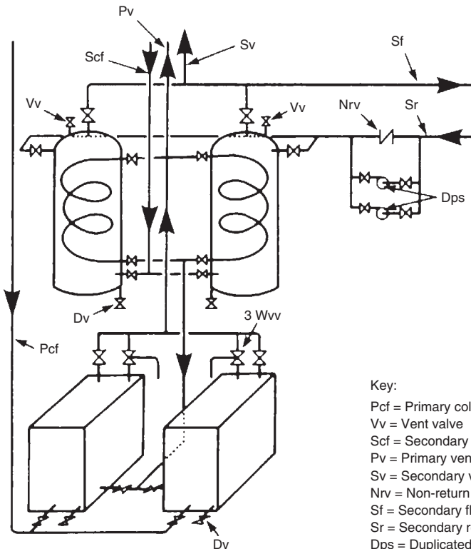
Duplicated plant
