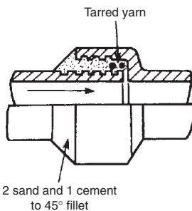
Cement mortar joint on clay pipe
