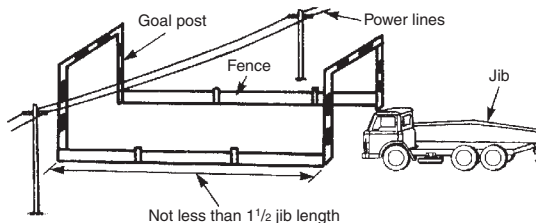
Goal posts (or barrier fences) give protection against contact with overhead power lines
