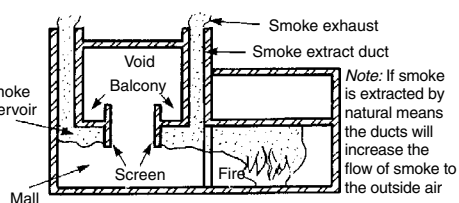
Use of smoke extract ducts through roof of mall
