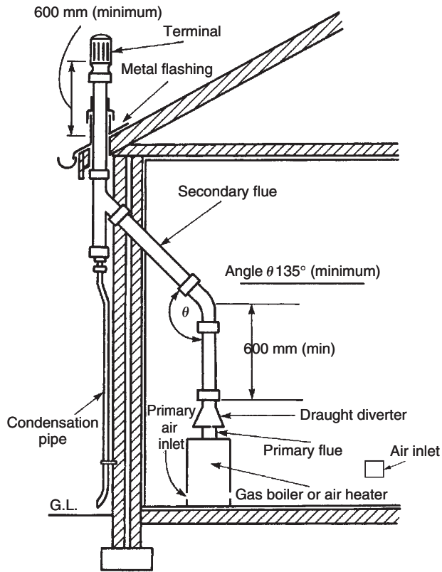
Installation of flue
