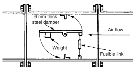
Swinging mechanical type
