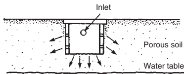
(a) Section
