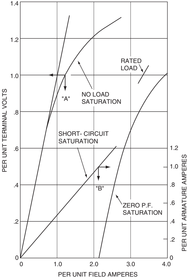
FIGURE 5.2 Saturation curves.
