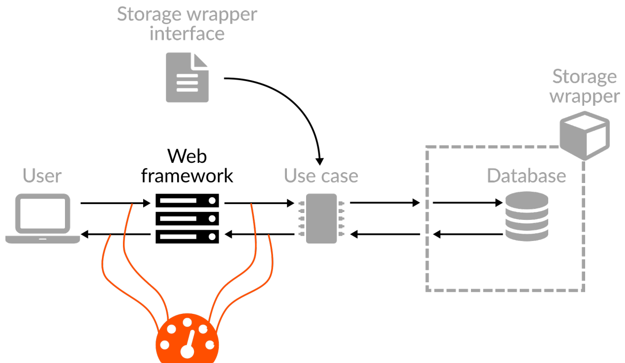
Testing the web layer in isolation
