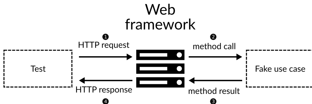
Detailed setup of the web layer testing
