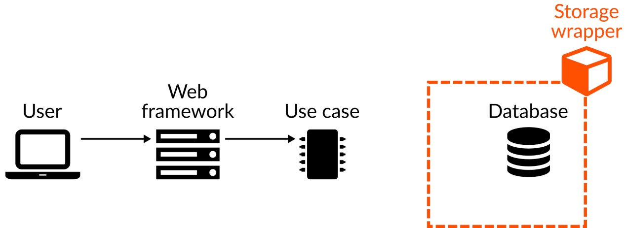
The storage interface
