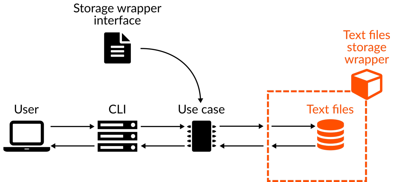
A database replaced by a more trivial file-based storage
